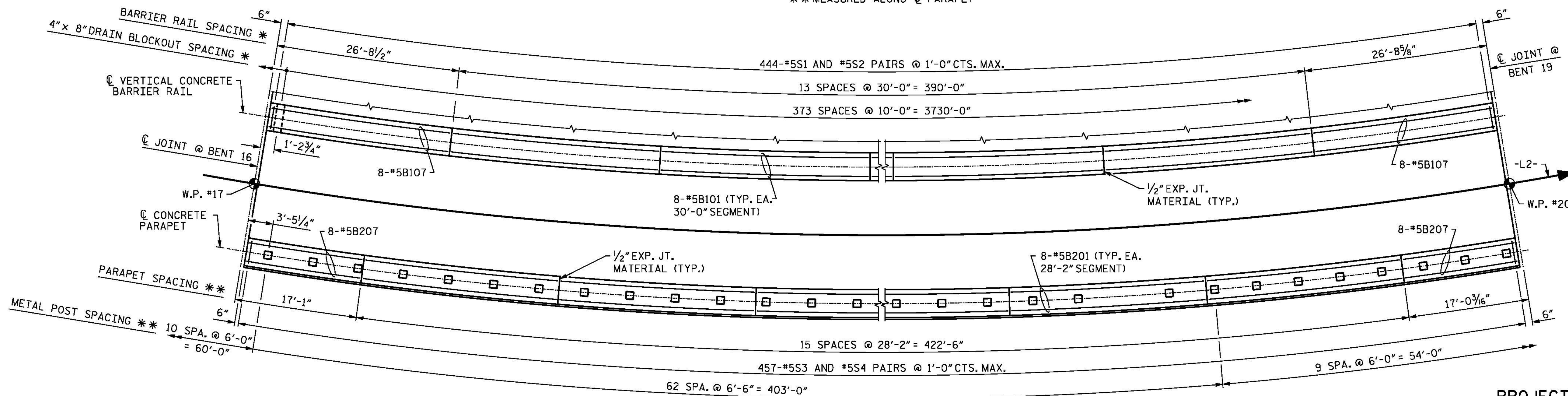
PLAN - UNIT 5 * MEASURED ALONG \bar{C} BARRIER ** MEASURED ALONG \bar{C} PARAPET
