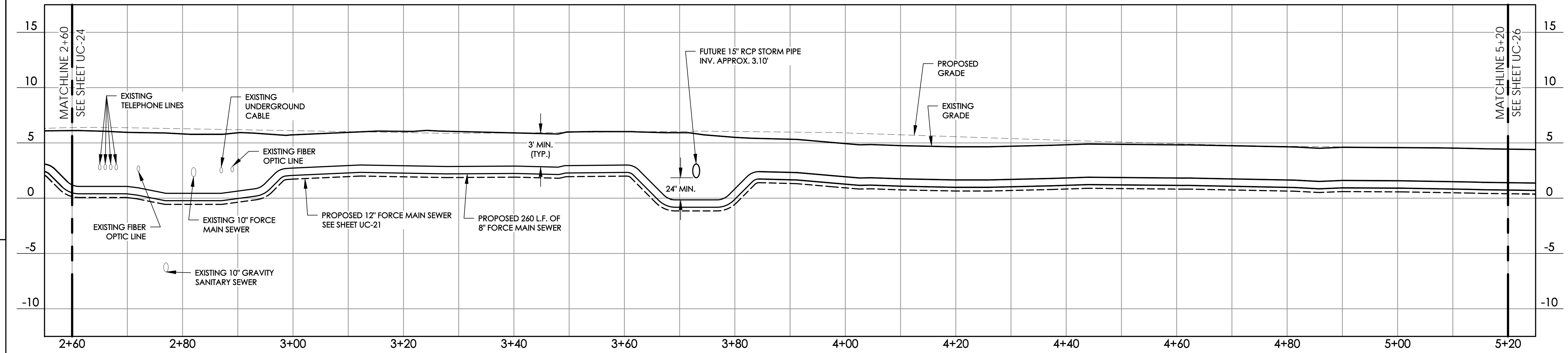
ISLAND 8" FORCE MAIN SEWER STA. 2+60 TO 5+20
