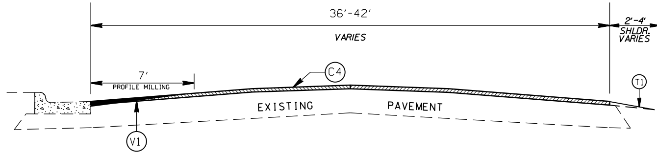
TYPICAL SECTION NO. 27
