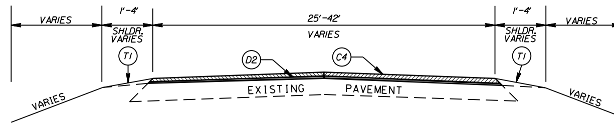
TYPICAL SECTION NO. 26
