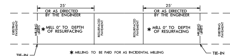
PAVEMENT TIE-IN DETAIL
