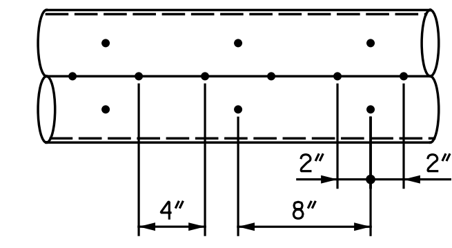
DETAIL 3
