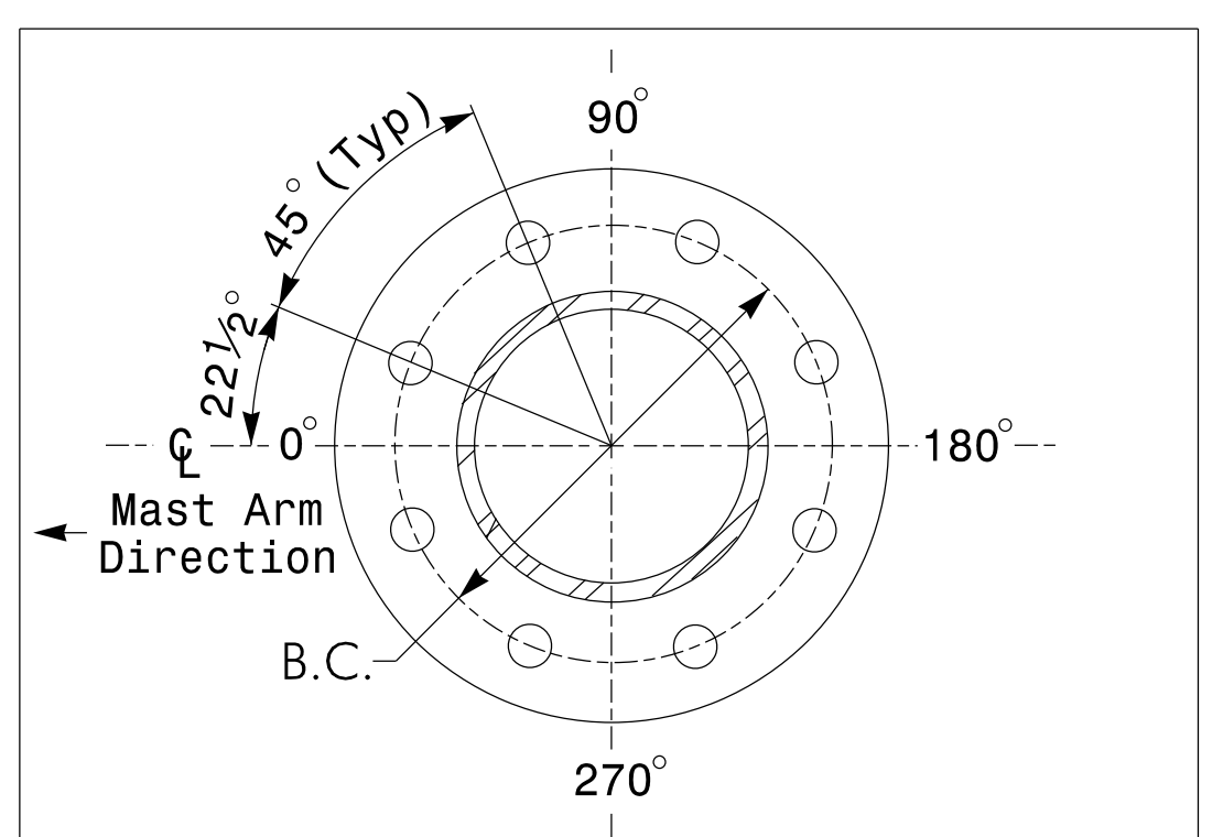
8 BOLT BASE PLATE DETAIL See Note 6
