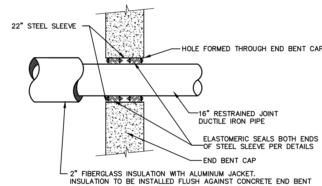
PIPE THROUGH END BENT CAP
