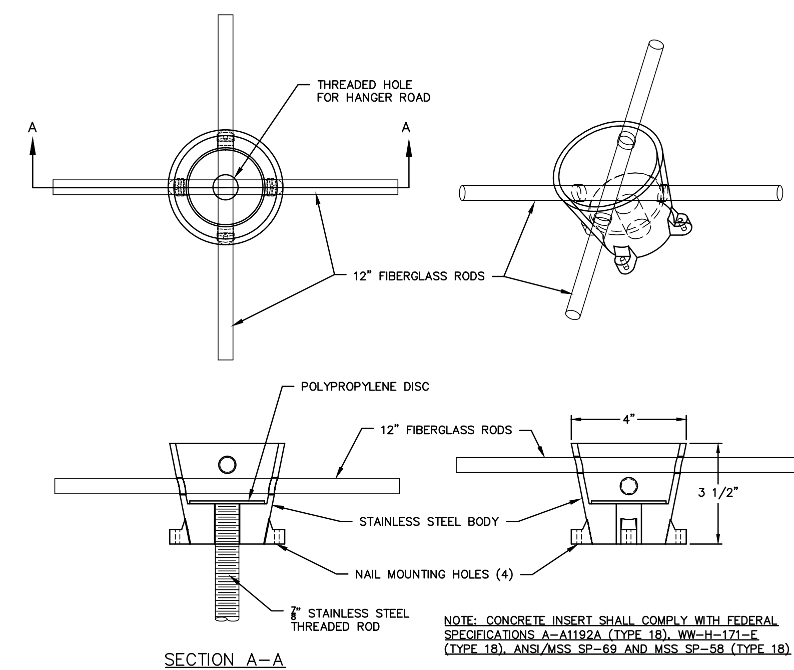
CONCRETE INSERT
