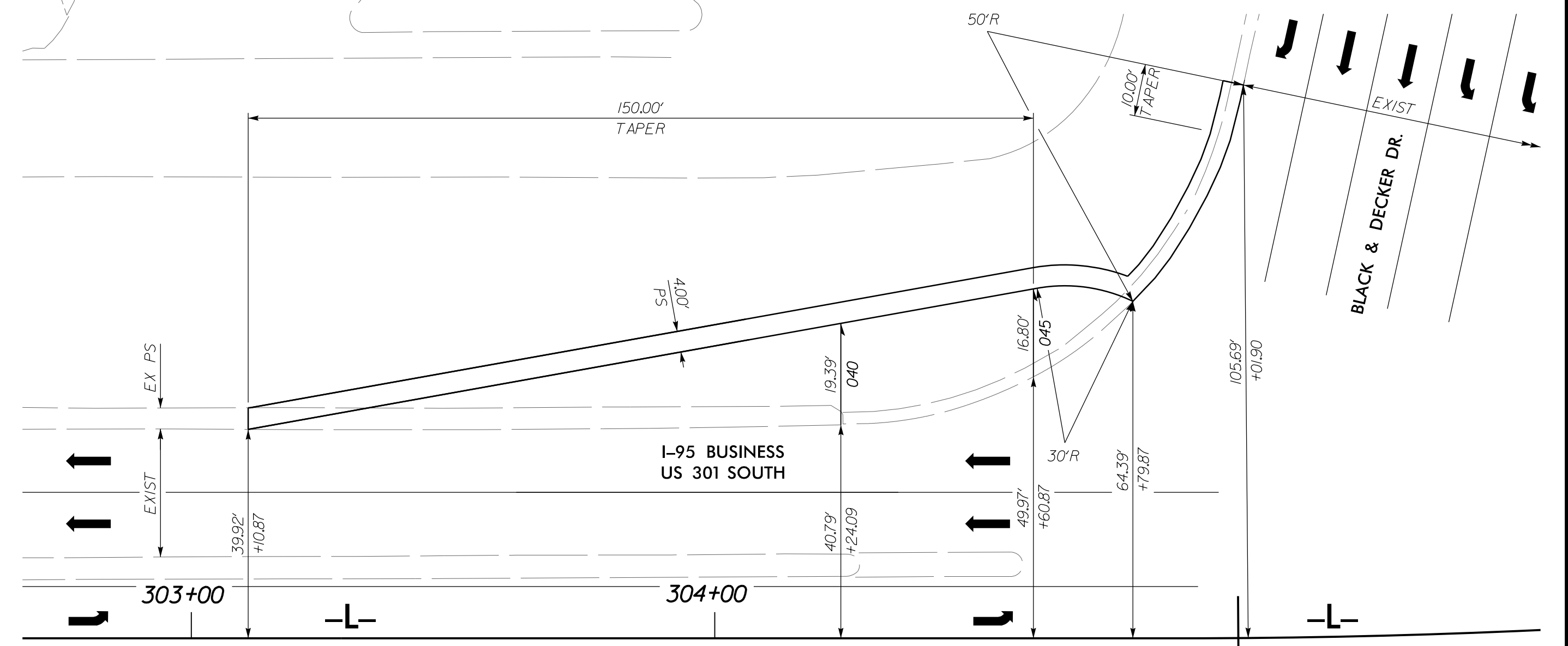
DETAIL #14 BLACK & DECKER DRIVE SEE PLAN SHEET 19
