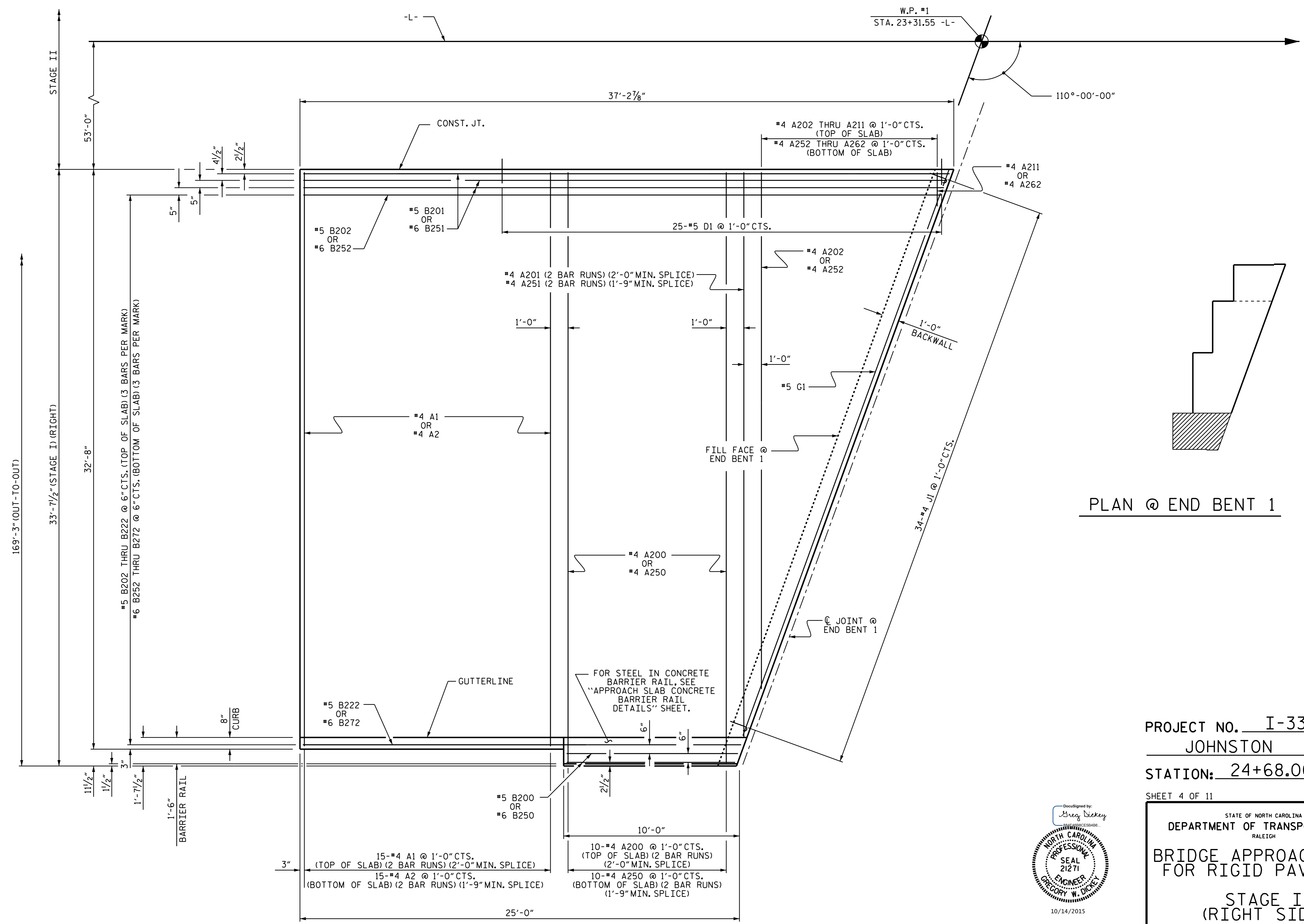
APPROACH SLAB AT END BENT 1 - STAGE I (RIGHT SIDE)
