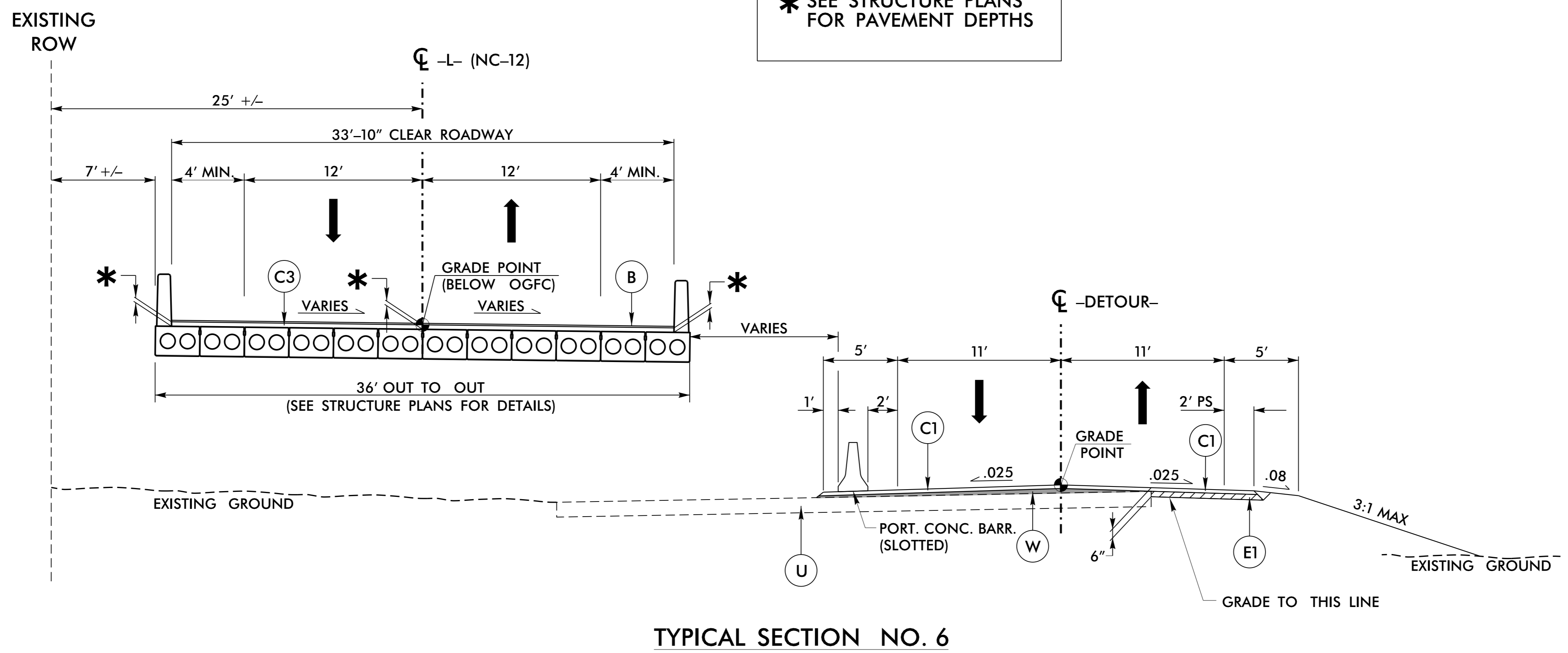
TYPICAL SECTION NO. 6 -DETOUR- STA. 29+06.50 TO STA. 39+46.67 (BEGIN EXIST. BRIDGE) -DETOUR- STA. 46+11.90 (END EXIST. BRIDGE) TO STA. 52+45.64
