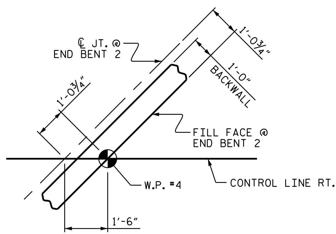
DETAIL "B"
