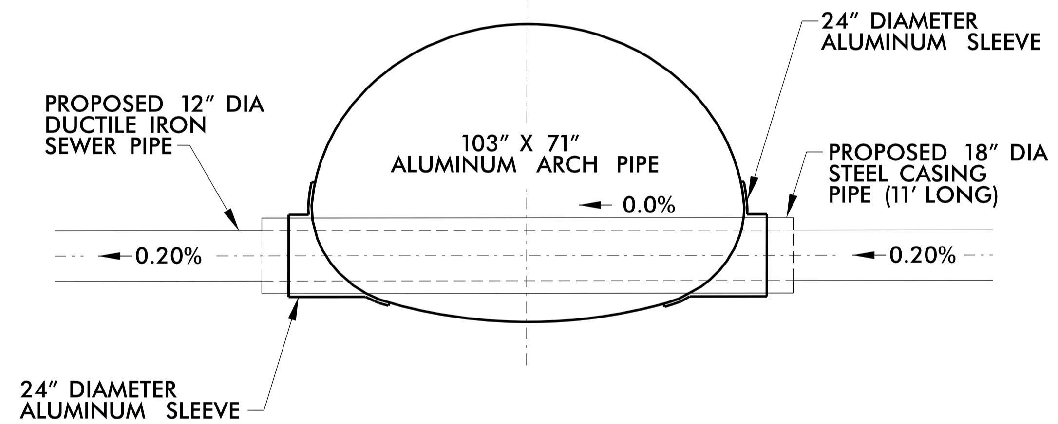
SECTION VIEW
