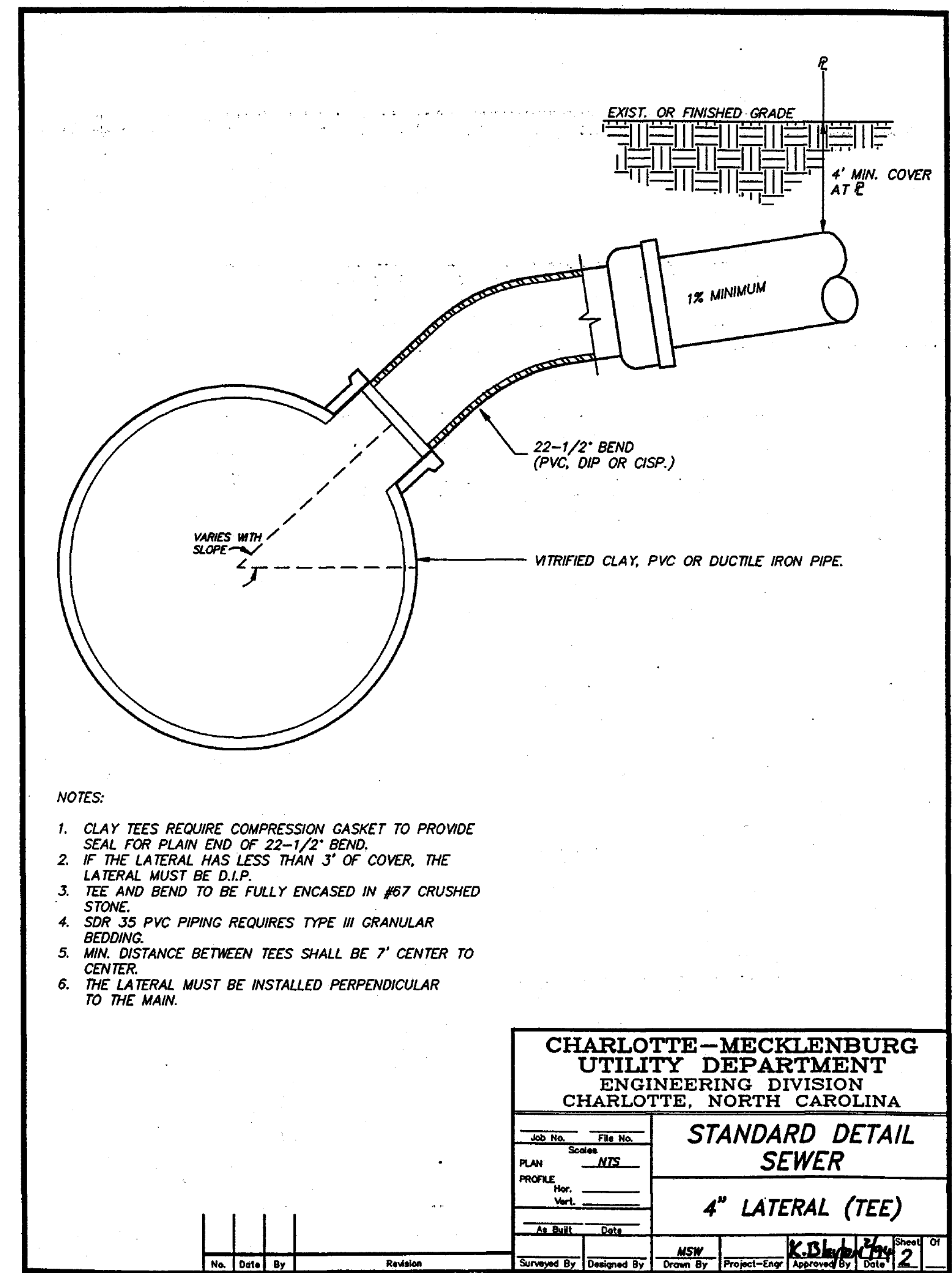
July 27, 1995 XV-58 Sewer Specifications/Details (SD)
