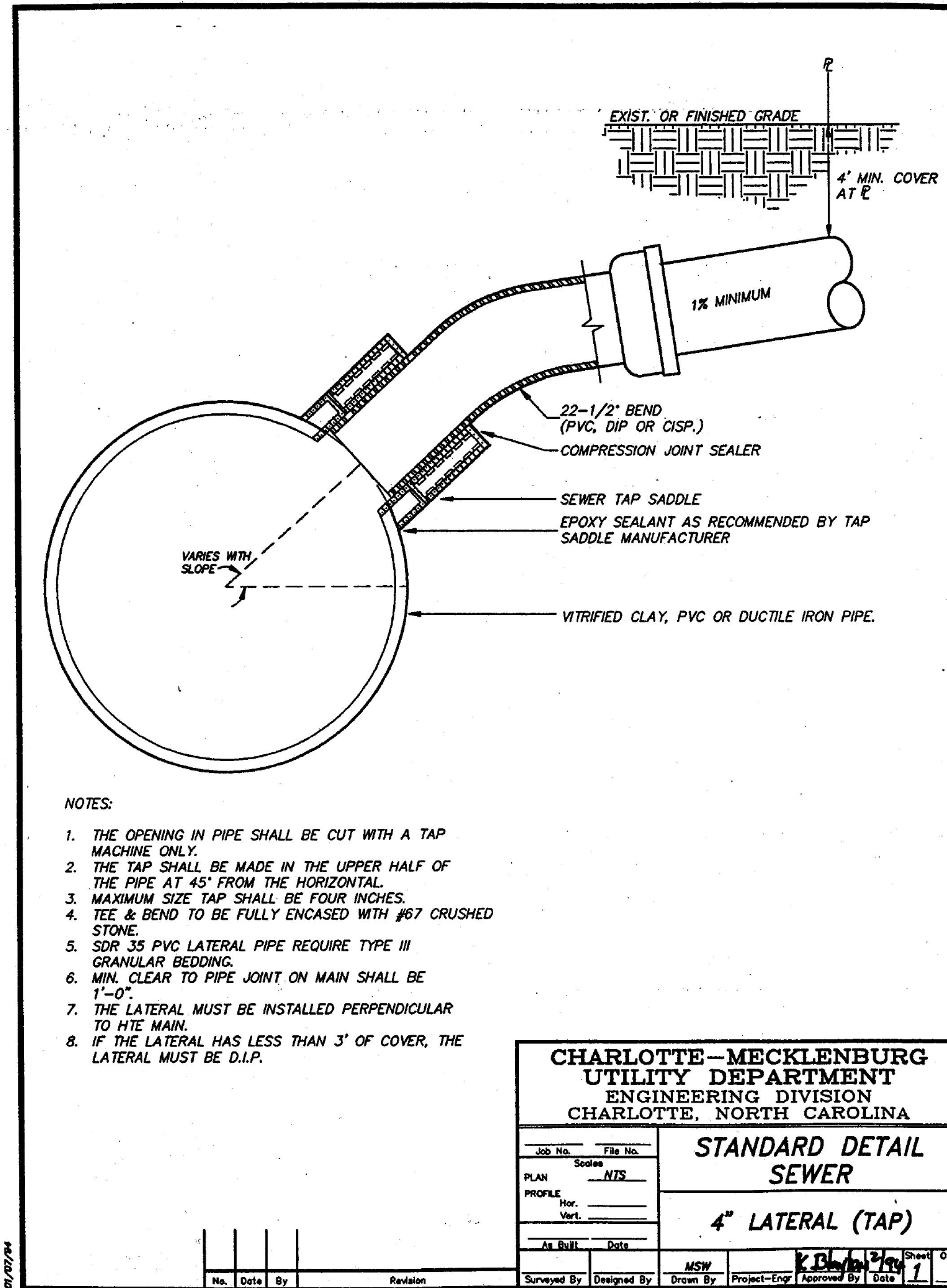
July 27, 1995 XV-57 Sewer Specifications/Details (SD)
