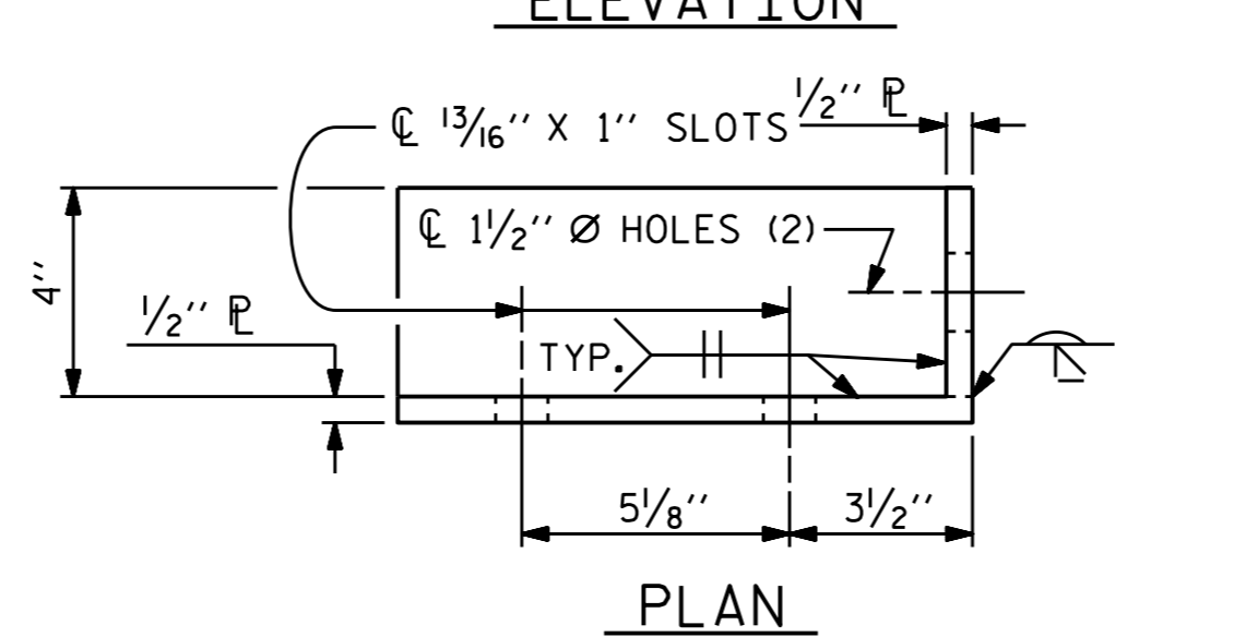
DETAILS FOR ATTACHMENT BRACKET (BOTTOM RAIL ONLY)
