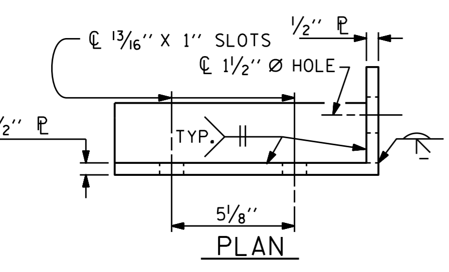
DETAILS FOR ATTACHMENT BRACKET (TOP & MIDDLE RAIL ONLY)
