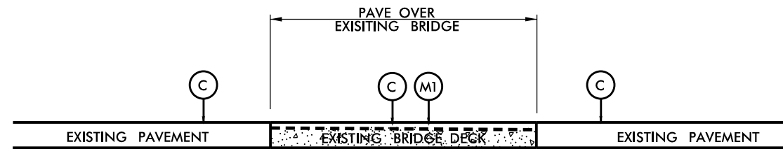
PAVE OVER EXISTING BRIDGE DECK Volunteer Rd SR 1136 (SEE BRIDGE DATA SHEET)
