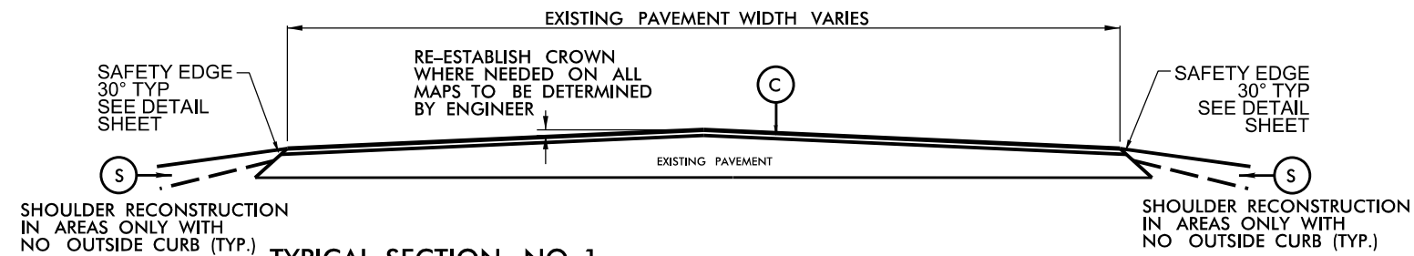
TYPICAL SECTION NO. 1 MAP NO.1 NC 8 MAP NO.2 SR 1136 VOLUNTEER RD. MAP NO.3 SR 1157 HIGH BRIDGE RD.
