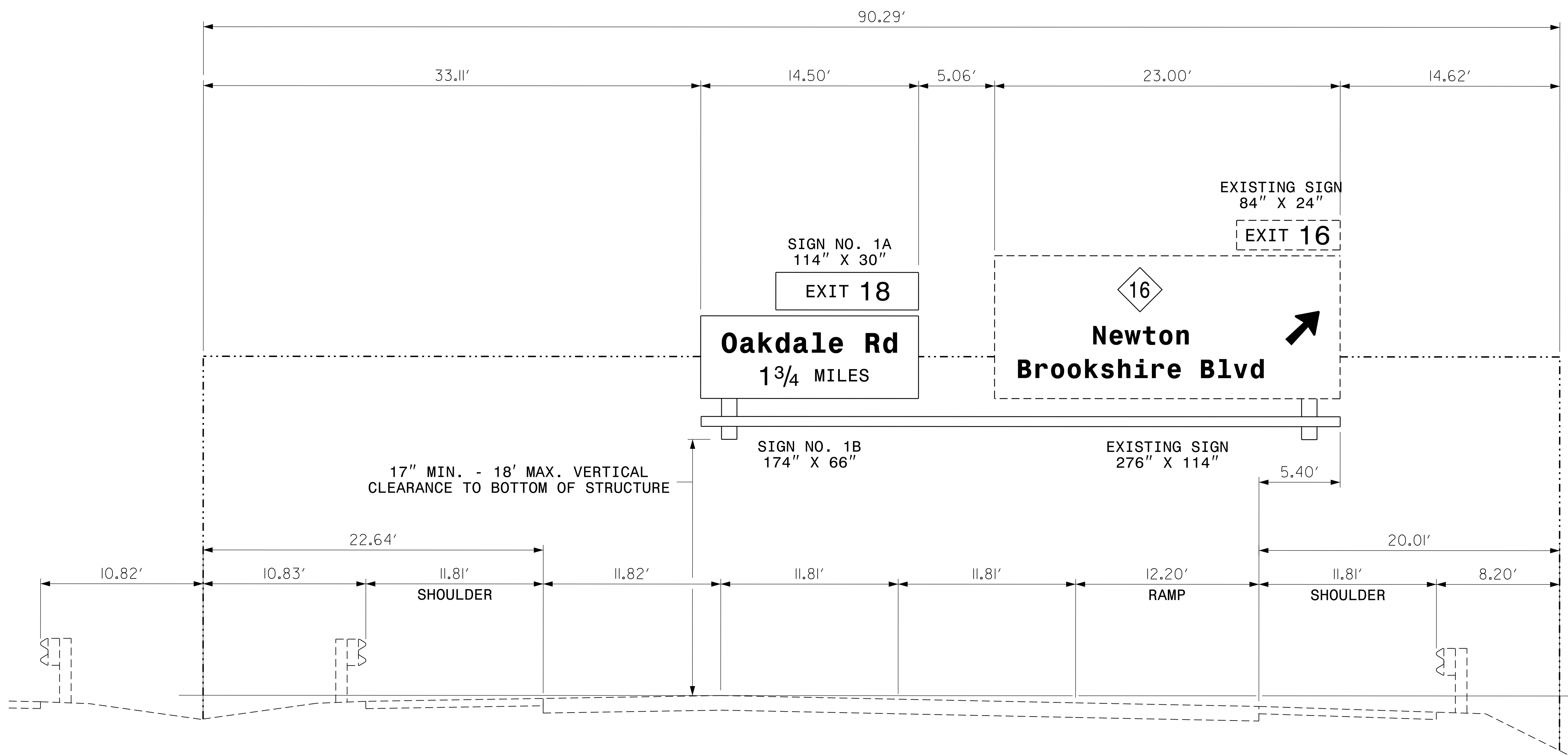
EXISTING OVERHEAD SIGN ASSEMBLY "A-A" I-485 -NB-
