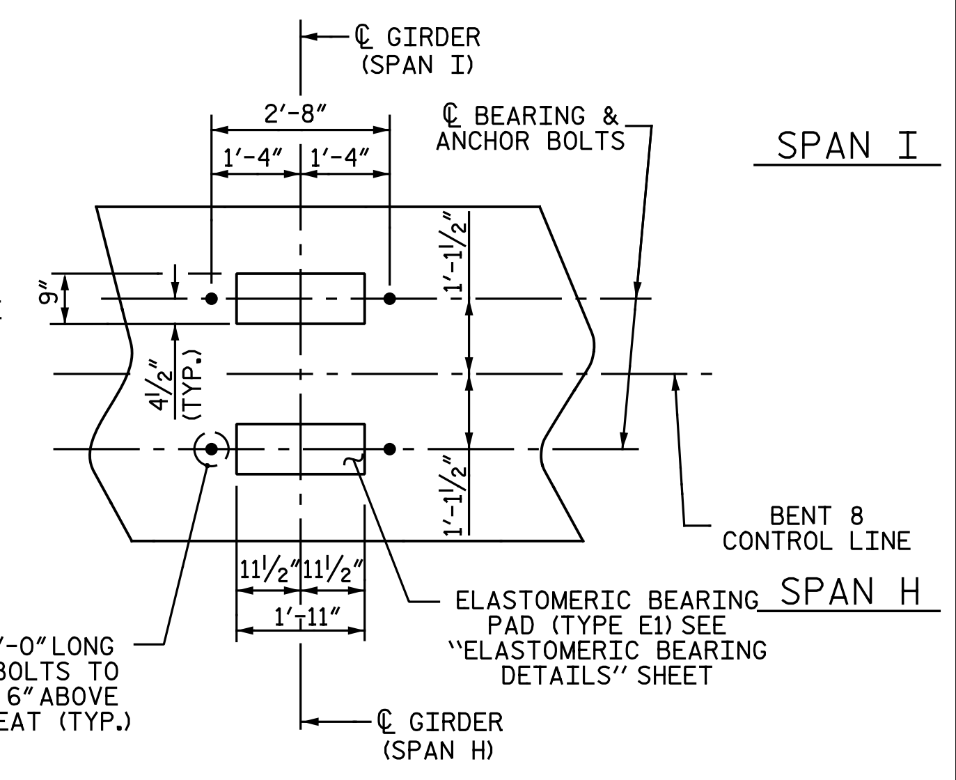
PLAN OF BEARINGS
