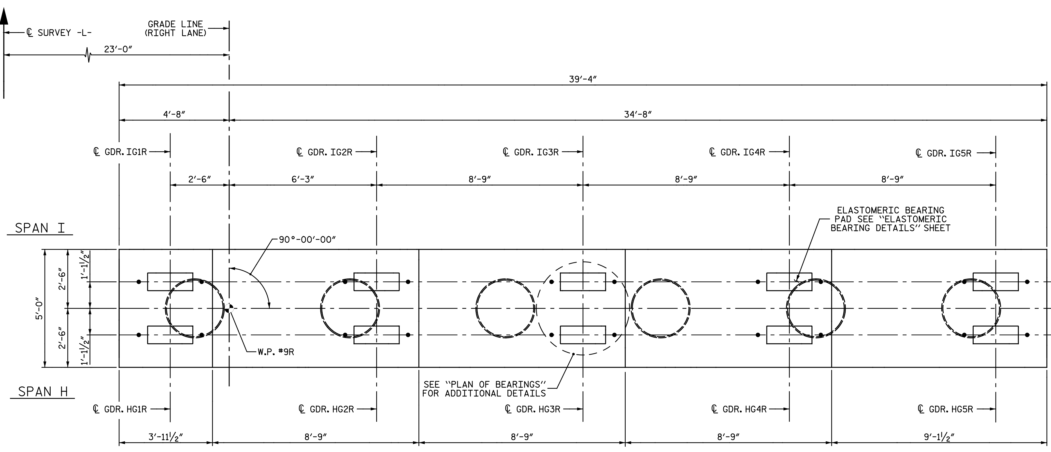
PLAN
