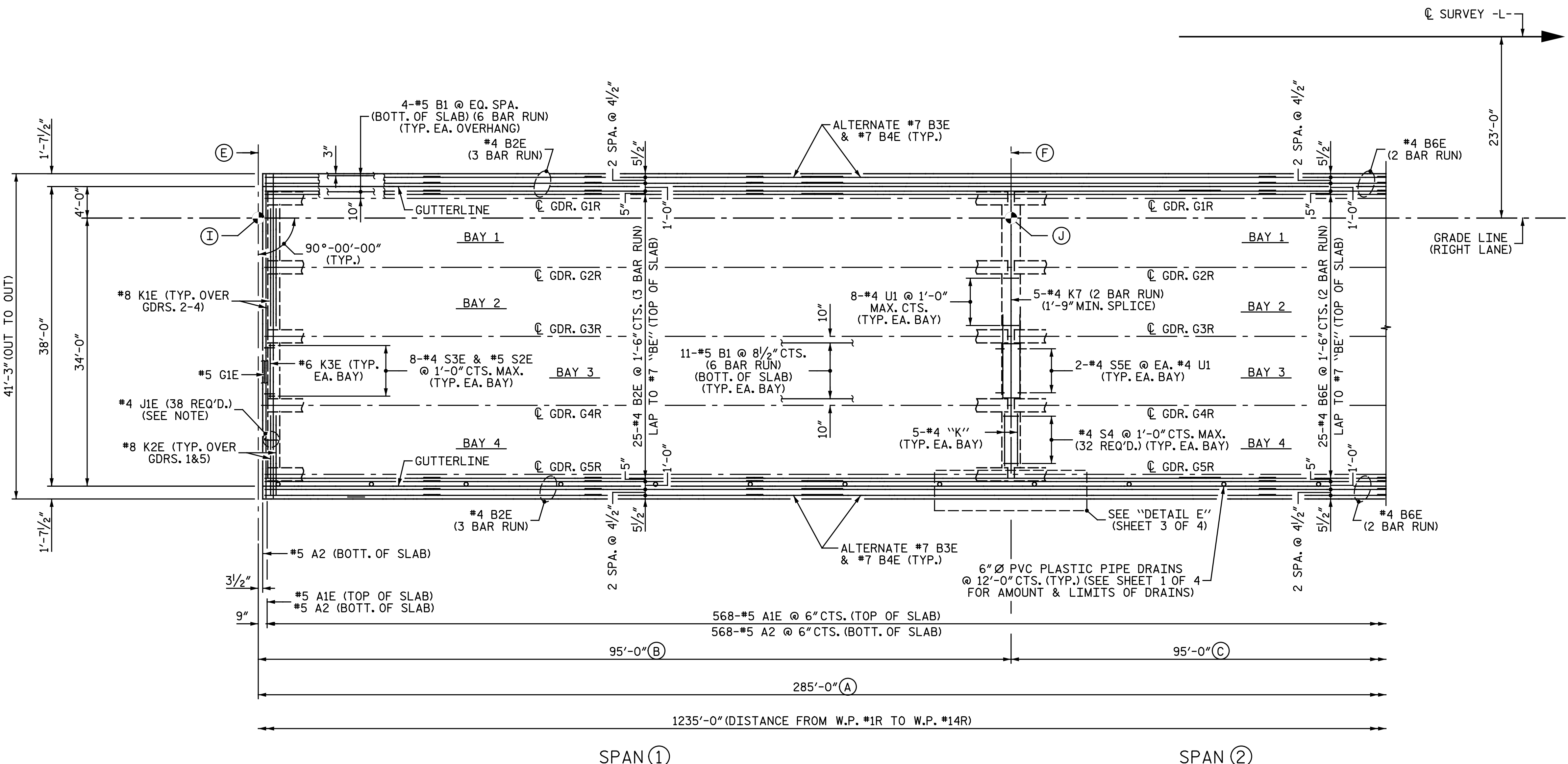
PART PLAN OF SPANS
