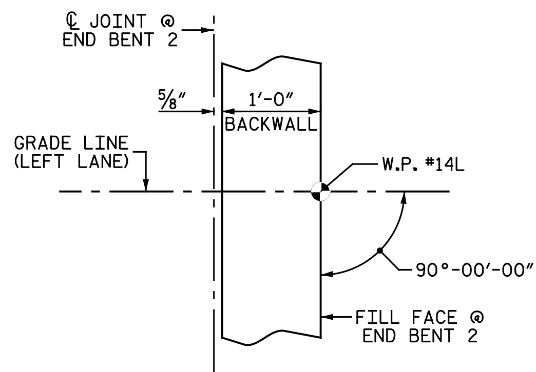
DETAIL G
