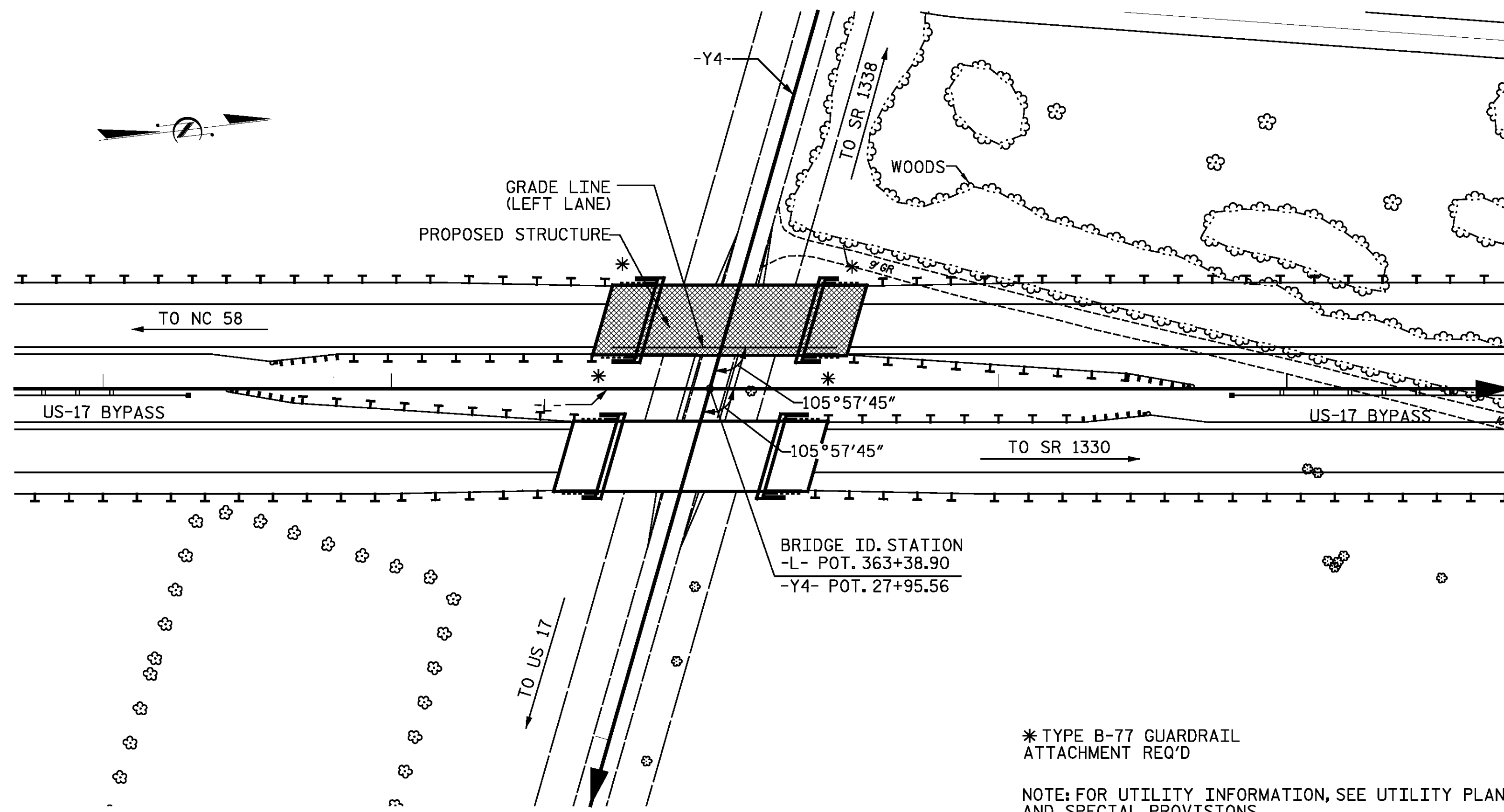
LOCATION SKETCH
