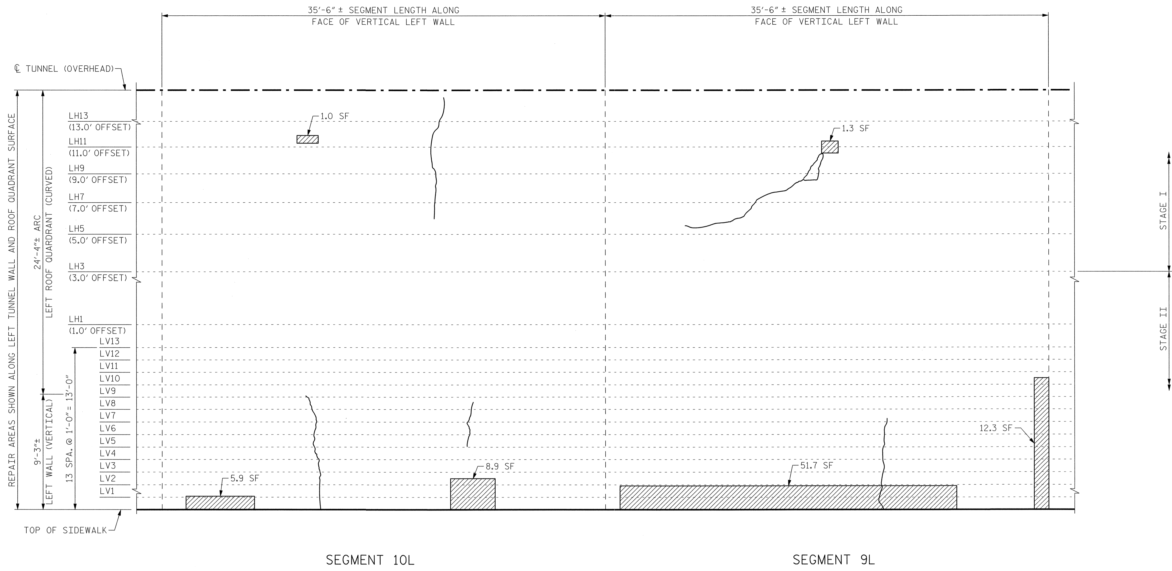
VIEW B-B: REPAIR SEGMENTS 9L & 10L TUNNEL SURFACE ELEVATION
