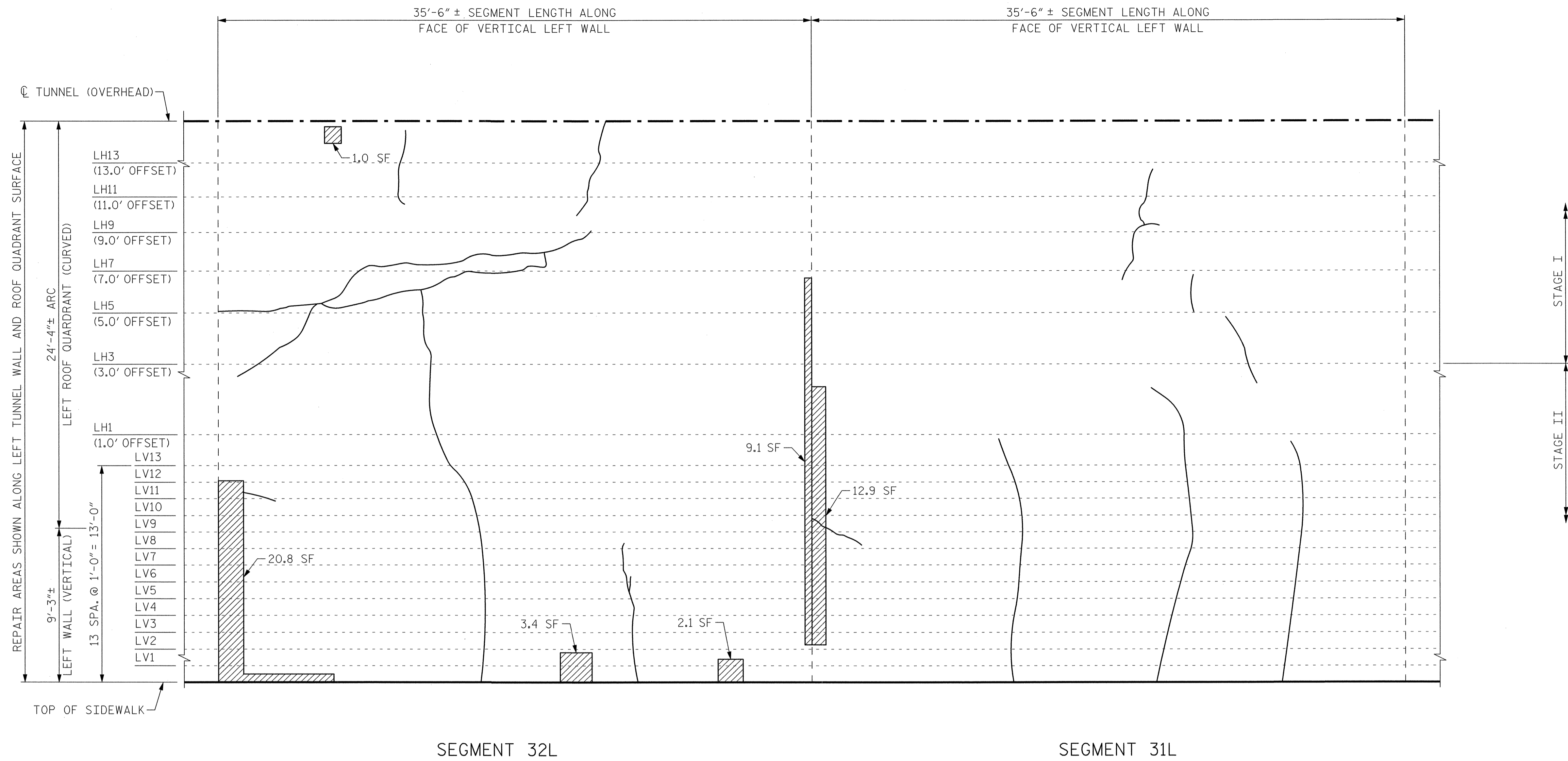
VIEW B-B: REPAIR SEGMENTS 31L & 32L TUNNEL SURFACE ELEVATION
