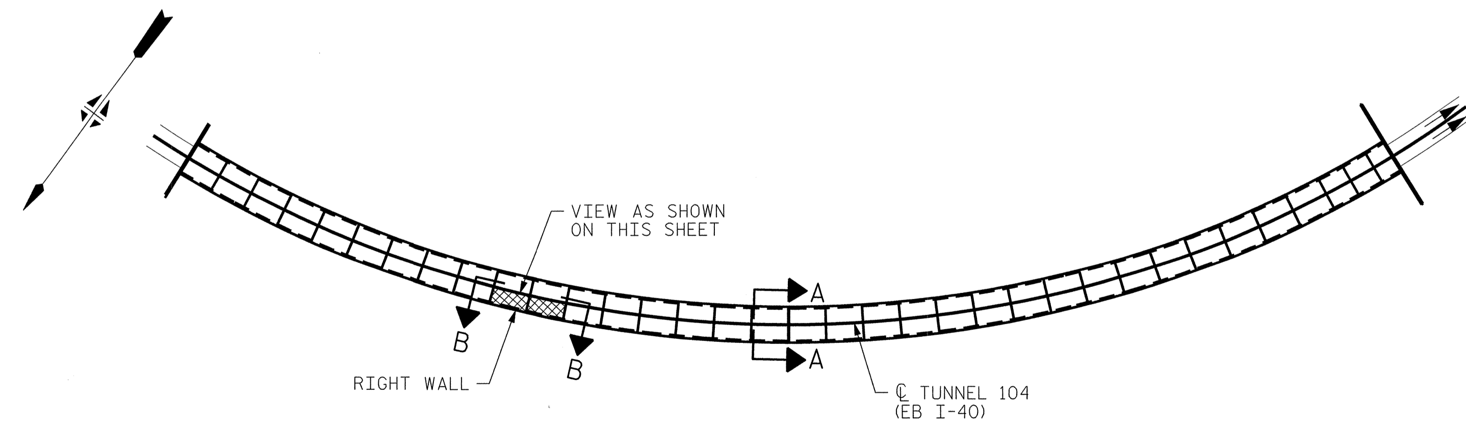
KEY PLAN
