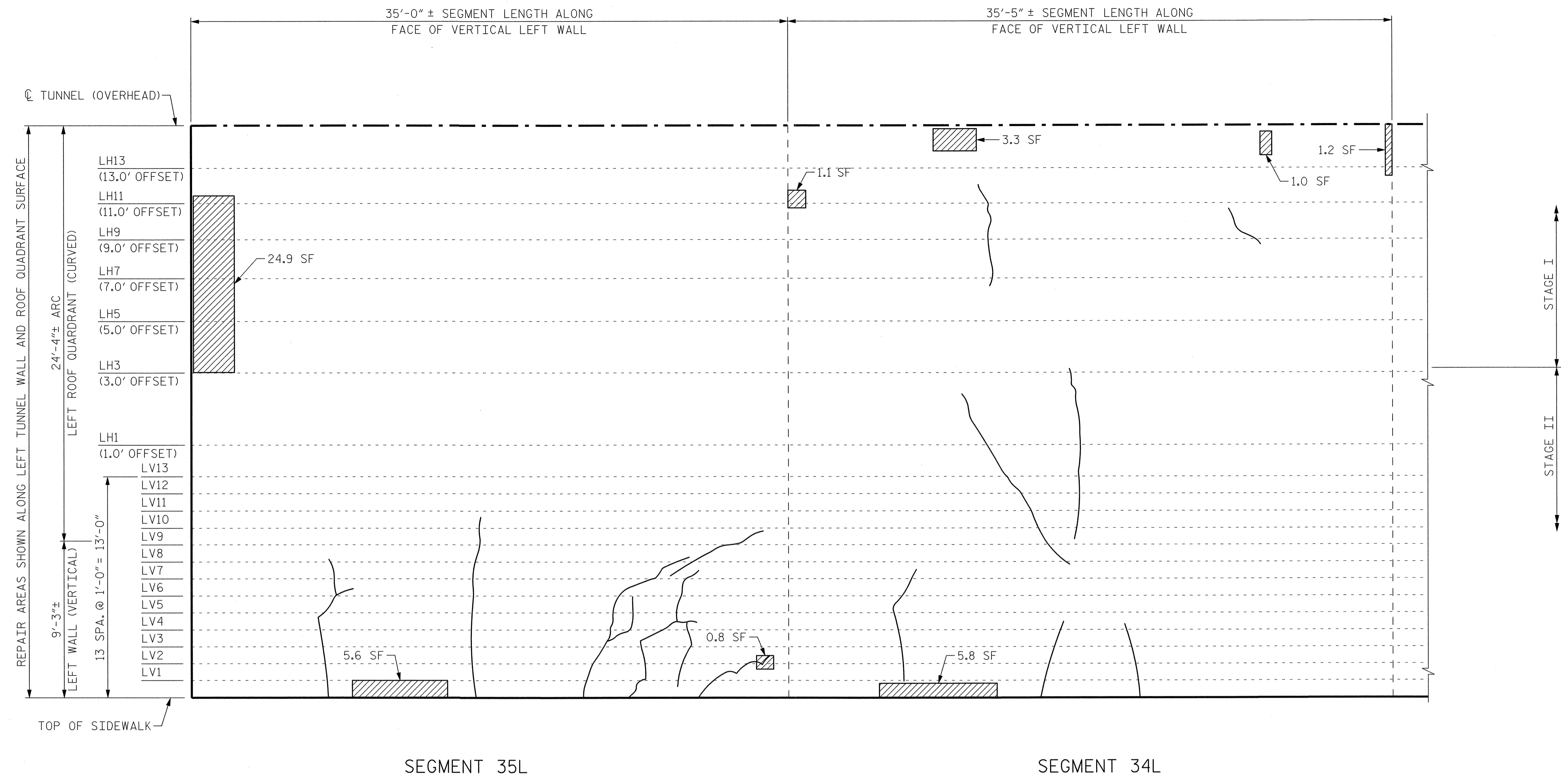
VIEW B-B: REPAIR SEGMENTS 34L & 35L TUNNEL SURFACE ELEVATION
