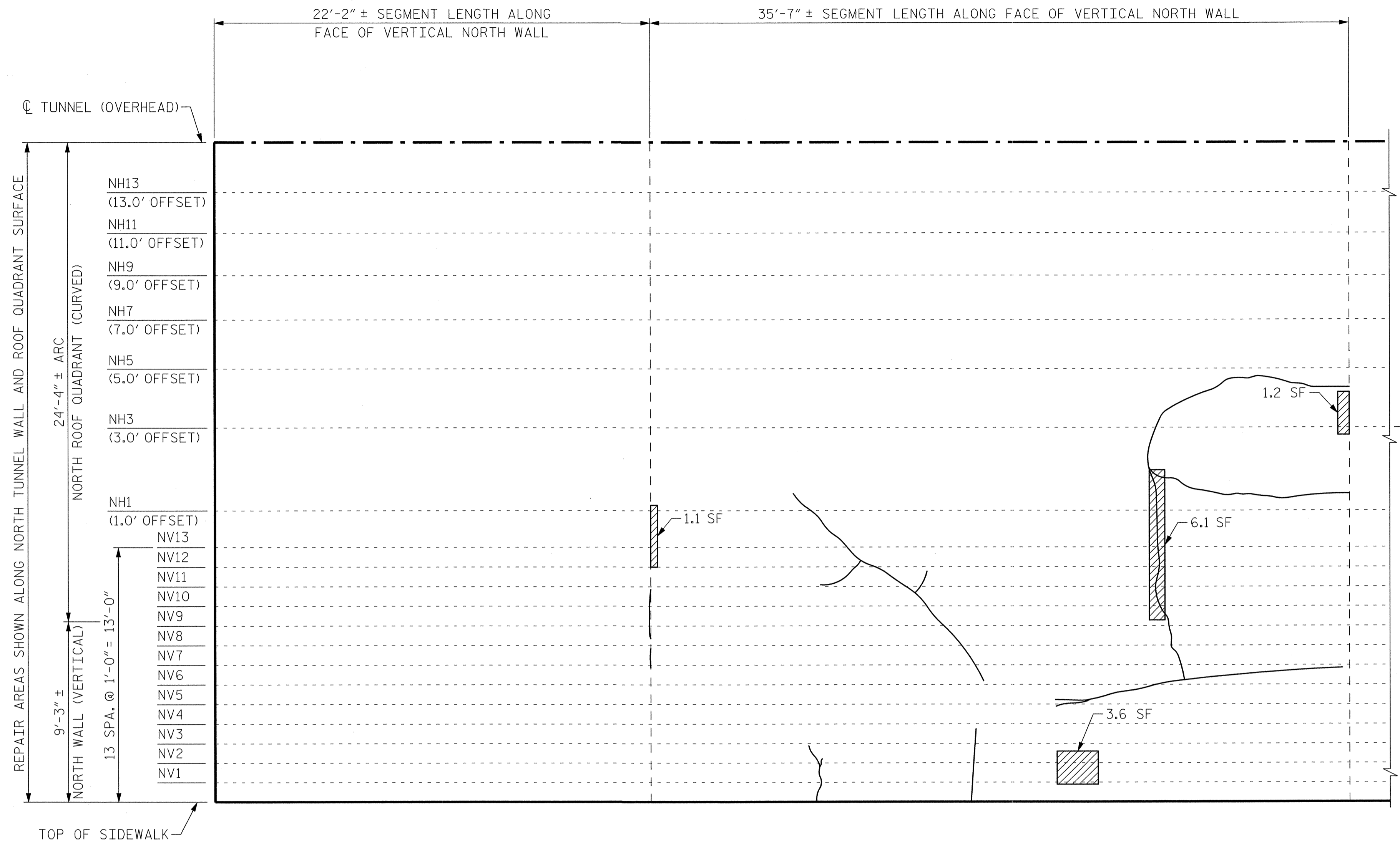
SEGMENT 30N SEGMENT 29N VIEW B-B: REPAIR SEGMENTS 29N & 30N TUNNEL SURFACE ELEVATION
