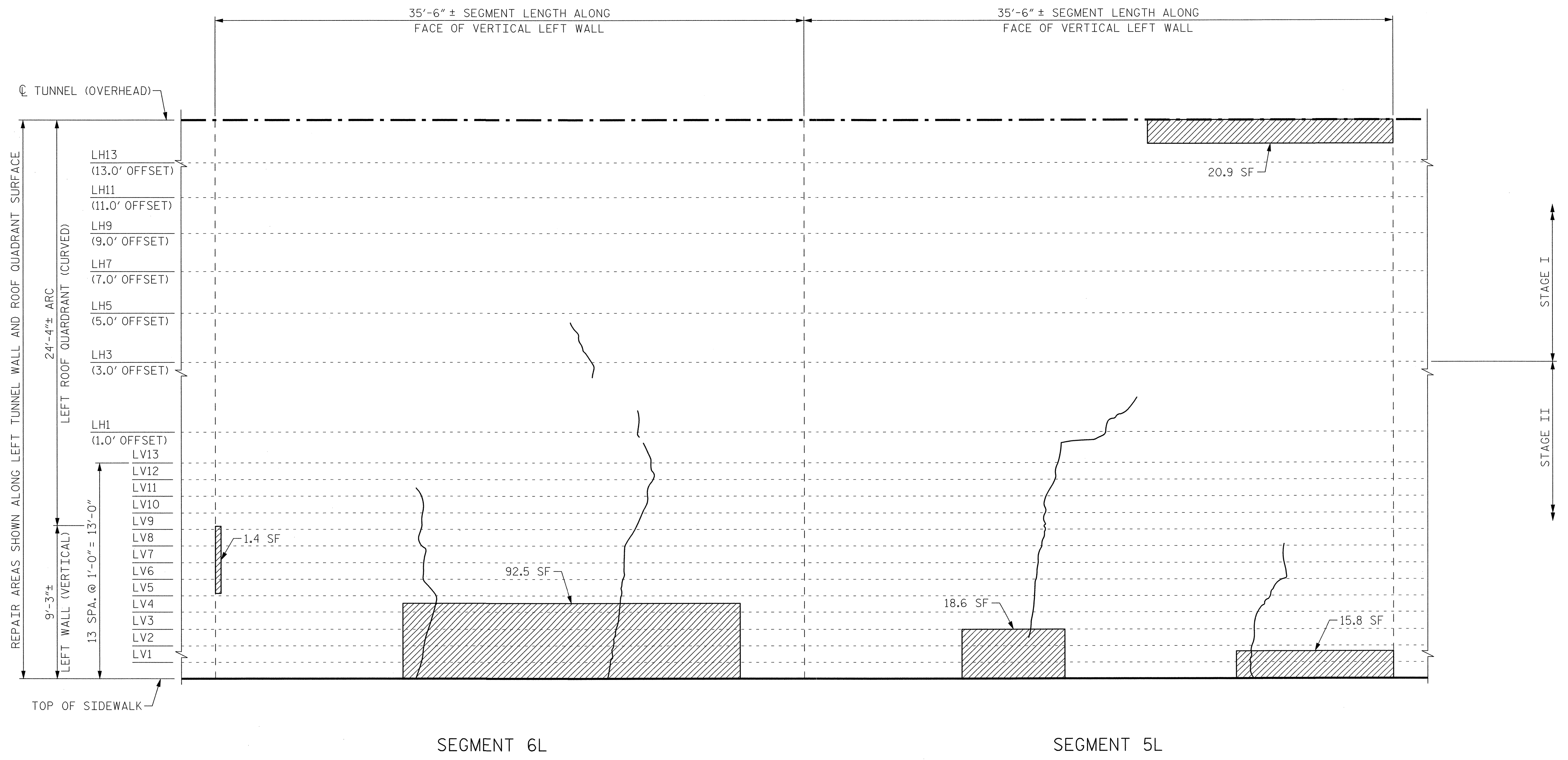
VIEW B-B: REPAIR SEGMENTS 5L & 6L TUNNEL SURFACE ELEVATION
