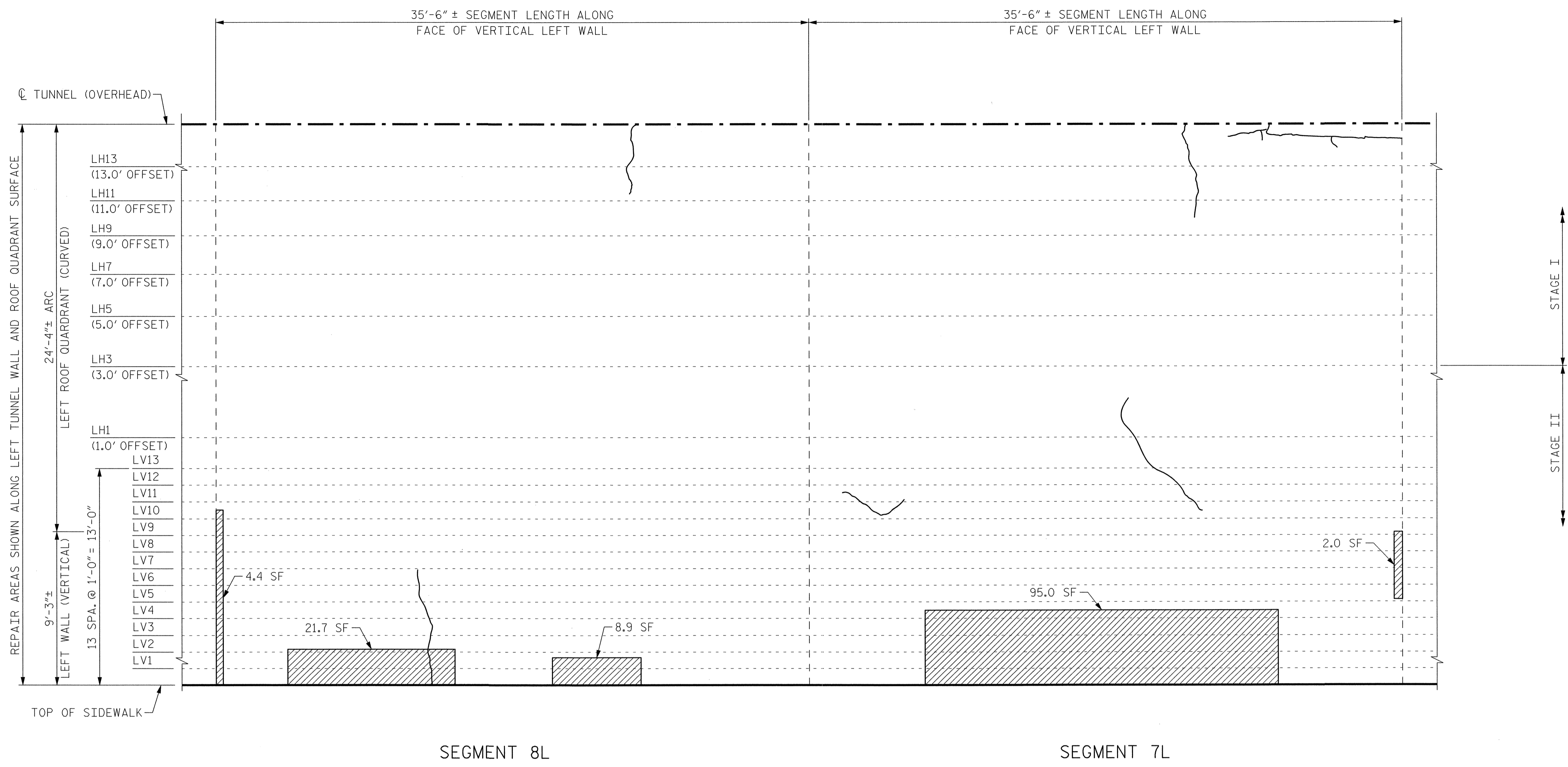
VIEW B-B: REPAIR SEGMENTS 7L & 8L TUNNEL SURFACE ELEVATION
