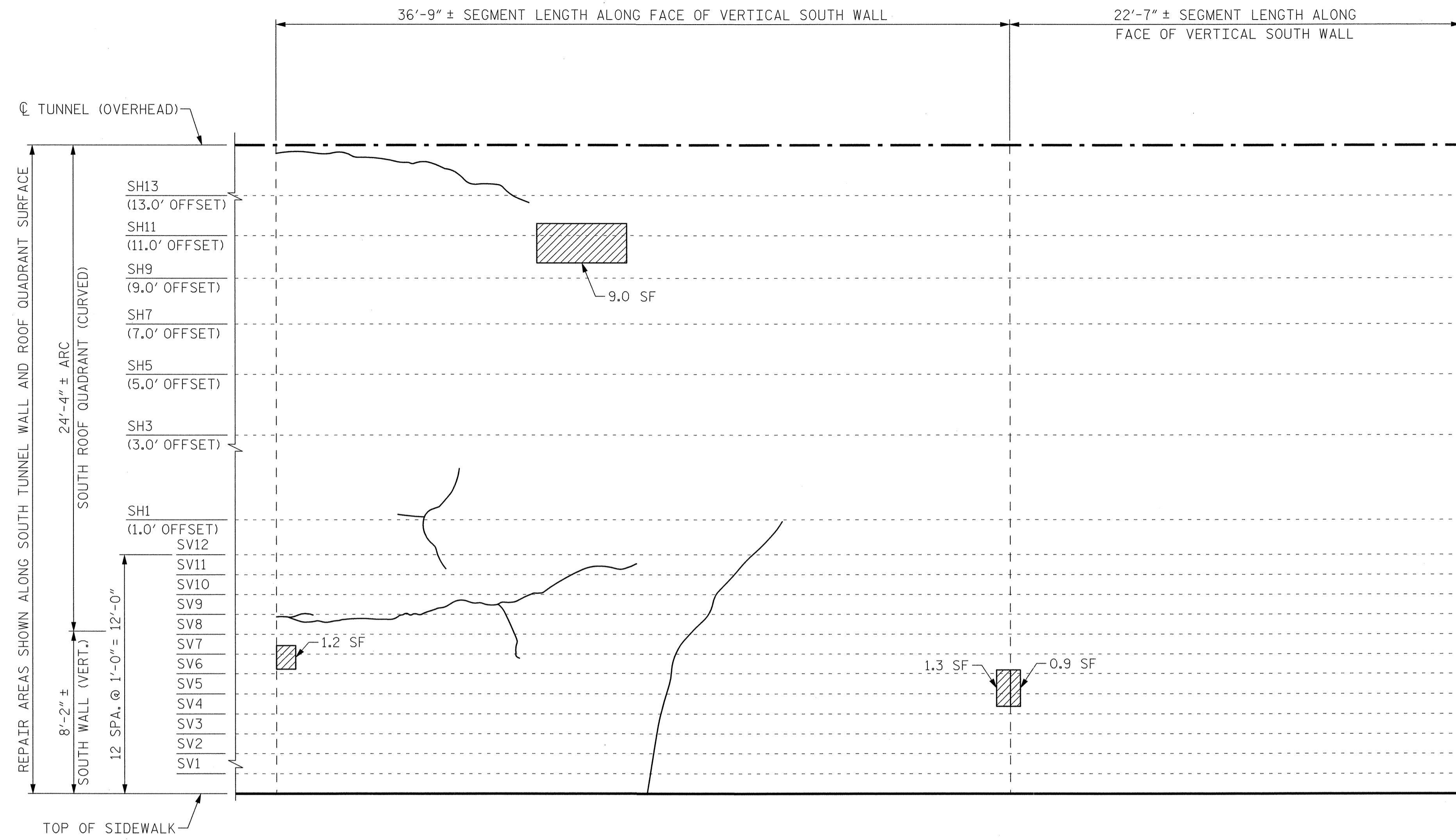
SEGMENT 29S SEGMENT 30S VIEW B-B: REPAIR SEGMENTS 29S & 30S TUNNEL SURFACE ELEVATION
