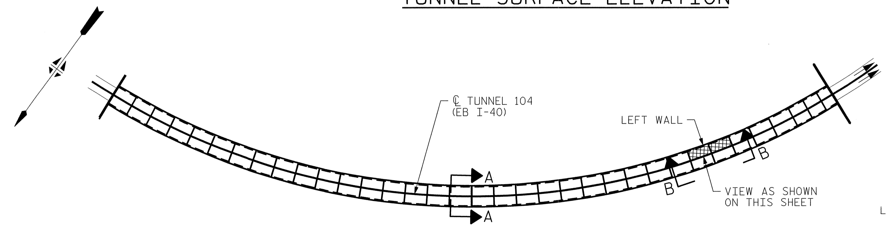
VIEW B-B: REPAIR SEGMENTS 7L & 8L TUNNEL SURFACE ELEVATION
