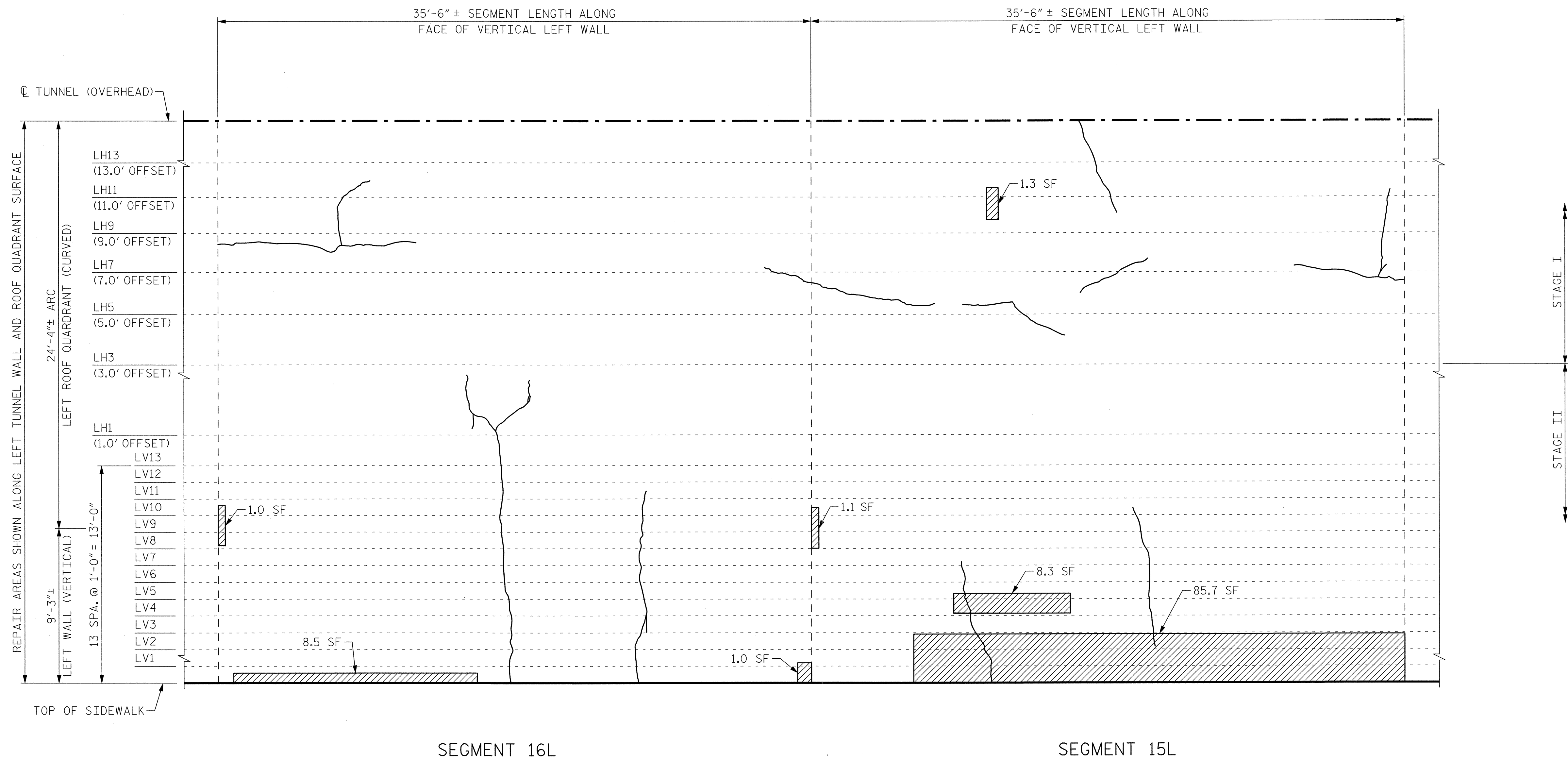
VIEW B-B: REPAIR SEGMENTS 15L & 16L TUNNEL SURFACE ELEVATION
