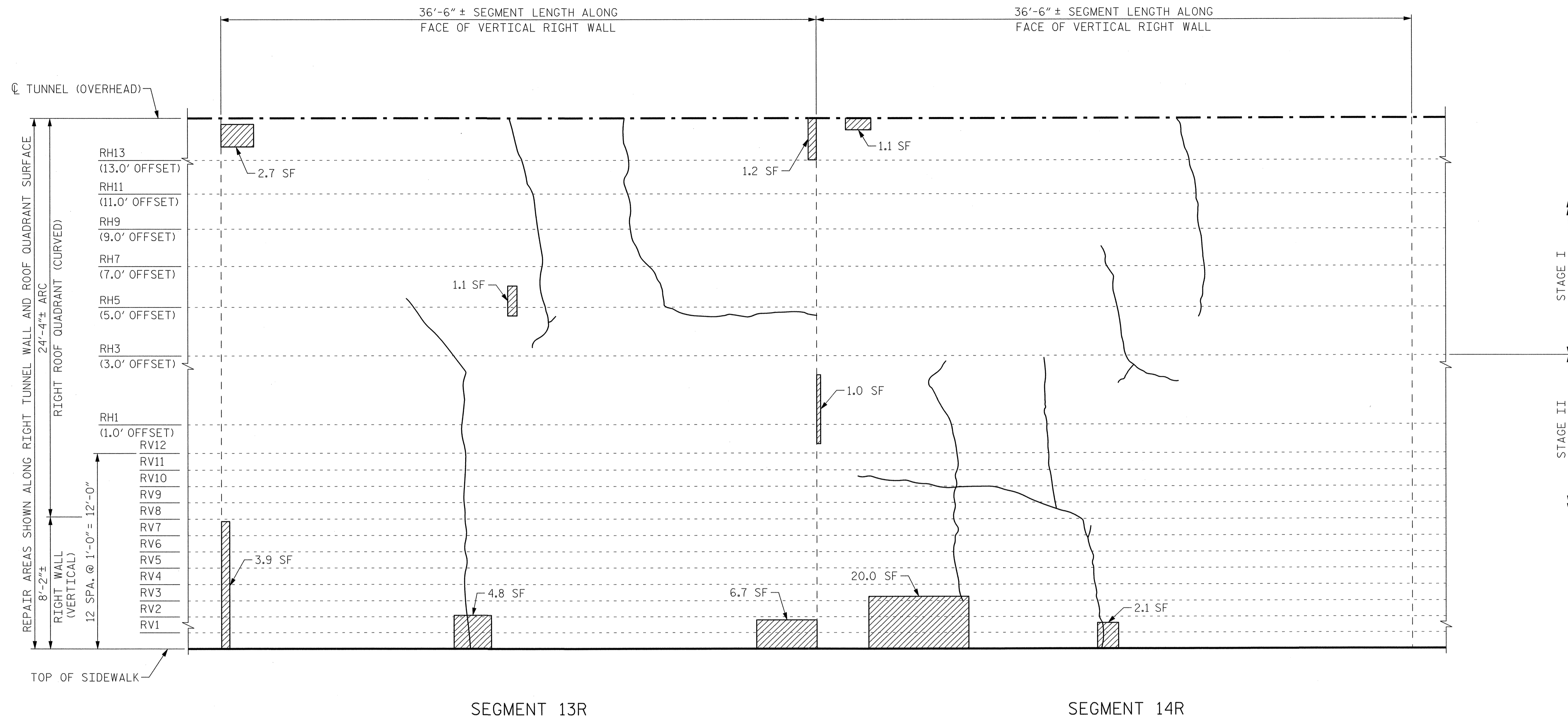
VIEW B-B: REPAIR SEGMENTS 13R & 14R TUNNEL SURFACE ELEVATION
