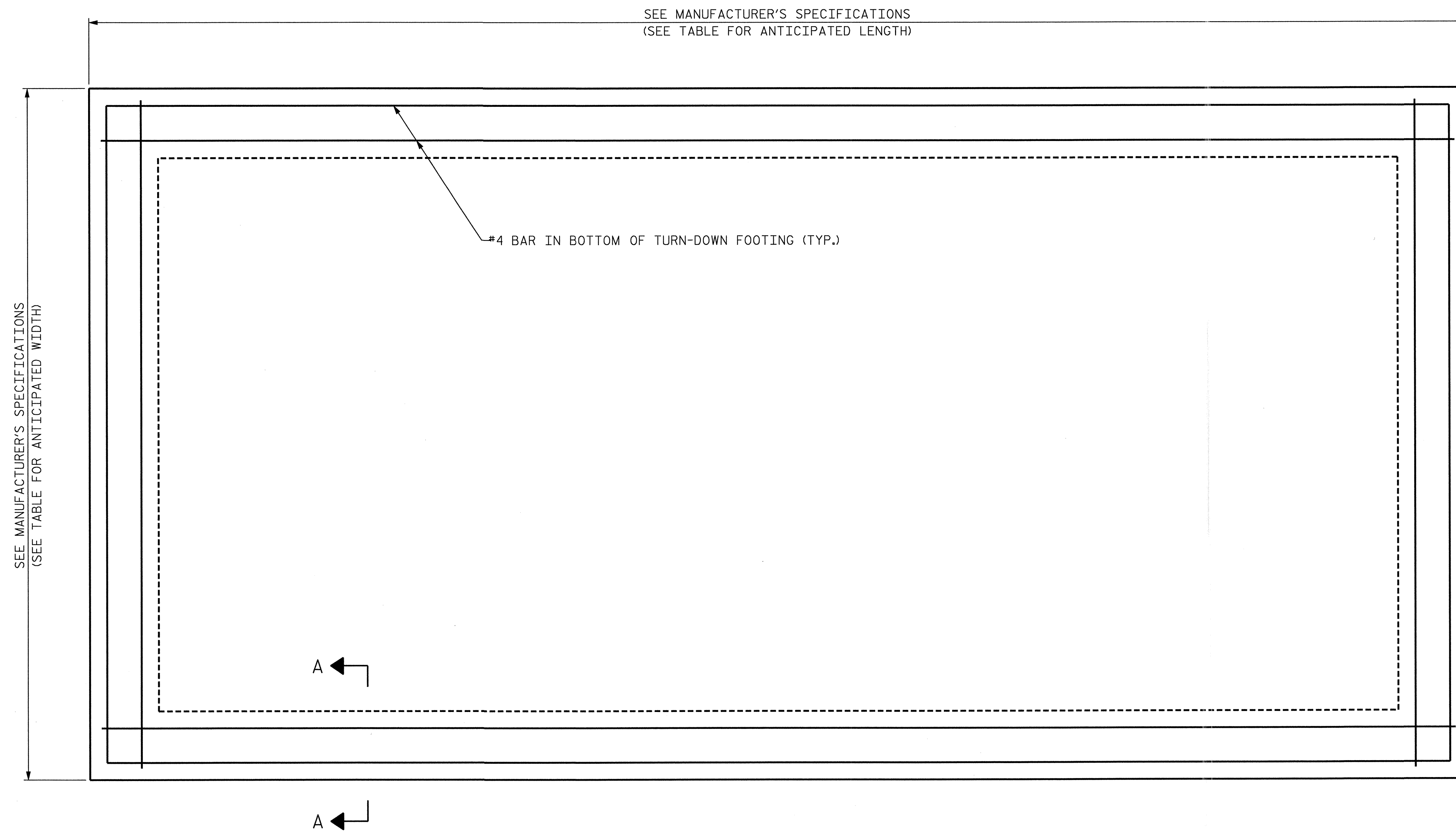
PLAN
