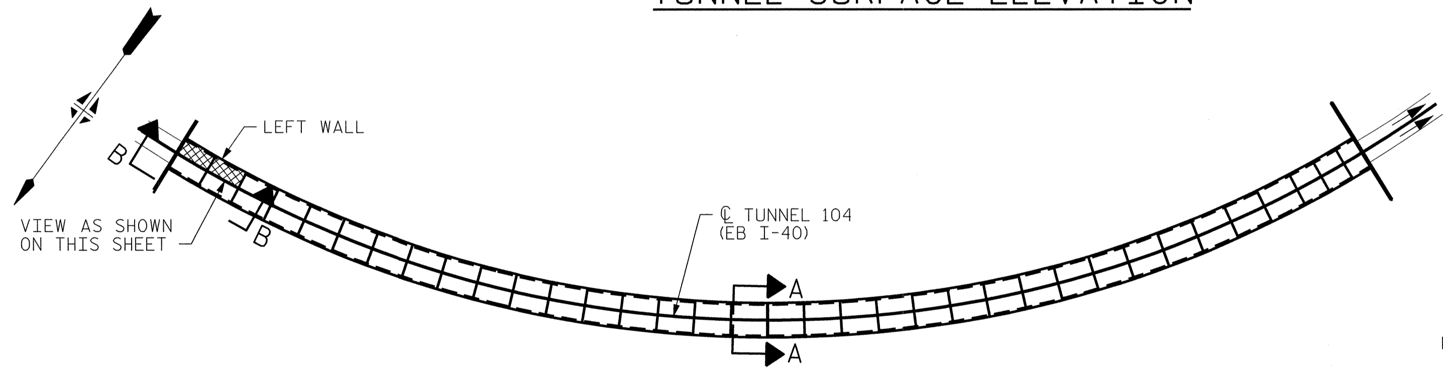
VIEW B-B: REPAIR SEGMENTS 34L & 35L TUNNEL SURFACE ELEVATION
