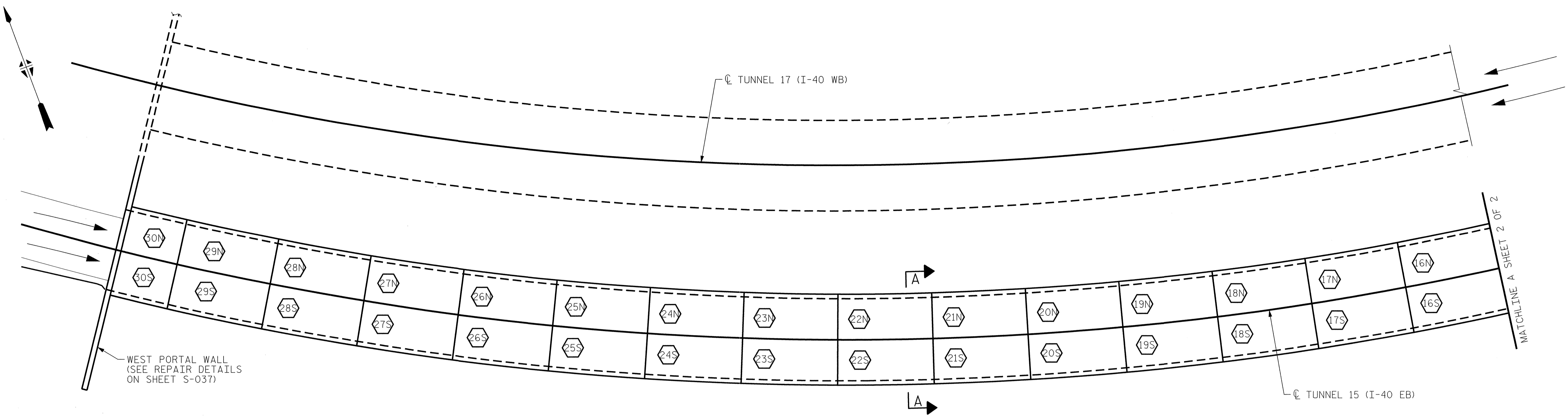
PARTIAL PLAN OF REPAIR SEGMENTS - TUNNEL 15
