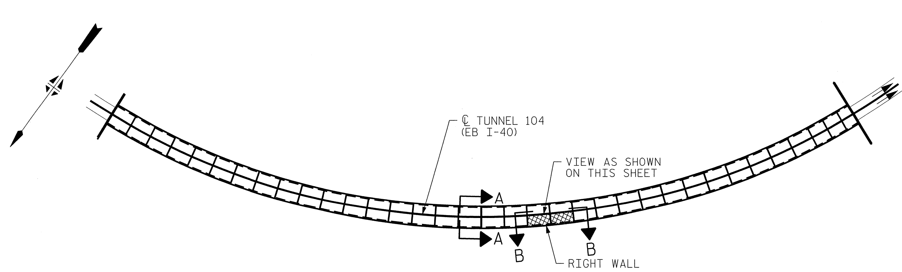
KEY PLAN
