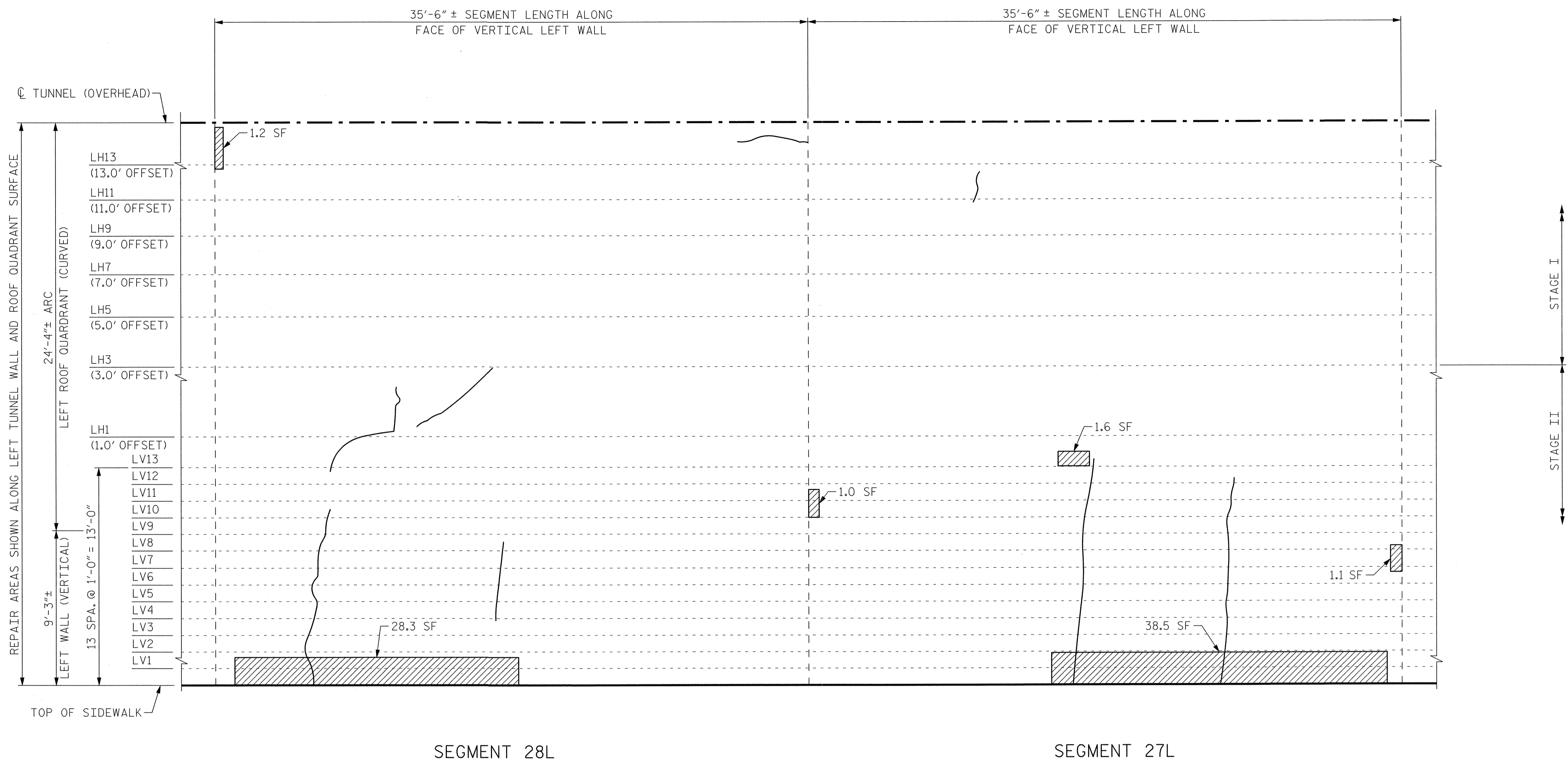
VIEW B-B: REPAIR SEGMENTS 27L & 28L TUNNEL SURFACE ELEVATION
