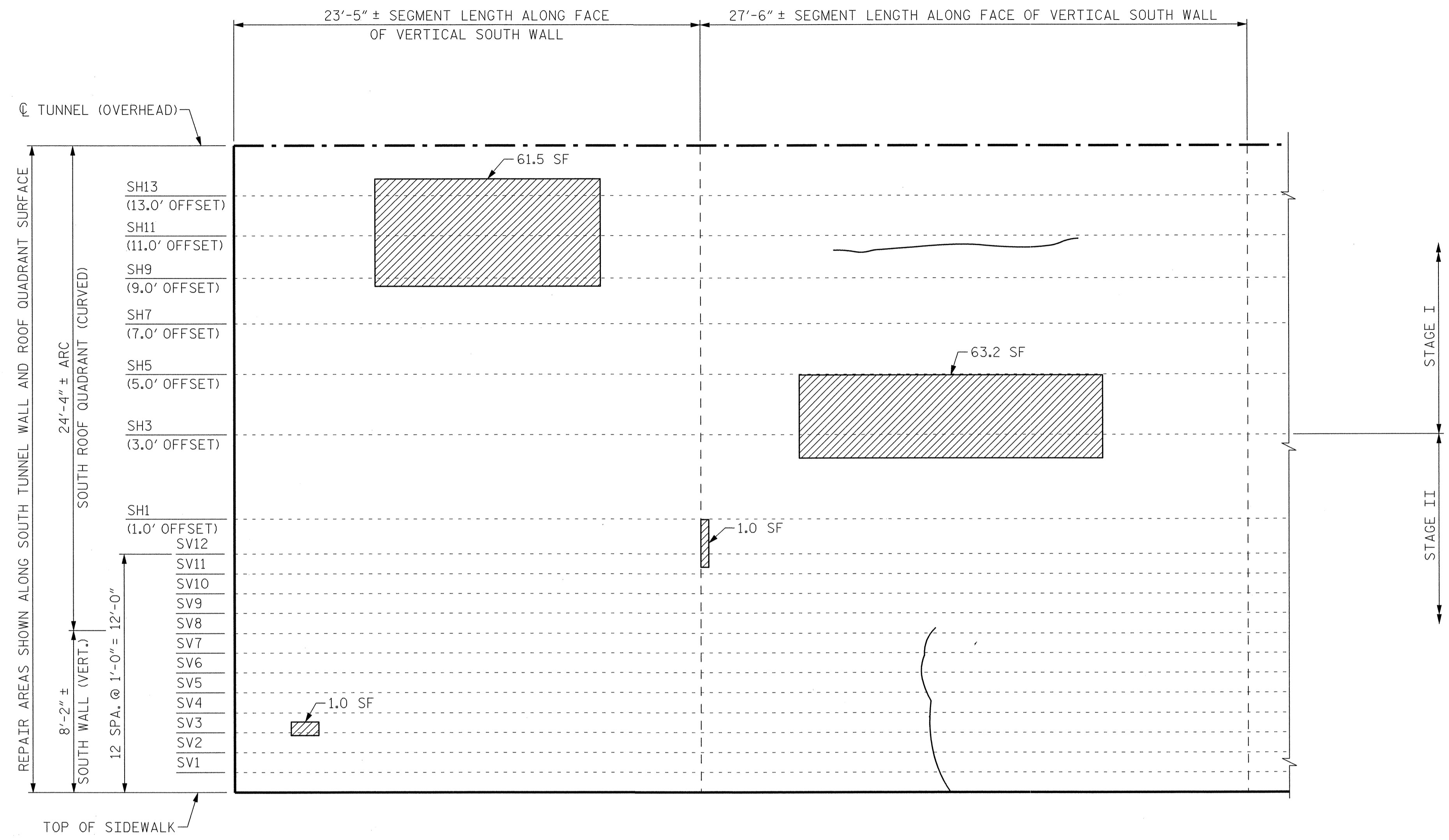
SEGMENT 1S SEGMENT 2S VIEW B-B: REPAIR SEGMENTS 1S & 2S TUNNEL SURFACE ELEVATION
