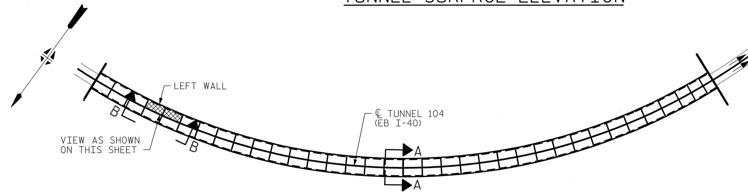
VIEW B-B: REPAIR SEGMENTS 31L & 32L TUNNEL SURFACE ELEVATION
