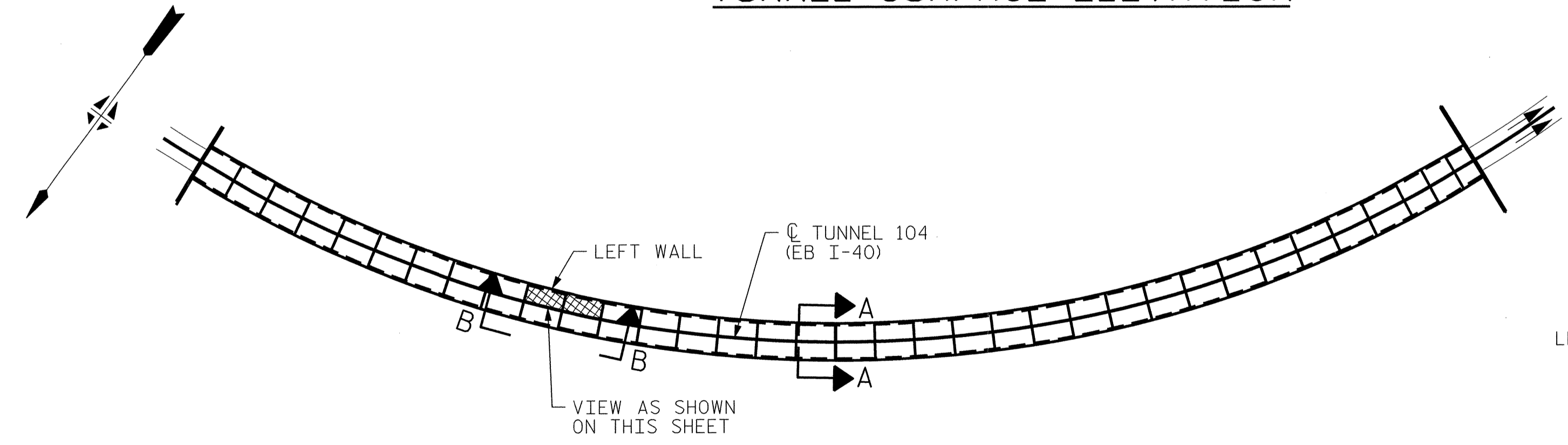
VIEW B-B: REPAIR SEGMENTS 25L & 26L TUNNEL SURFACE ELEVATION
