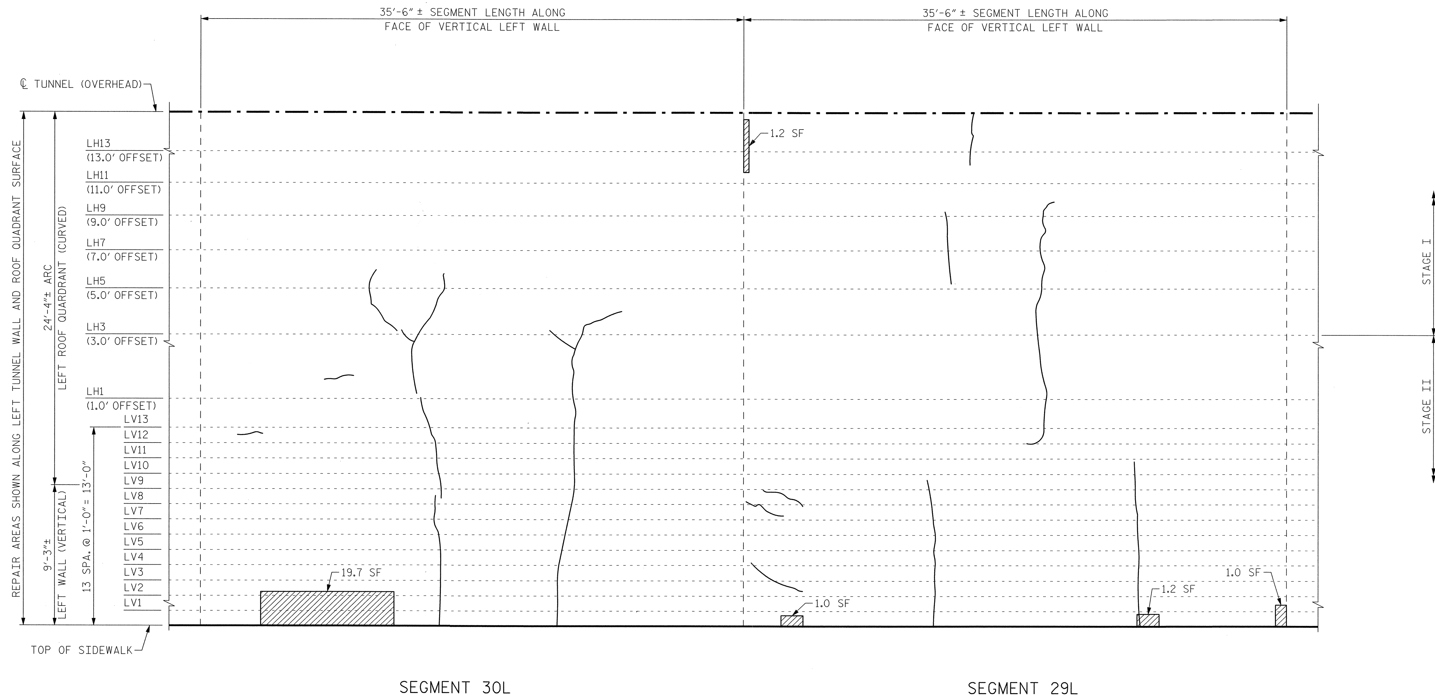
VIEW B-B: REPAIR SEGMENTS 29L & 30L TUNNEL SURFACE ELEVATION
