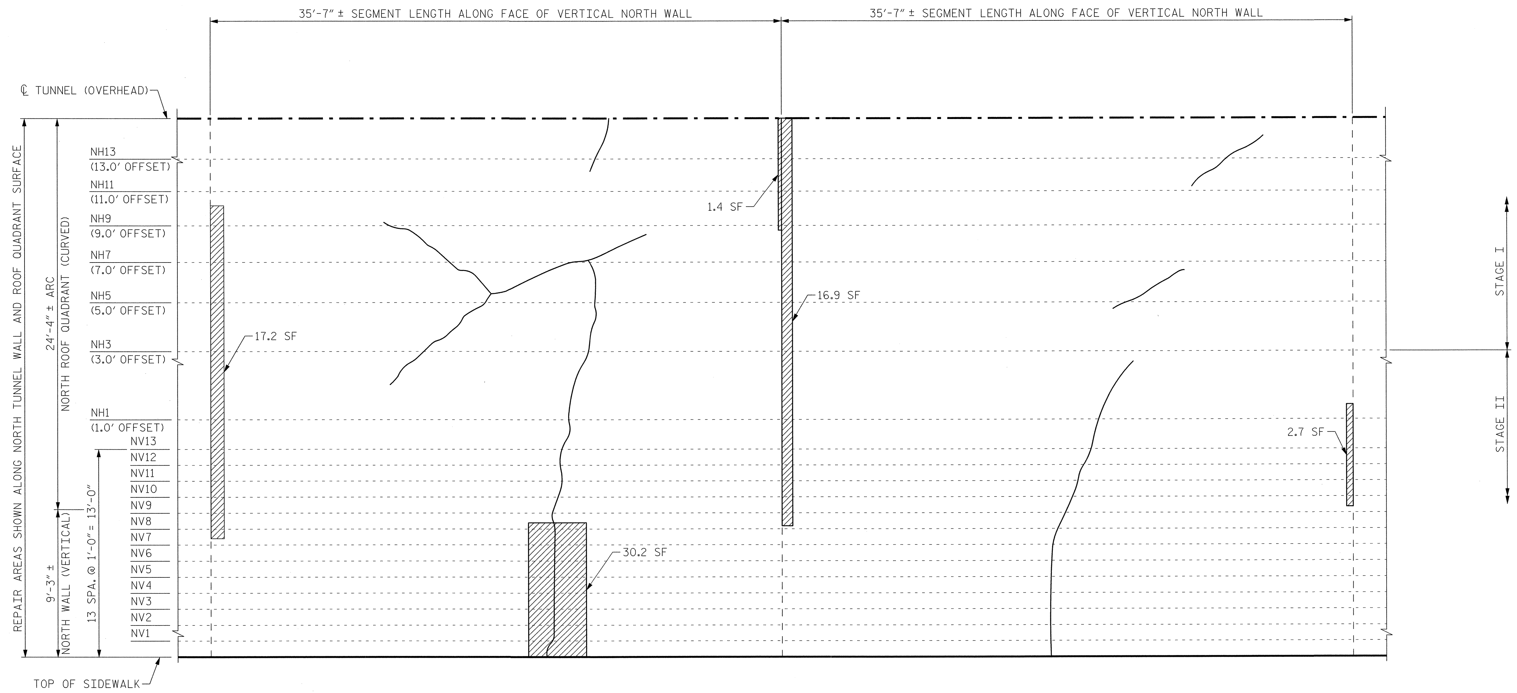
SEGMENT 26N SEGMENT 25N VIEW B-B: REPAIR SEGMENTS 25N & 26N TUNNEL SURFACE ELEVATION
