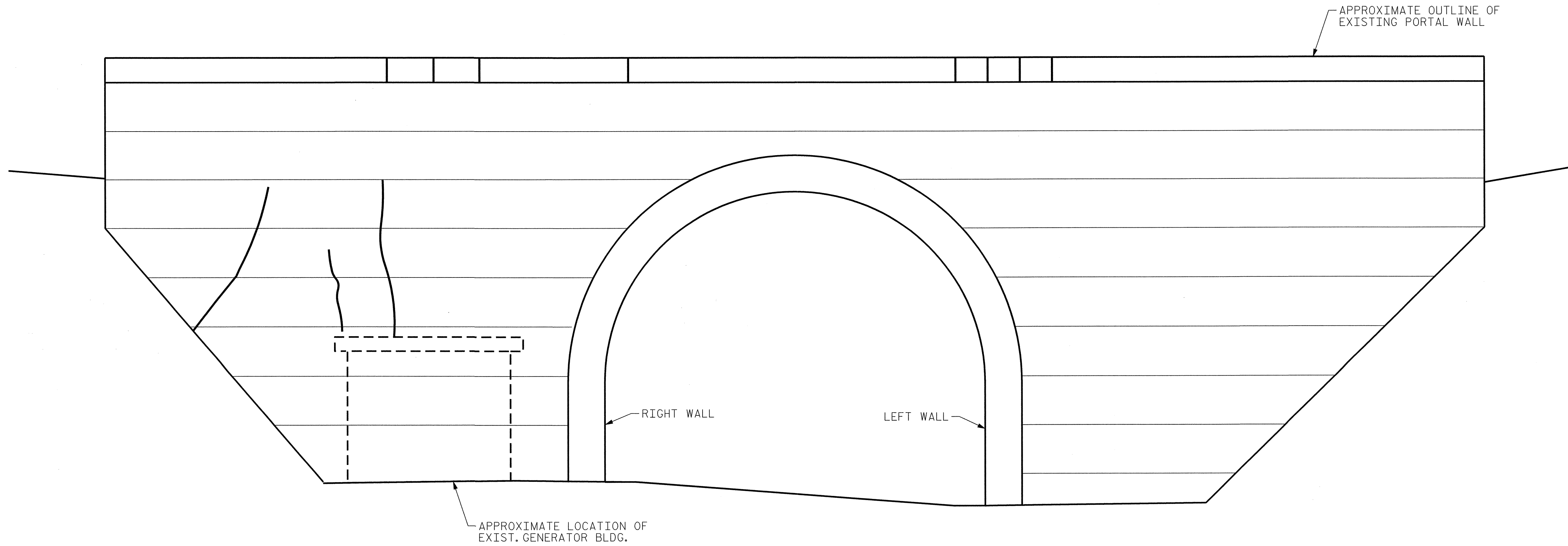
EXIT PORTAL WALL (SOUTH OR EAST END)
