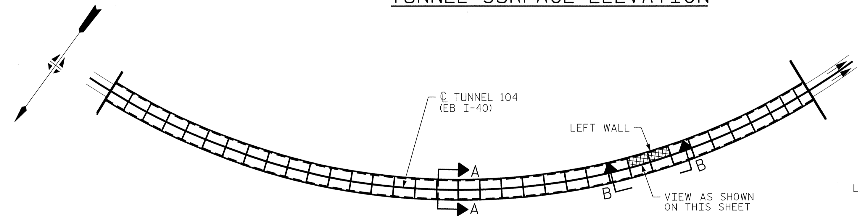
VIEW B-B: REPAIR SEGMENTS 9L & 10L TUNNEL SURFACE ELEVATION
