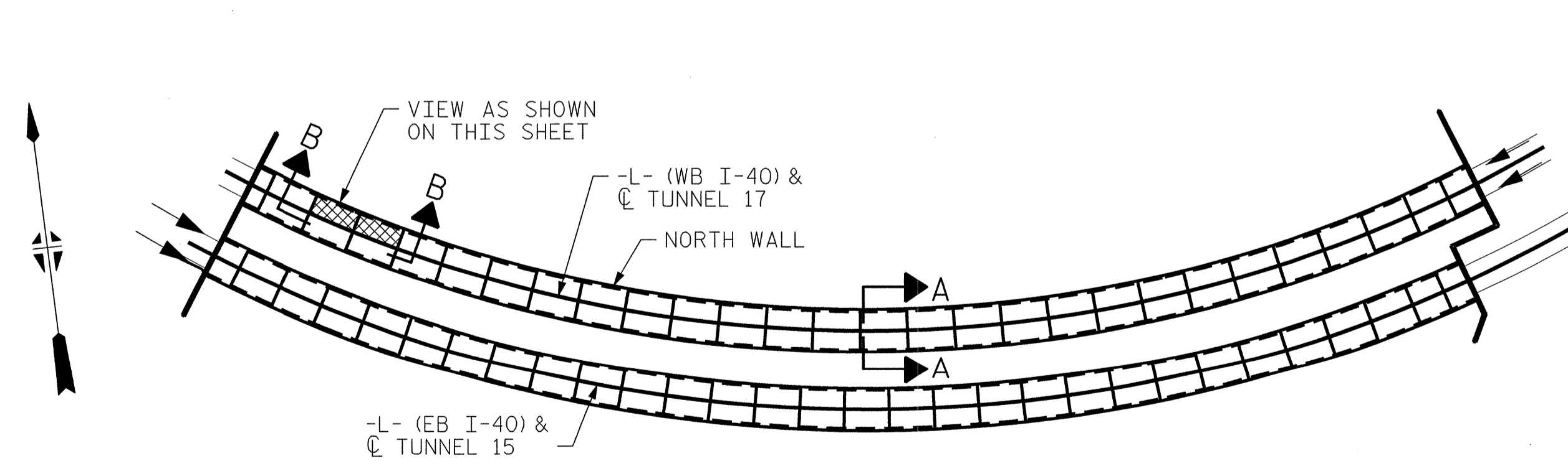
KEY PLAN
