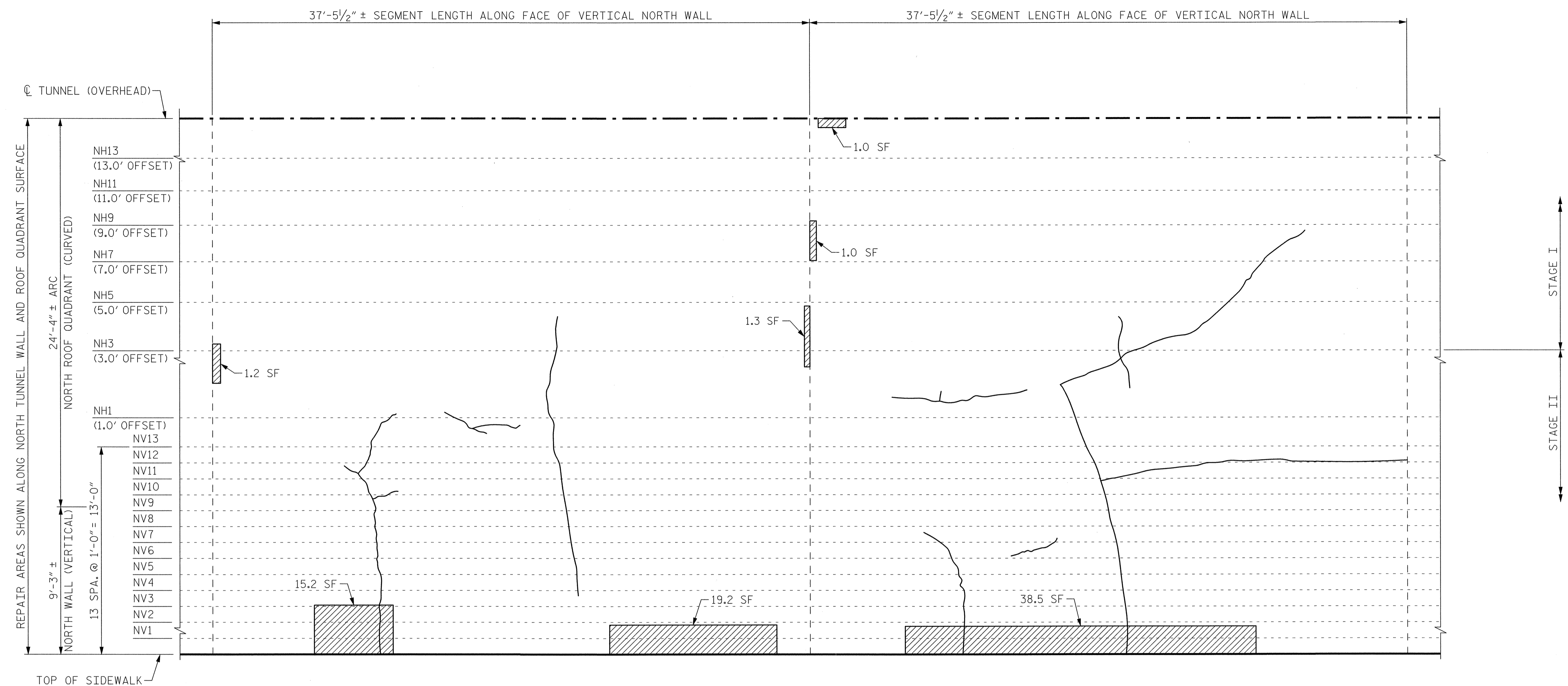
SEGMENT 14N SEGMENT 13N VIEW B-B: REPAIR SEGMENTS 13N & 14N TUNNEL SURFACE ELEVATION
