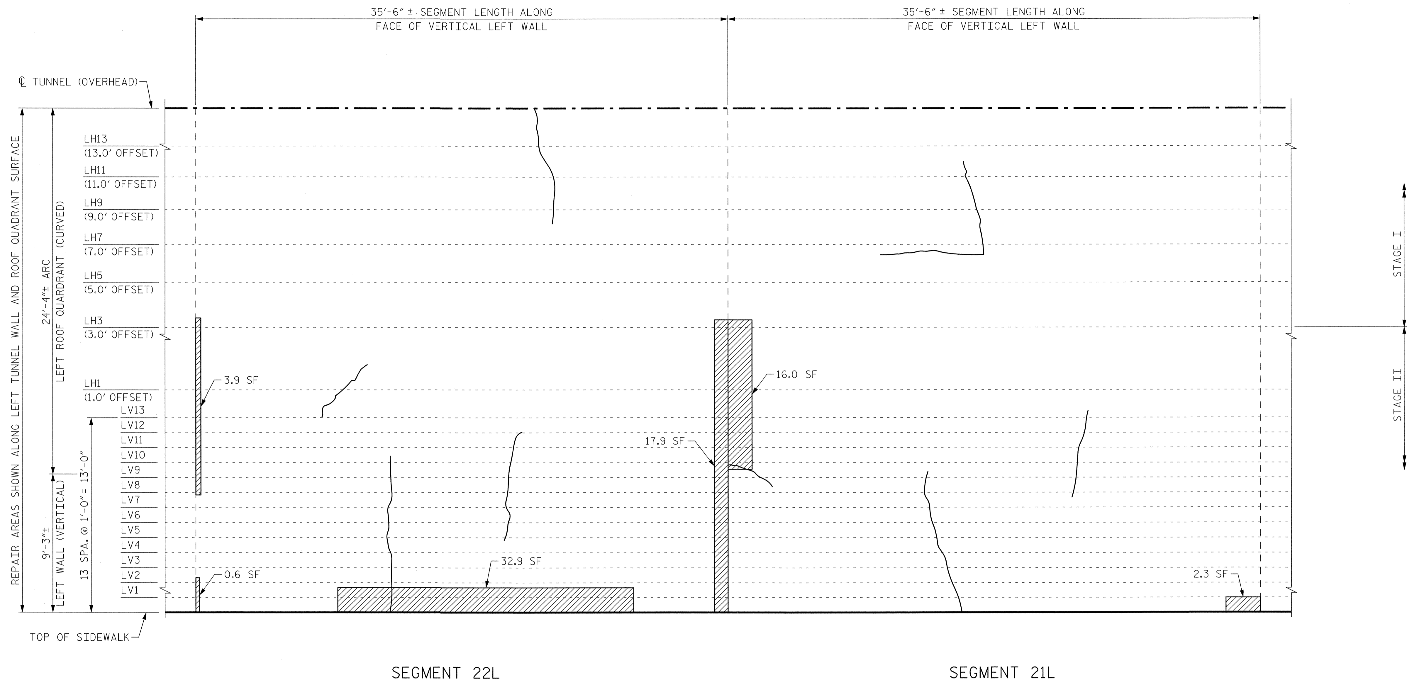
VIEW B-B: REPAIR SEGMENTS 21L & 22L TUNNEL SURFACE ELEVATION
