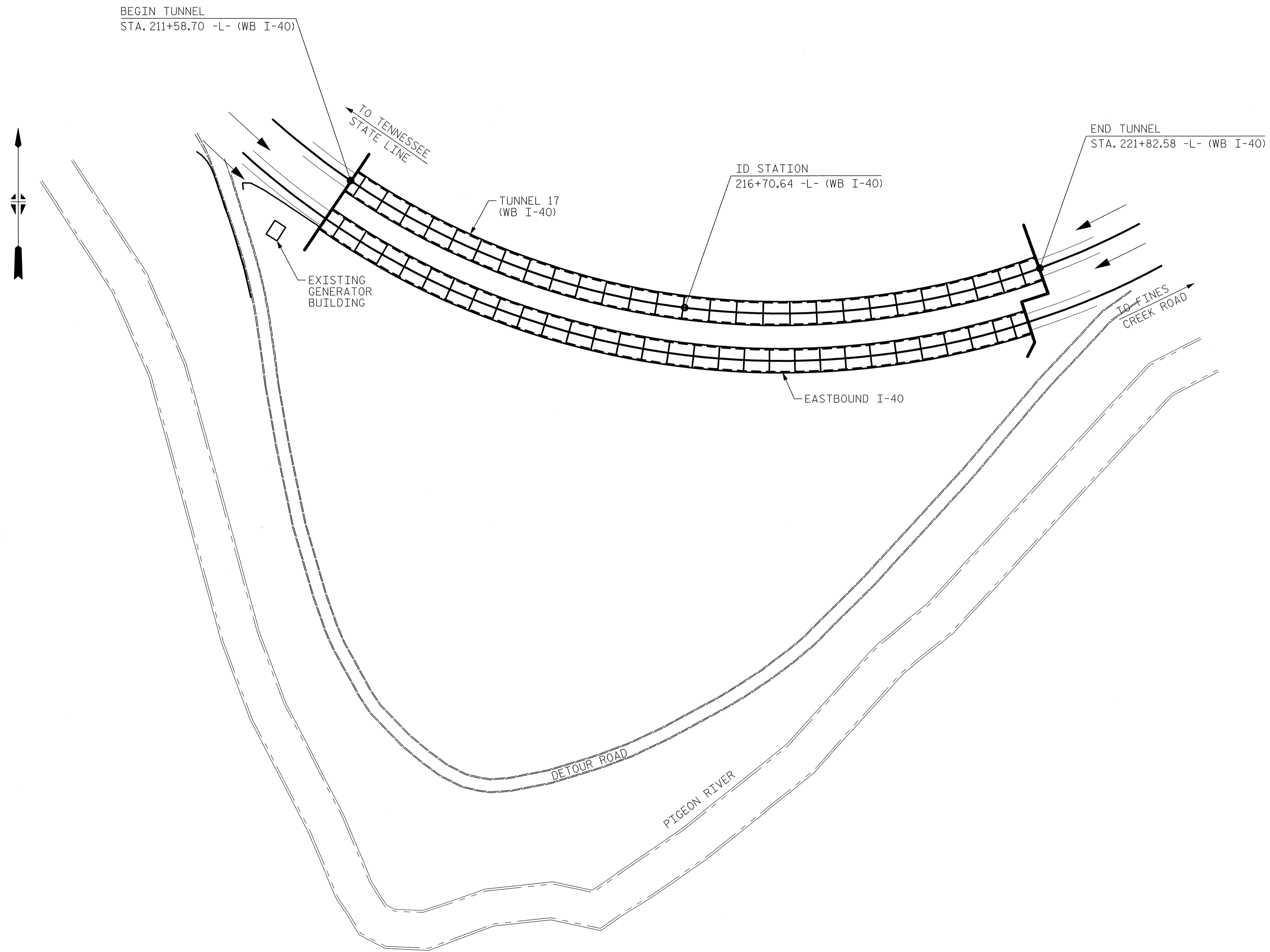
PLAN VIEW
