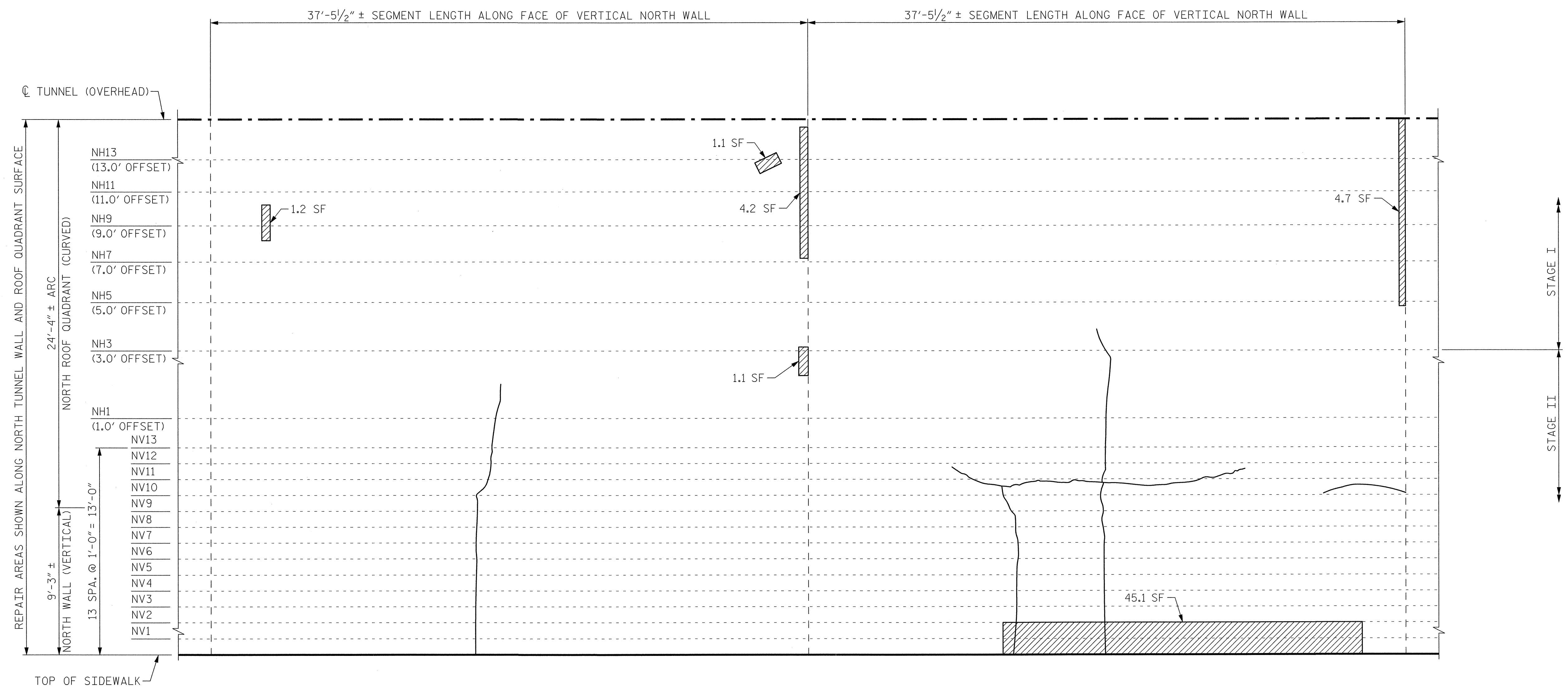
VIEW B-B: REPAIR SEGMENTS 23N & 24N TUNNEL SURFACE ELEVATION
