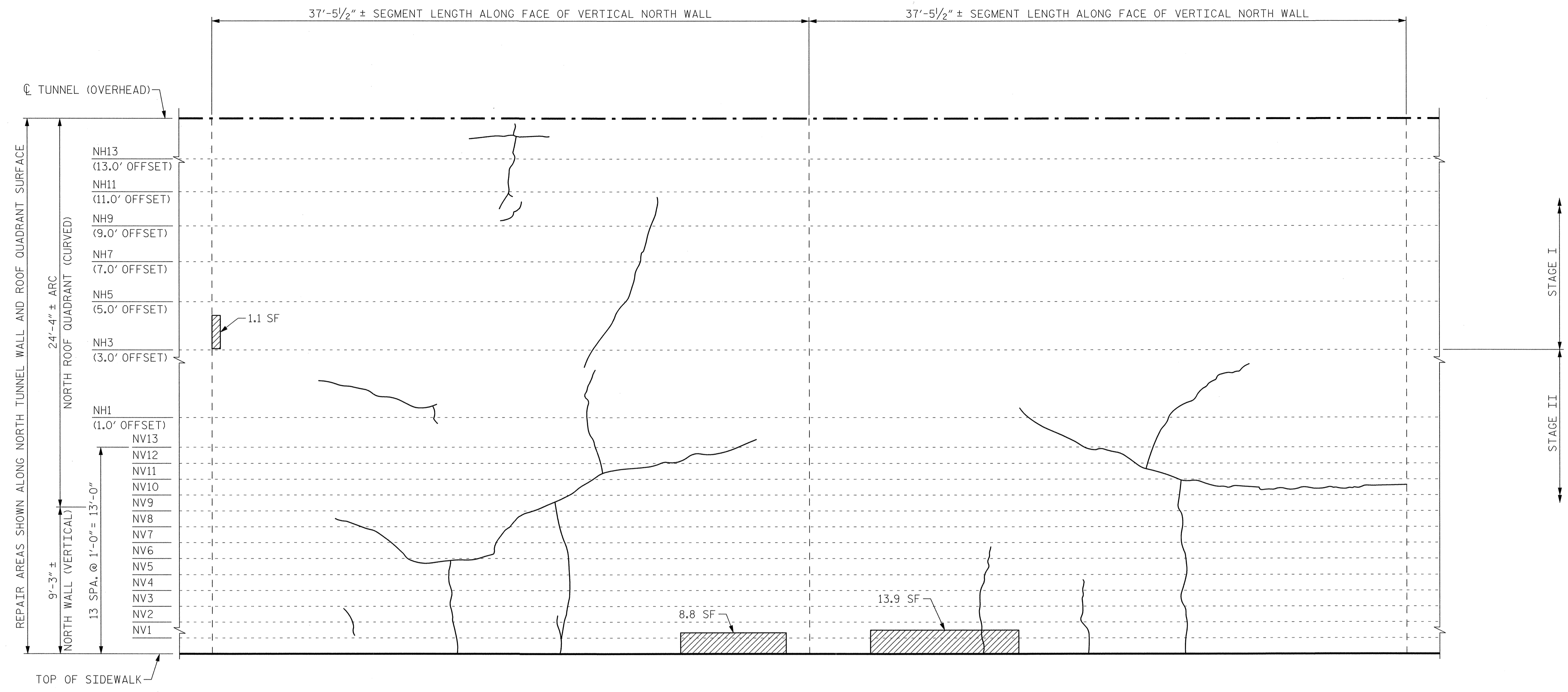
SEGMENT 6N SEGMENT 5N VIEW B-B: REPAIR SEGMENTS 5N & 6N TUNNEL SURFACE ELEVATION
