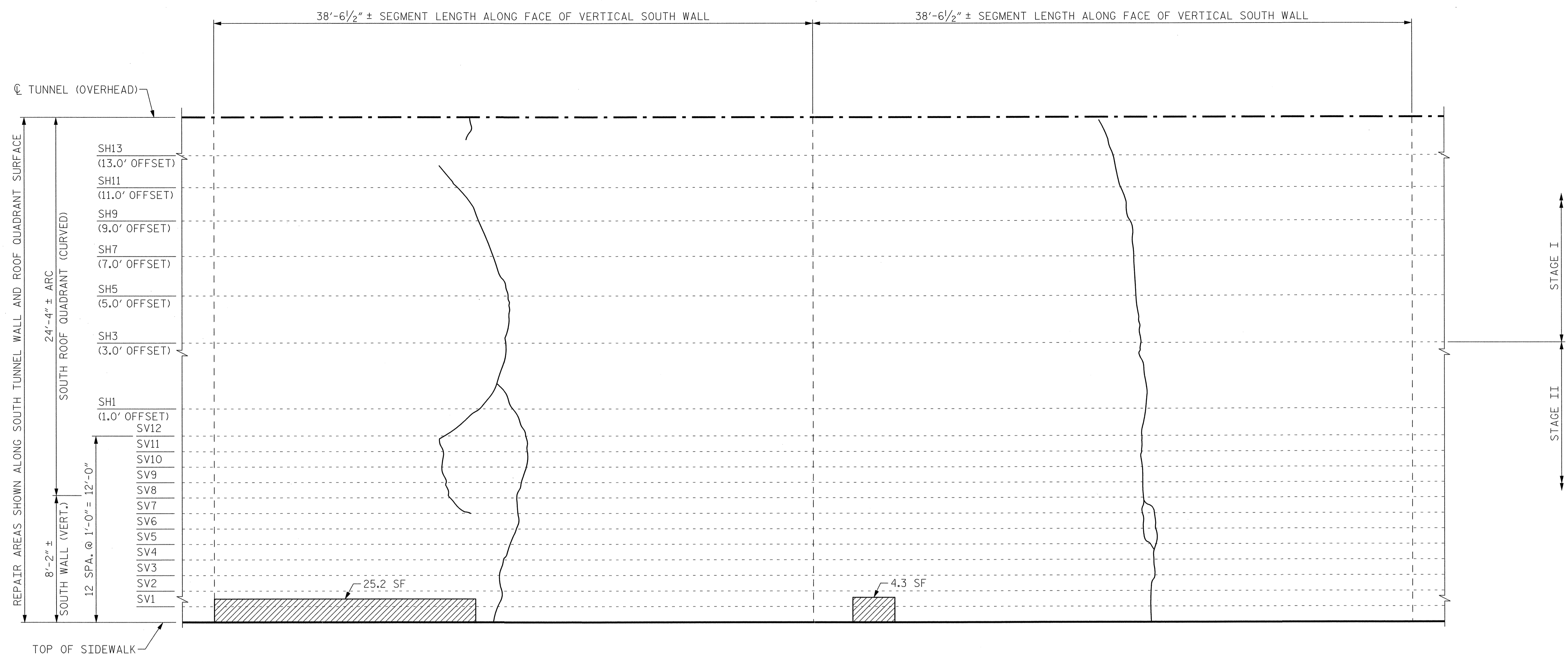
VIEW B-B: REPAIR SEGMENTS 7S & 8S TUNNEL SURFACE ELEVATION
