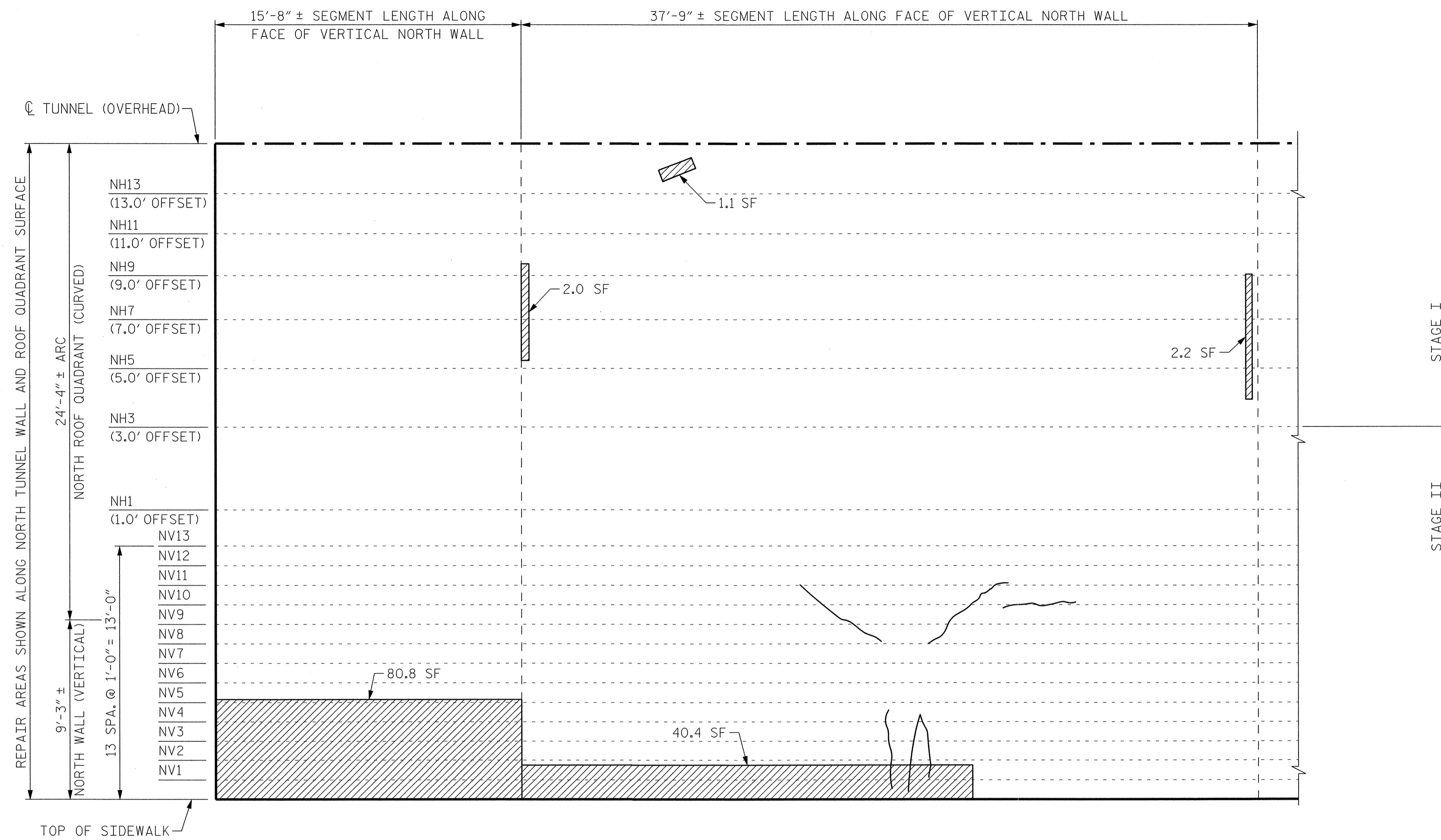
VIEW B-B: REPAIR SEGMENTS 27N & 28N TUNNEL SURFACE ELEVATION
