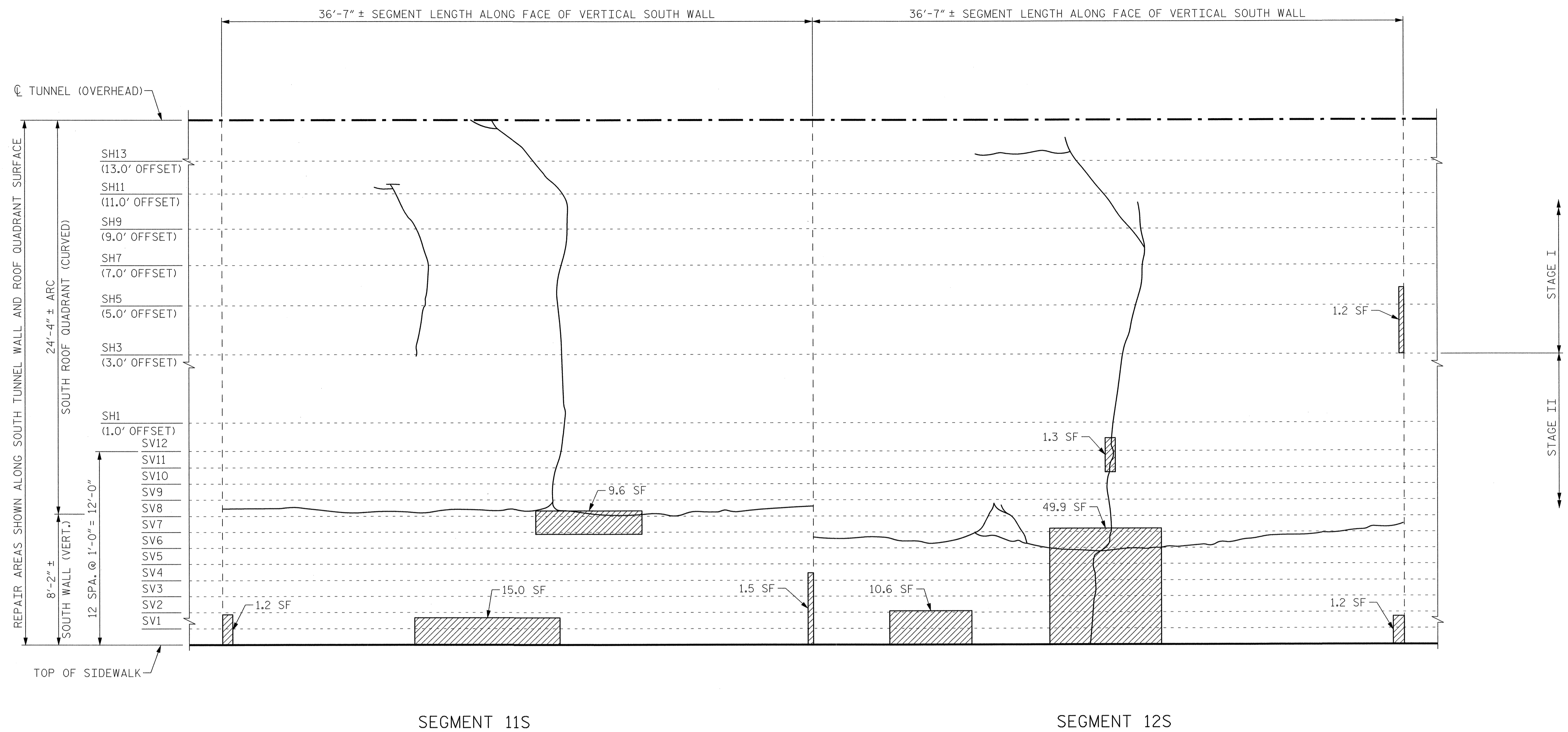
VIEW B-B: REPAIR SEGMENTS 11S & 12S TUNNEL SURFACE ELEVATION
