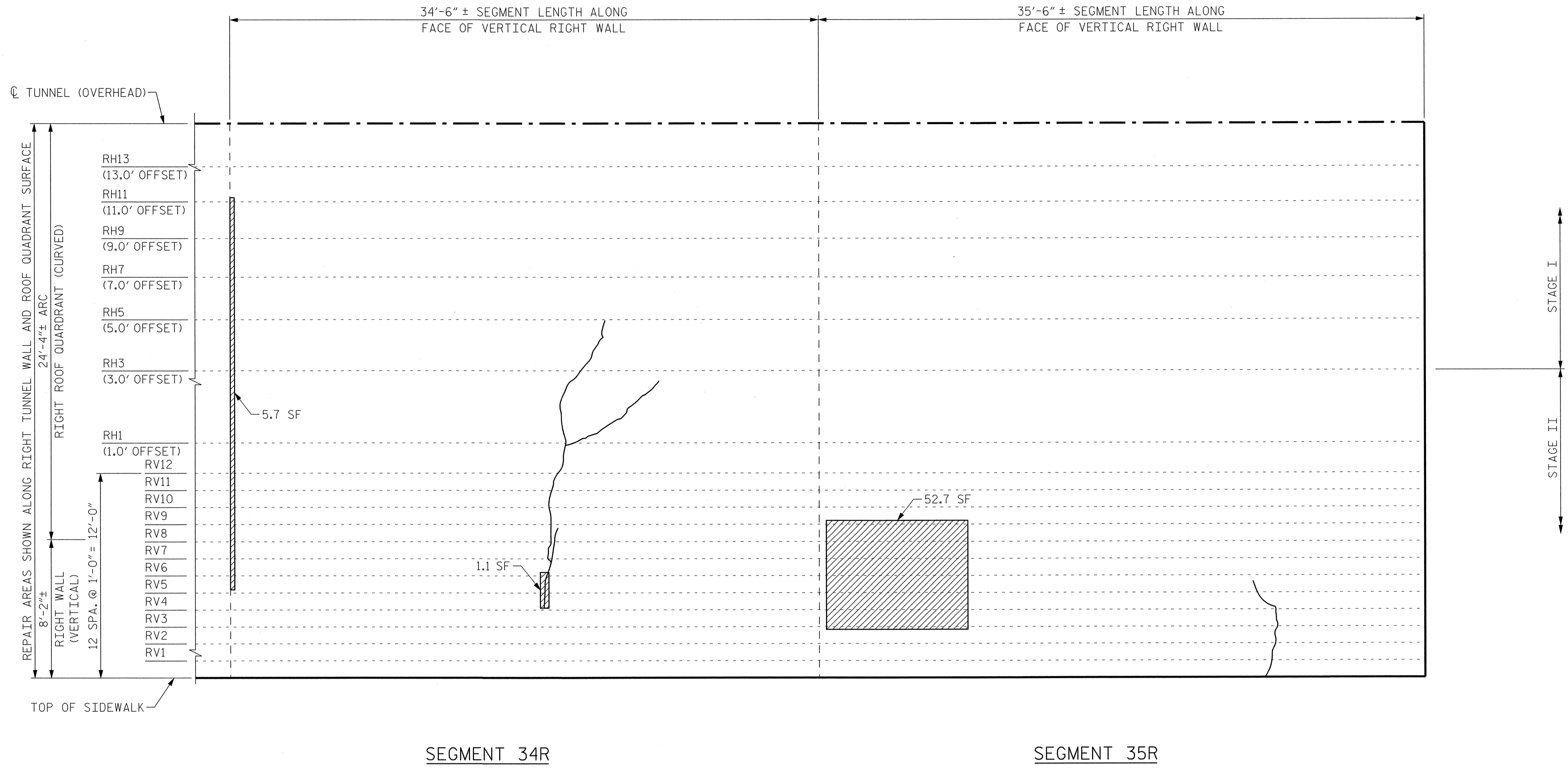
VIEW B-B: REPAIR SEGMENTS 34R & 35R TUNNEL SURFACE ELEVATION
