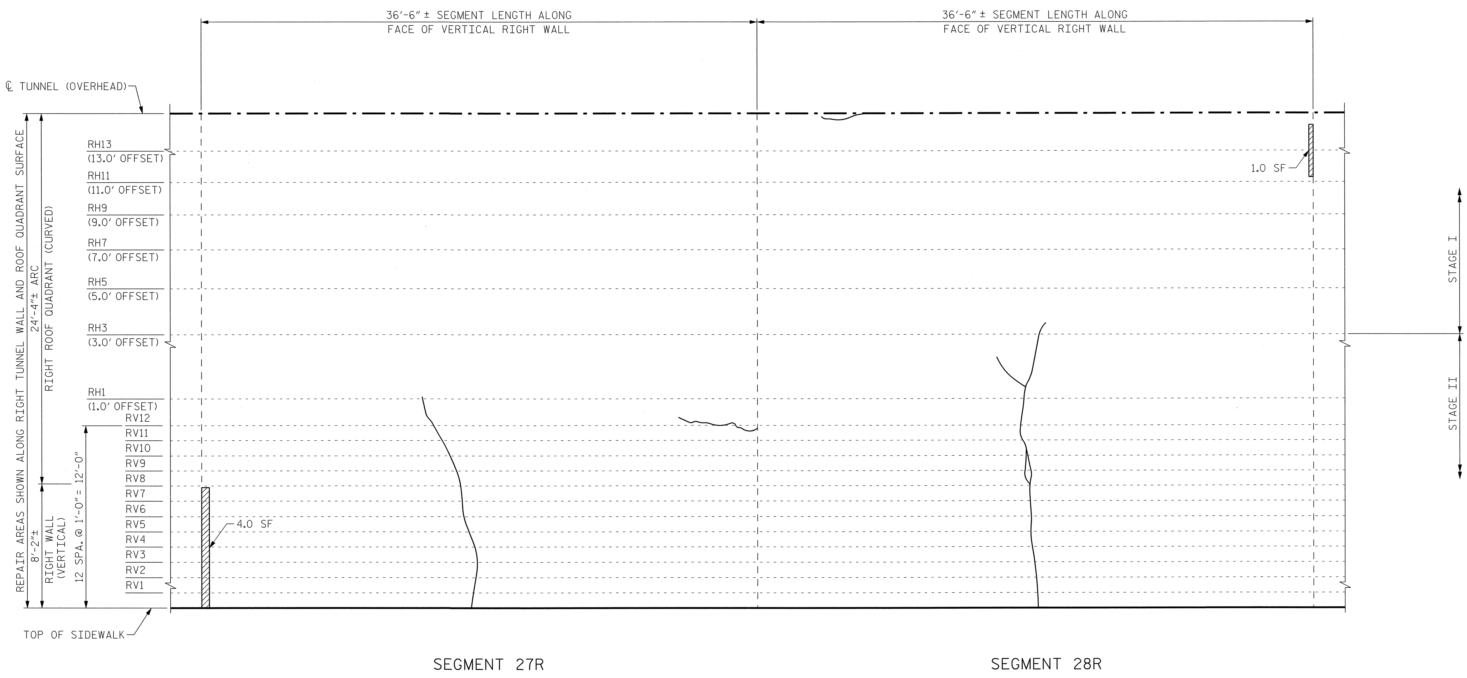
VIEW B-B: REPAIR SEGMENTS 27R & 28R TUNNEL SURFACE ELEVATION
