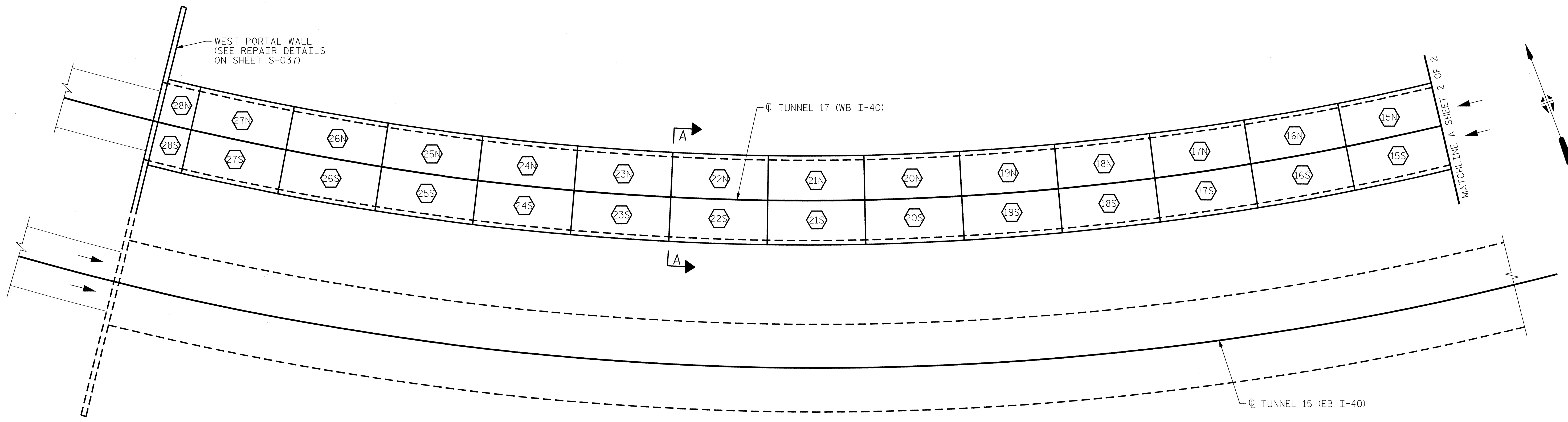
PARTIAL PLAN OF REPAIR SEGMENTS - TUNNEL 17
