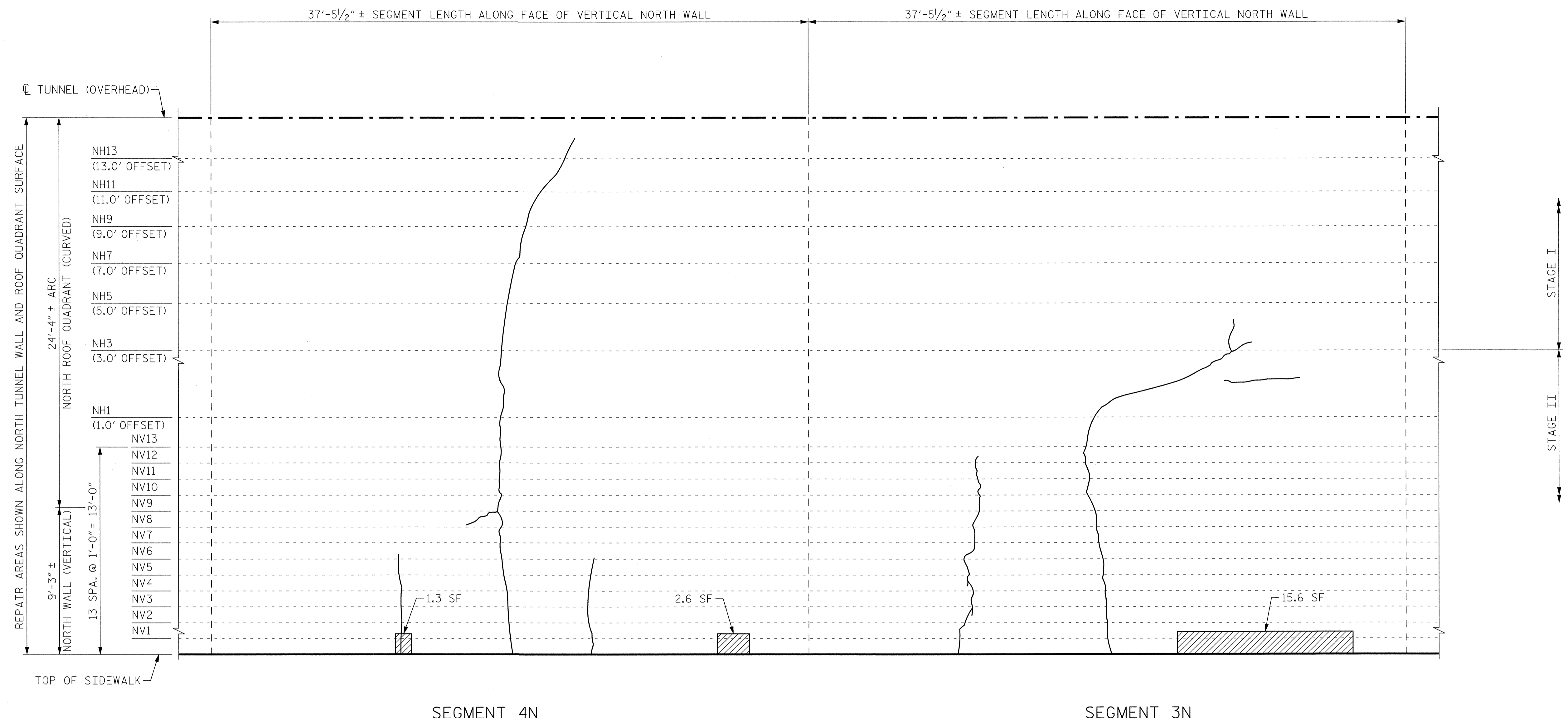
VIEW B-B: REPAIR SEGMENTS 3N & 4N TUNNEL SURFACE ELEVATION
