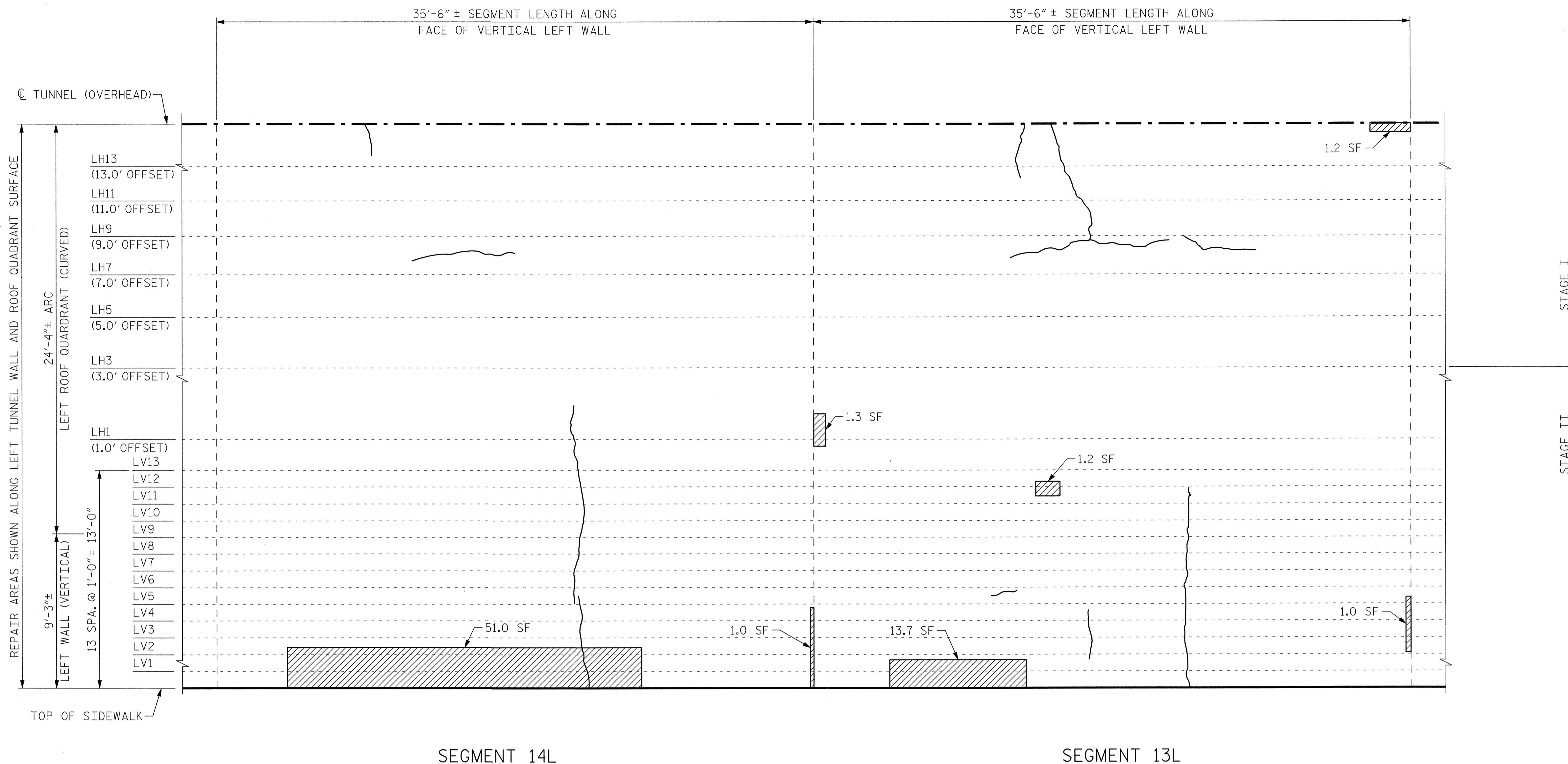
VIEW B-B: REPAIR SEGMENTS 13L & 14L TUNNEL SURFACE ELEVATION
