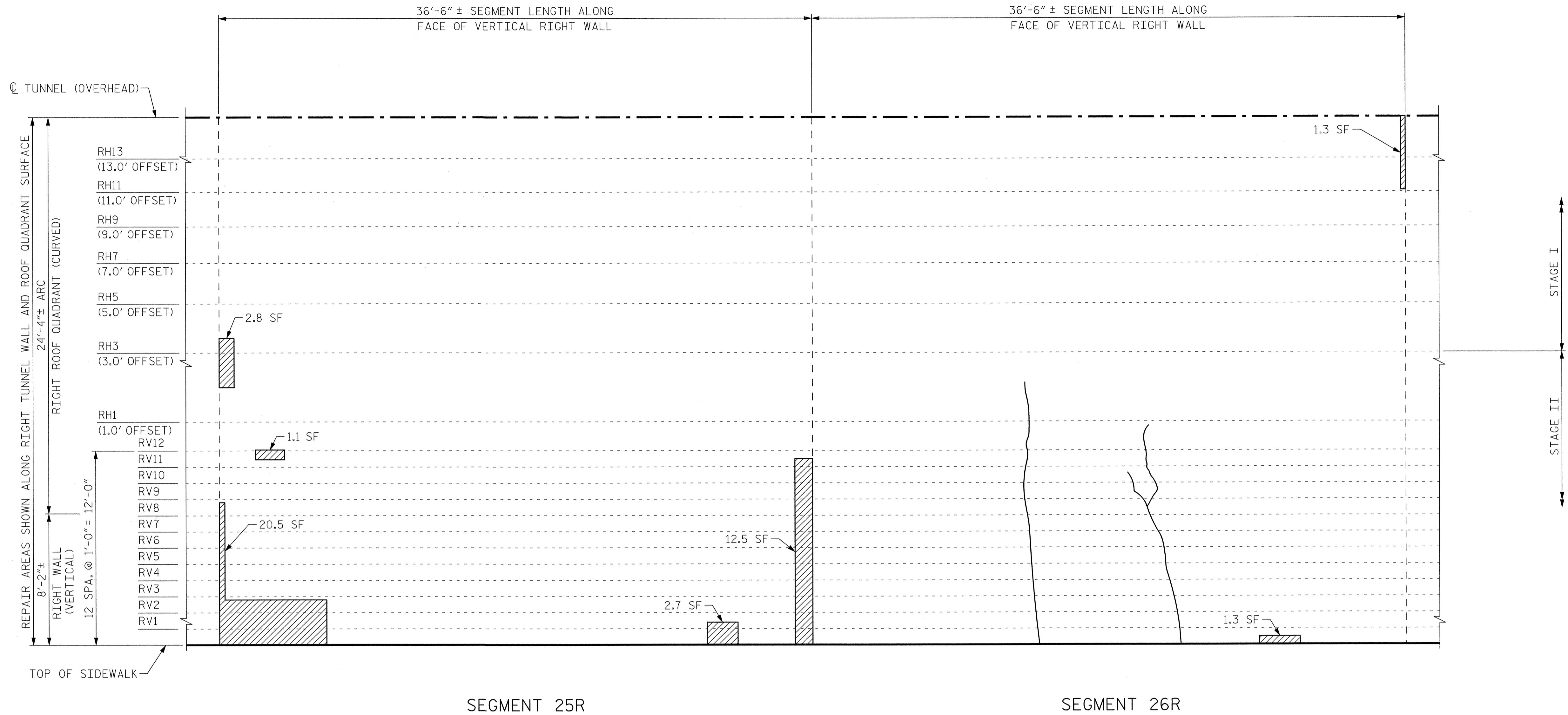
VIEW B-B: REPAIR SEGMENTS 25R & 26R TUNNEL SURFACE ELEVATION
