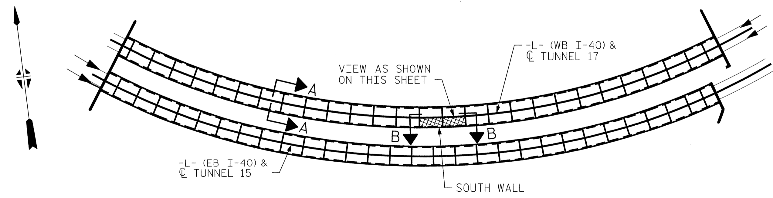
KEY PLAN
