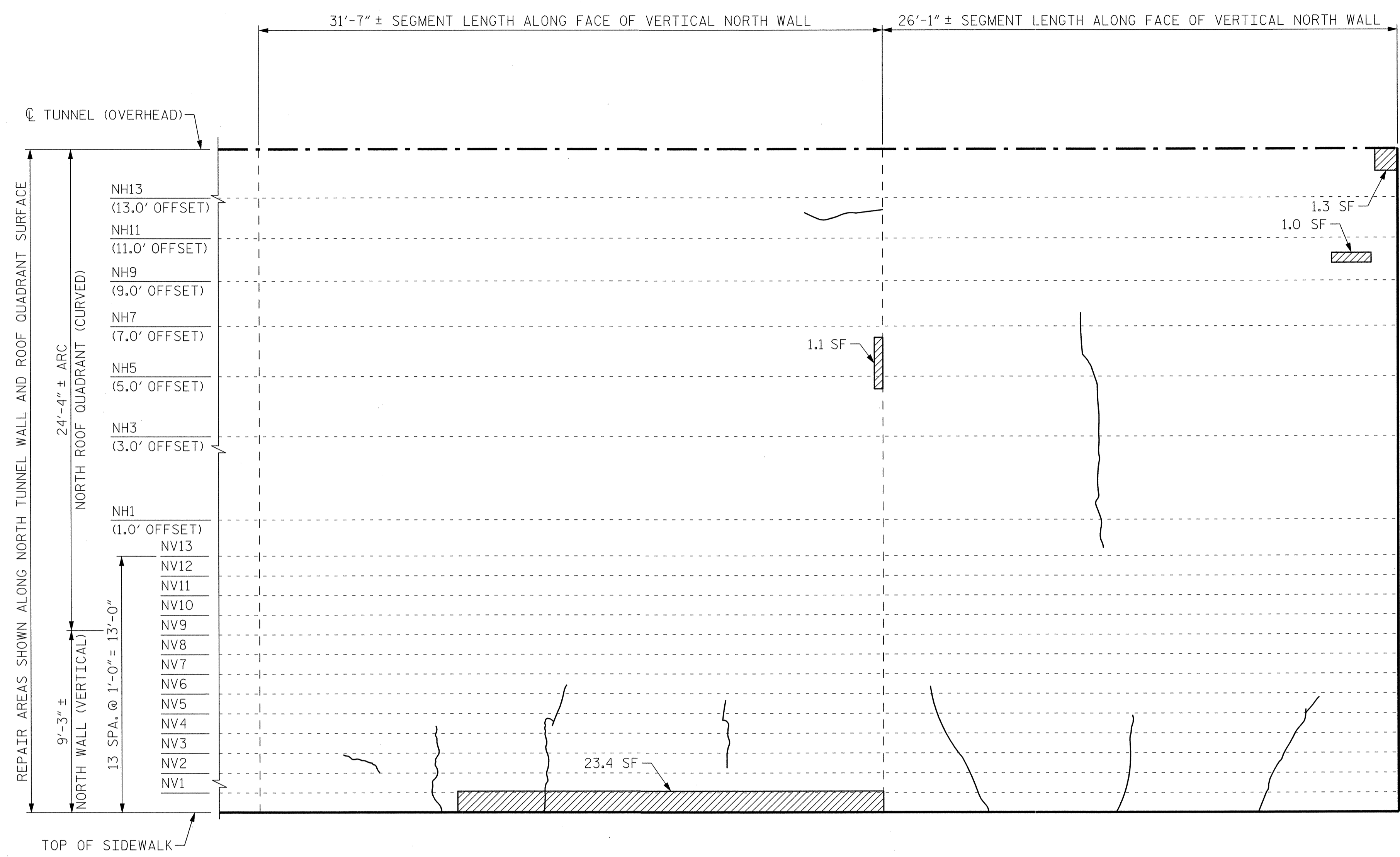
SEGMENT 2N SEGMENT 1N VIEW B-B: REPAIR SEGMENTS 1N & 2N TUNNEL SURFACE ELEVATION
