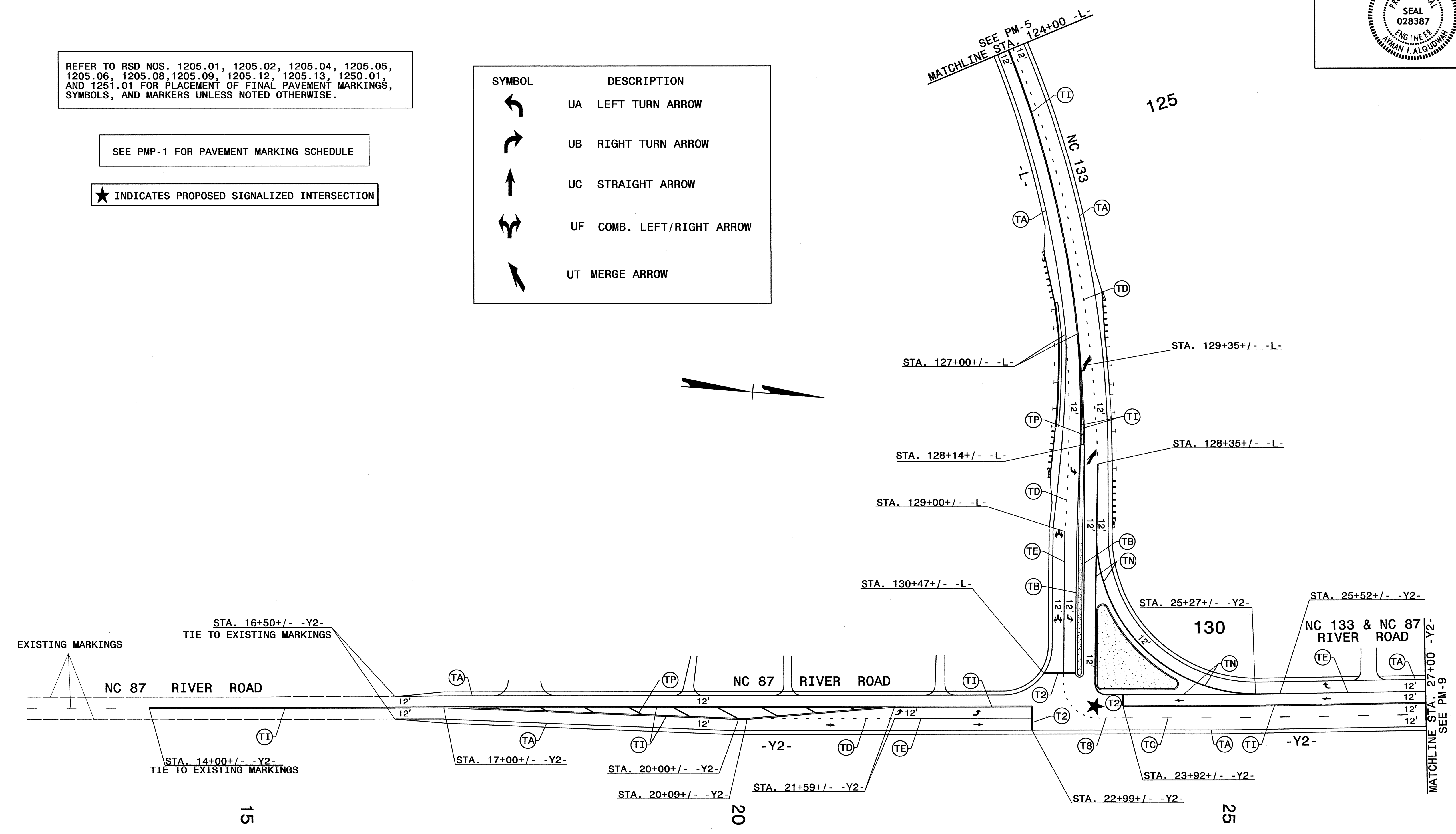
PAVEMENT MARKING DETAIL
