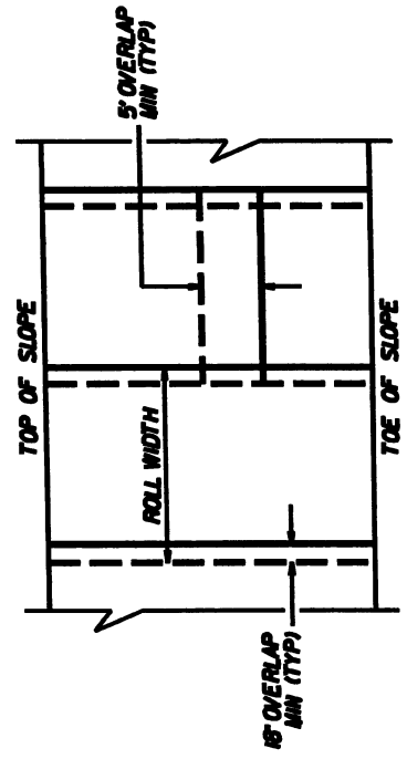
FABRIC OVERLAP DETAIL (PLAN VIEW)
