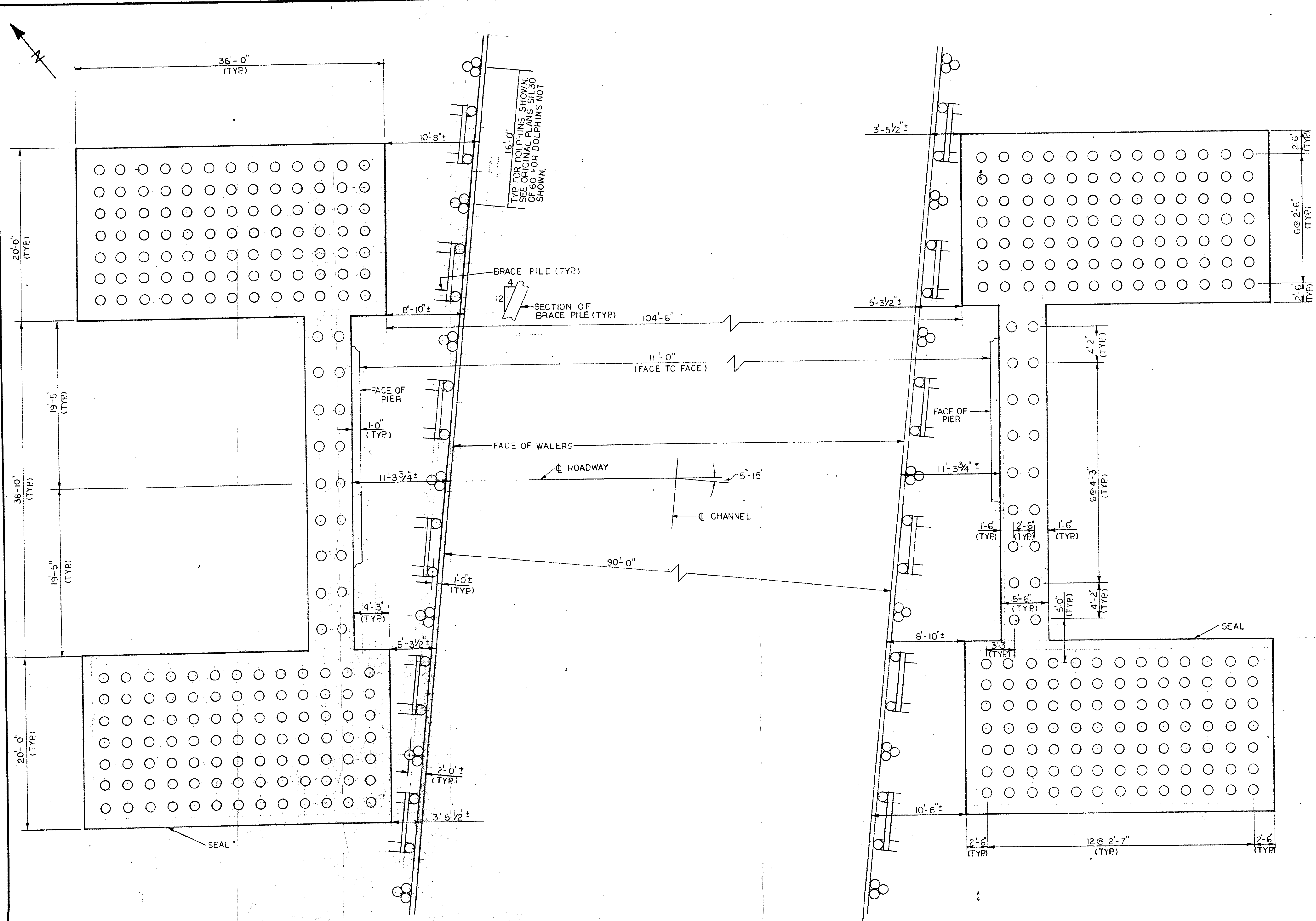
PLAN SCALE: 3/16" = 1' 0"
