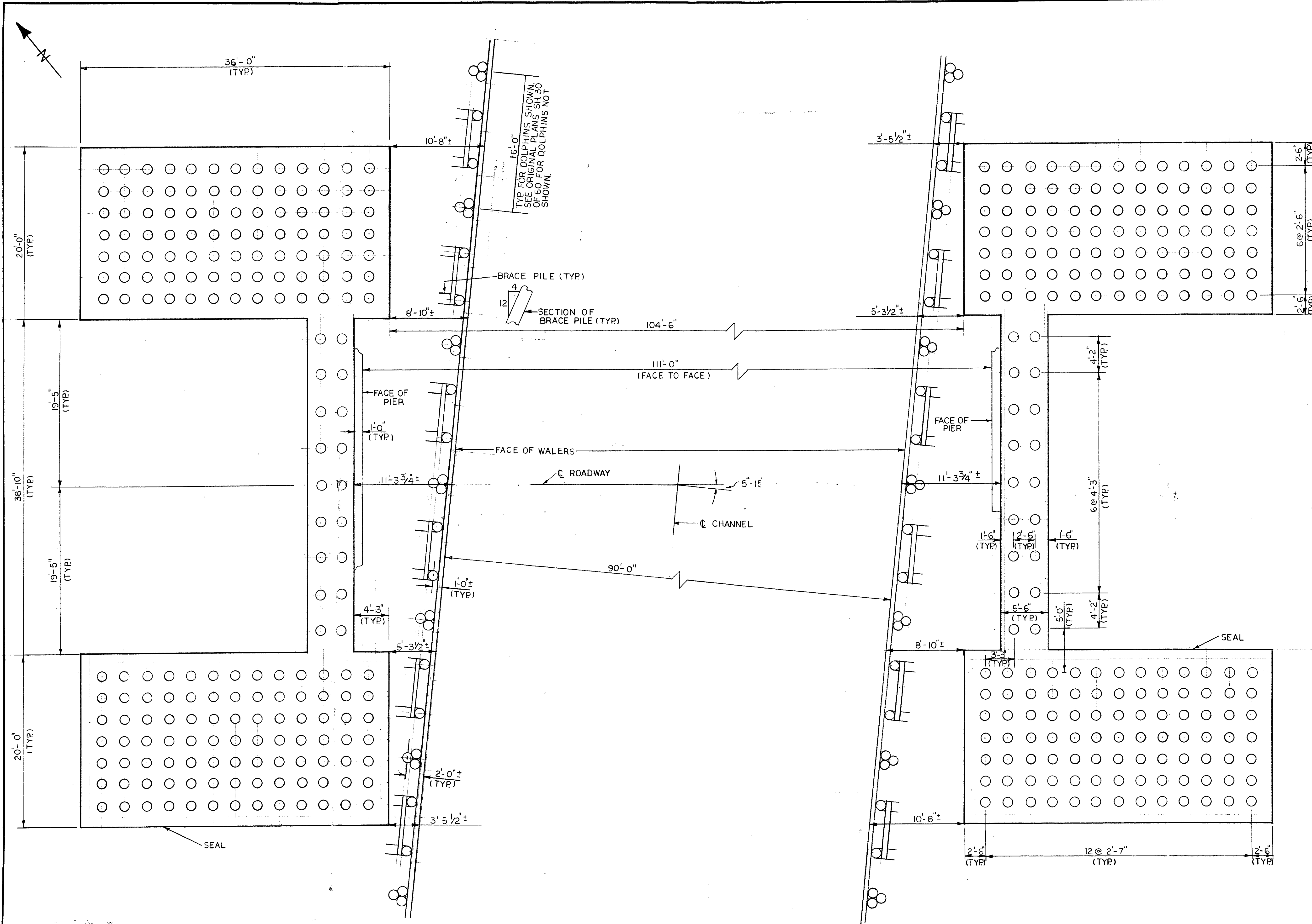
PLAN SCALE: 3/16"=1' 0"
