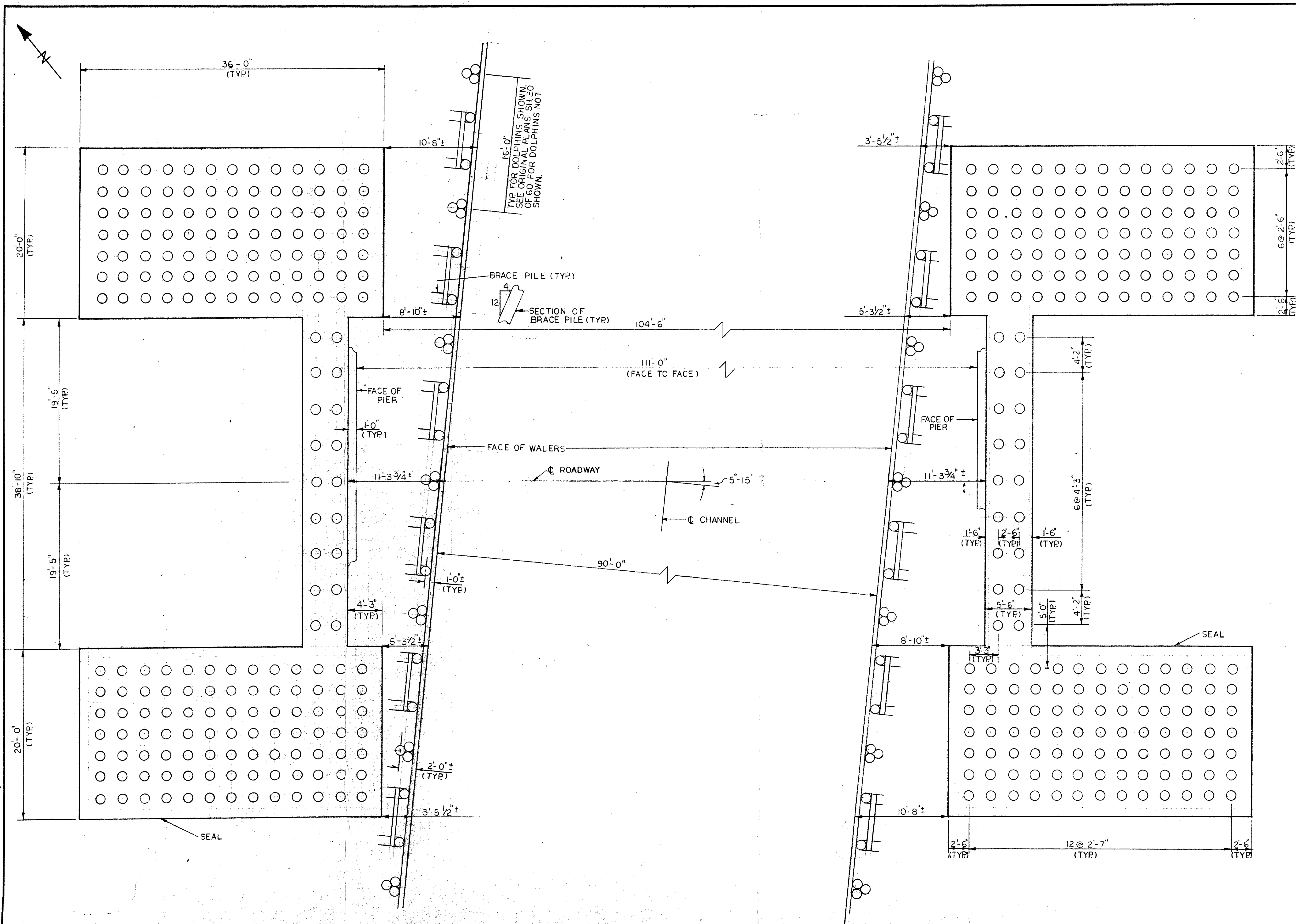
PLAN SCALE: 3/16"=1' 0"
