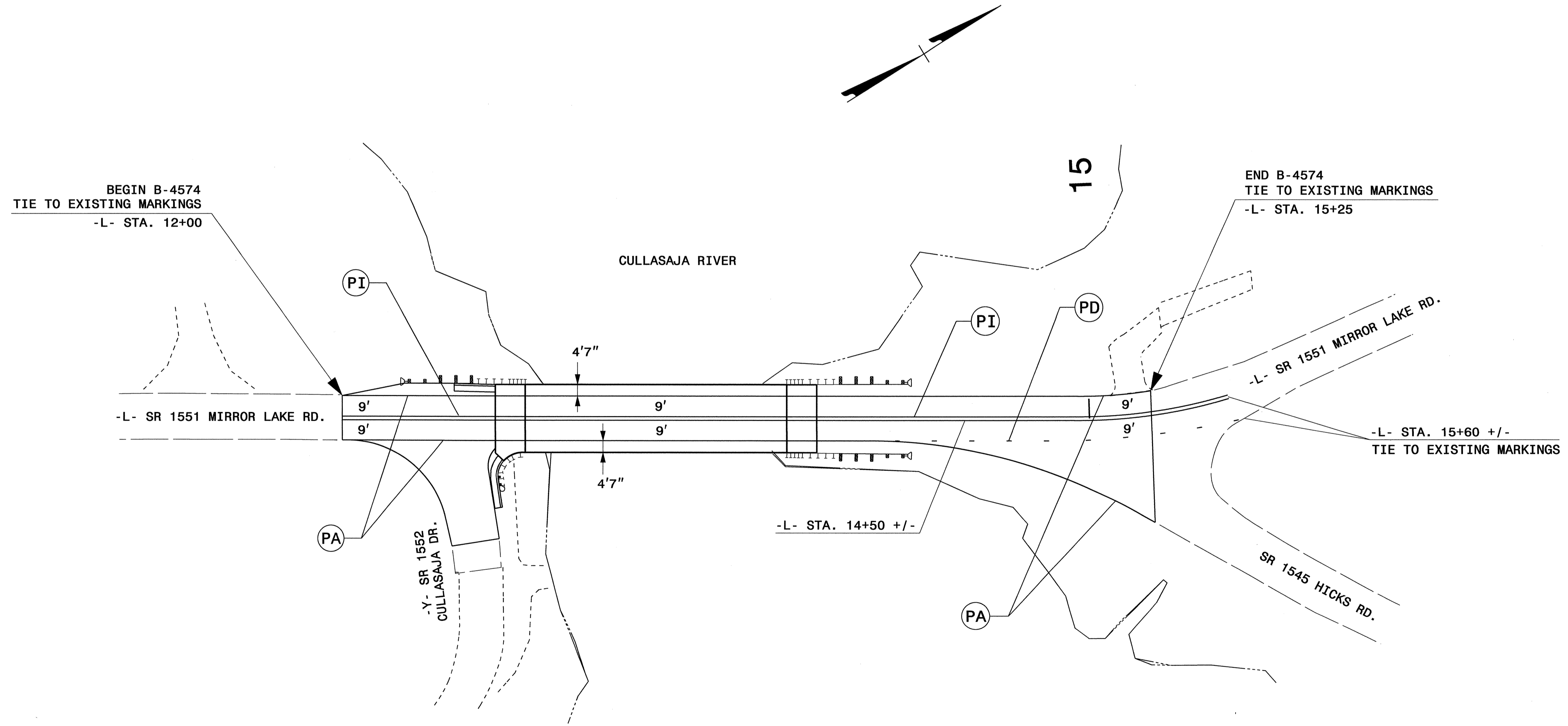
PAVEMENT MARKING SCHEDULE AND PAVEMENT MARKING DETAIL
