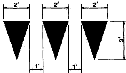
SPECIAL DETAIL FOR YIELD LINE
