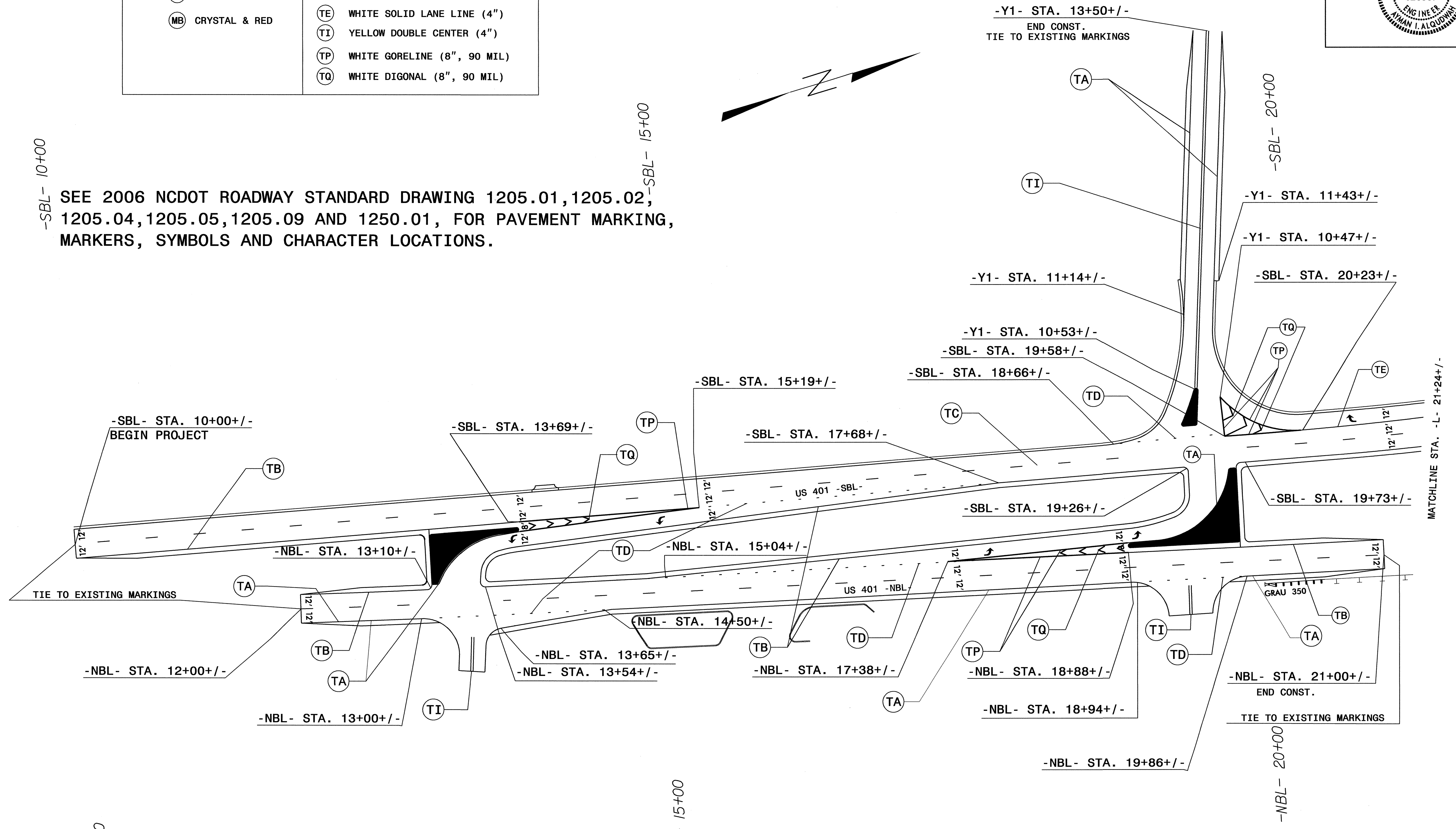
FINAL PAVEMENT MARKING DETAIL
