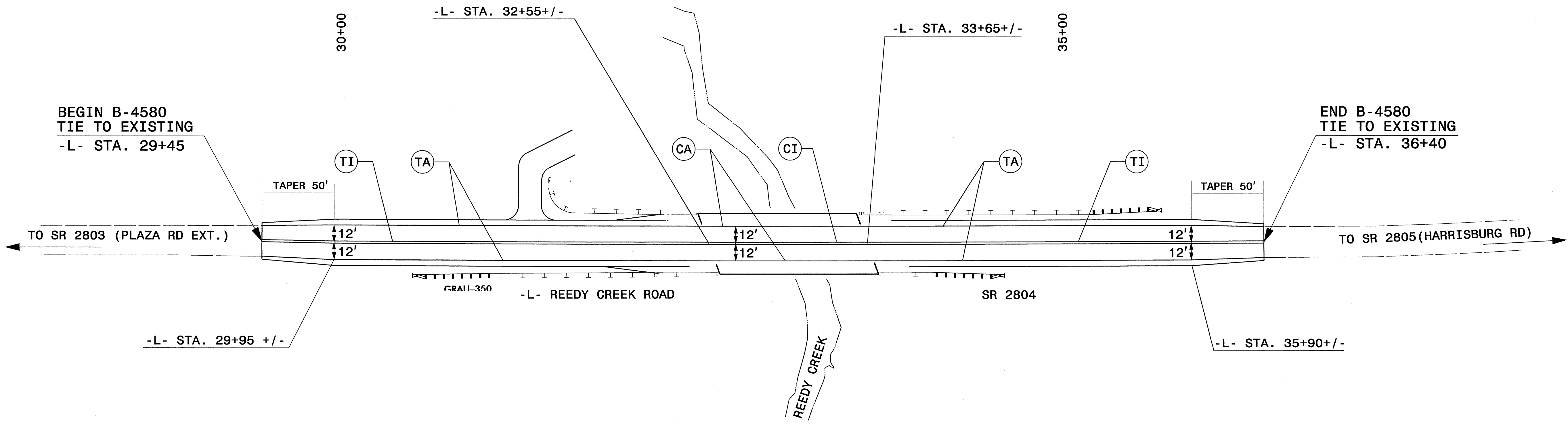
PAVEMENT MARKING SCHEDULE AND PAVEMENT MARKING DETAIL
