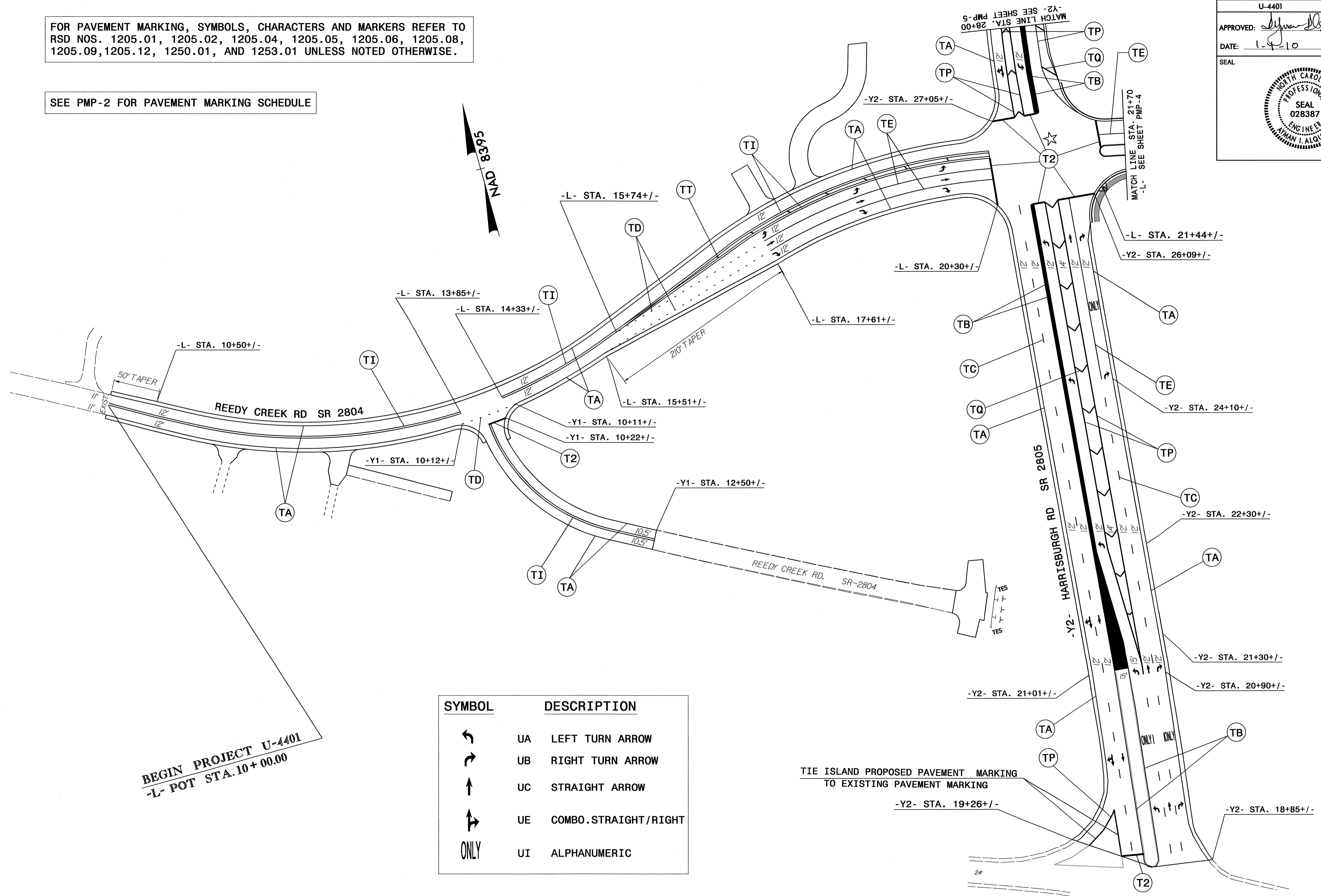
FINAL PAVEMENT MARKING DETAIL
