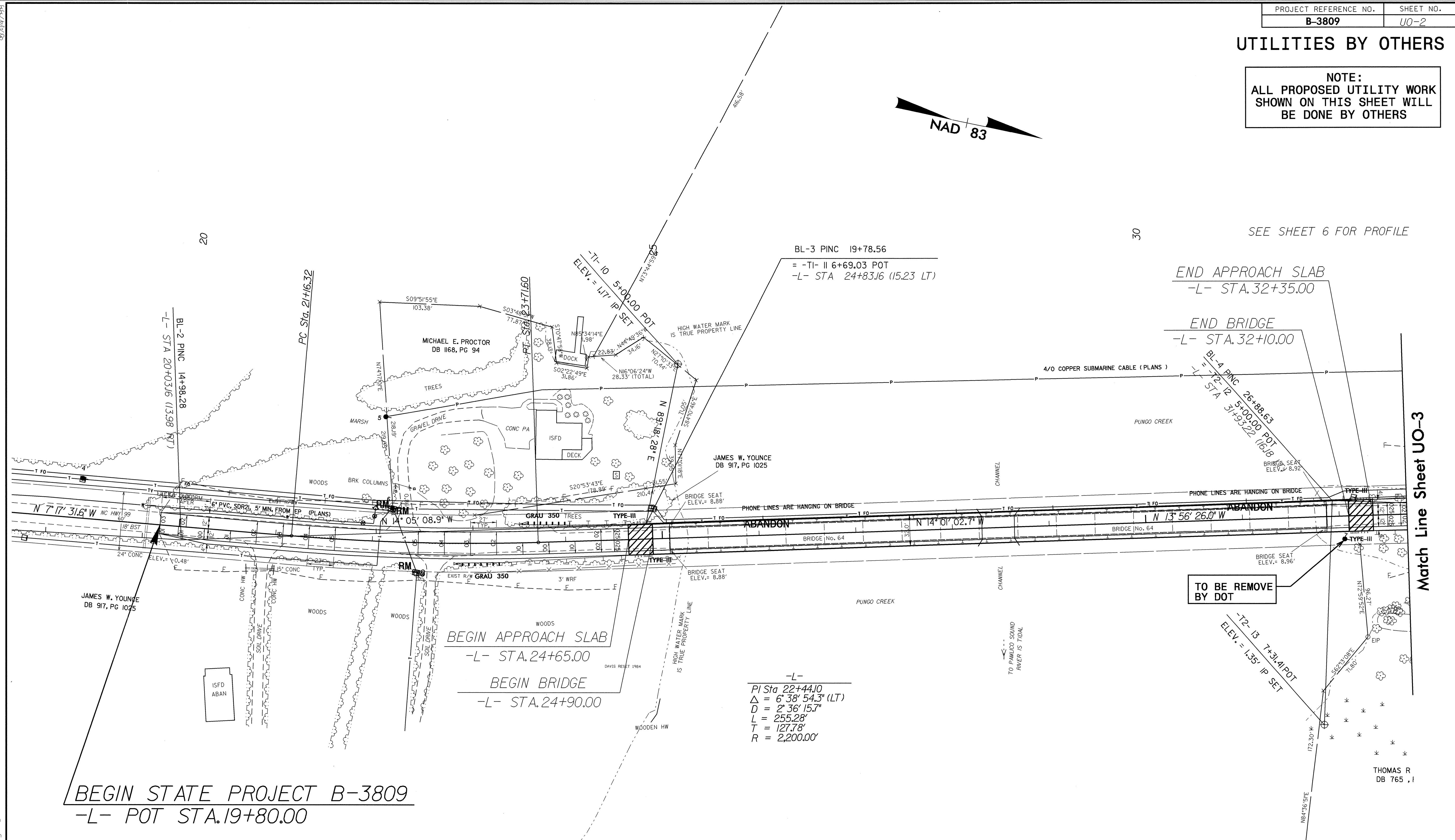
SKETCH SHOWING BRIDGE /PAVEMENT RELATIONSHIP
