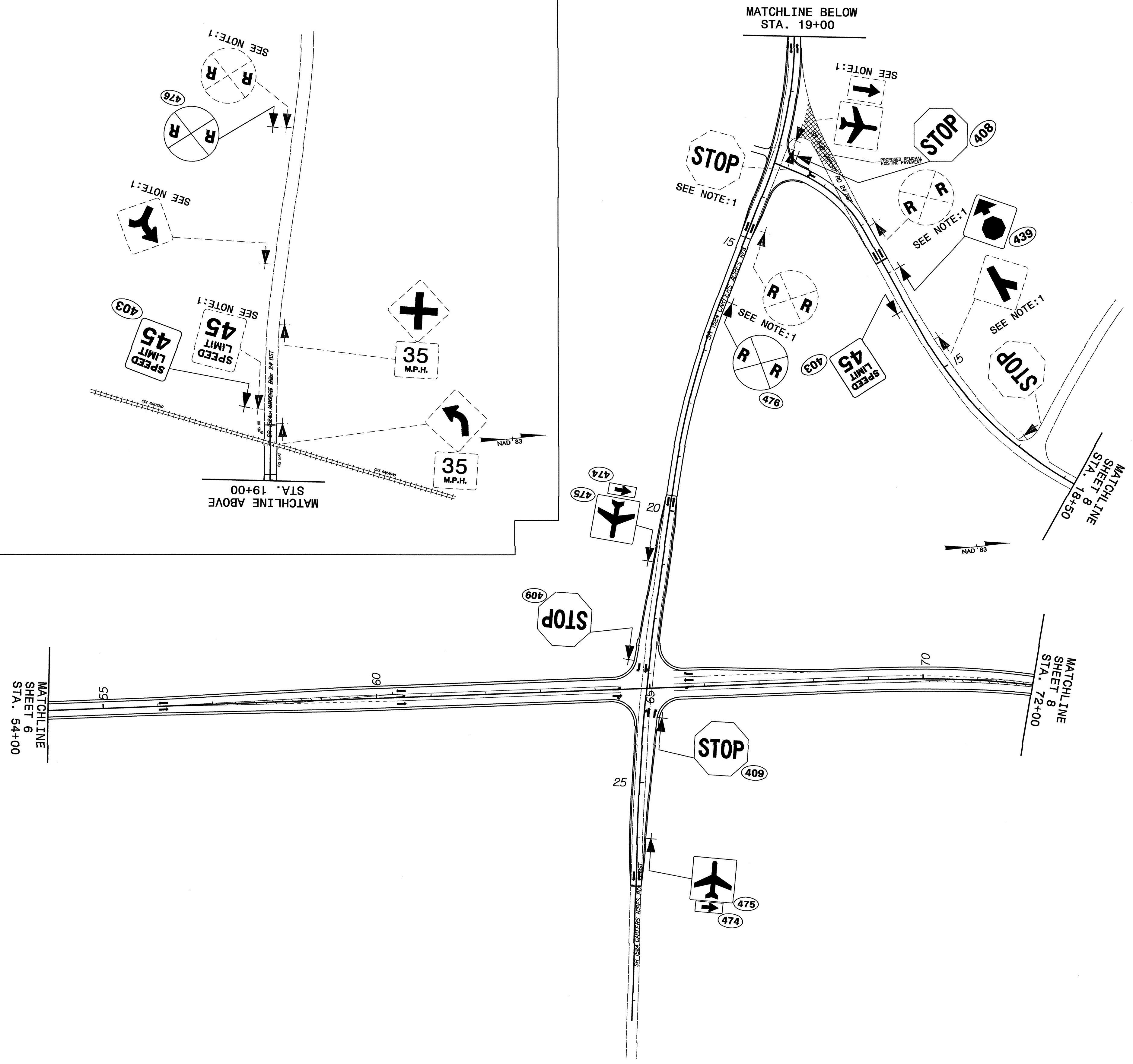
EXISTING AND PROPOSED SIGNS STA. 54+00 TO STA. 72+00
