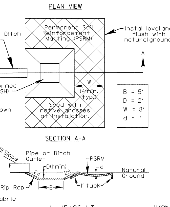
DETAIL A PREFORMED SCOUR HOLE
