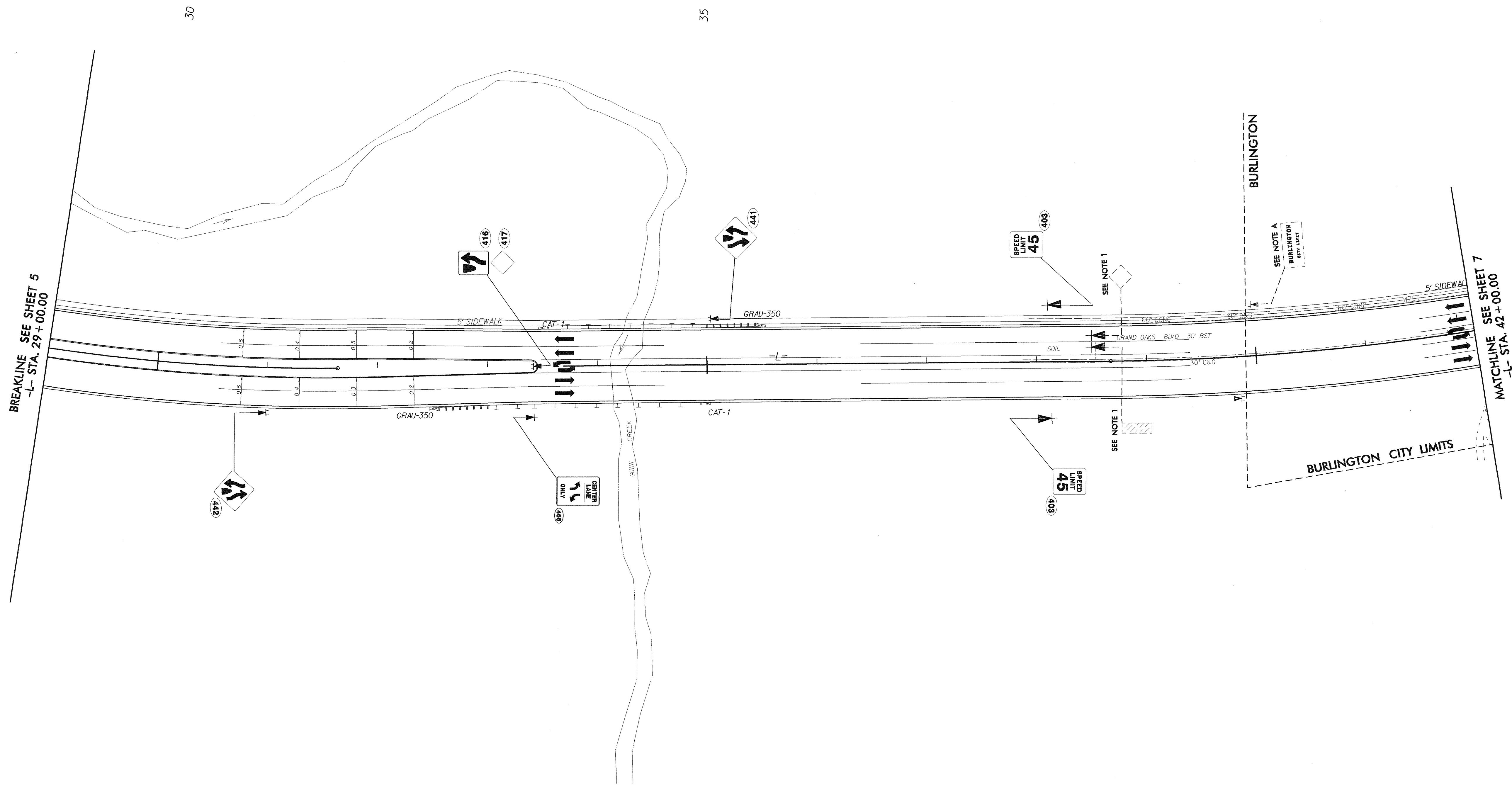
EXISTING and PROPOSED SIGNS GRAND OAKS BLVD
