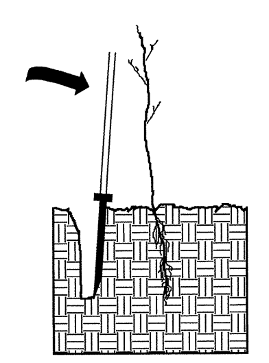
5. Push handle forward firming soil at top.
