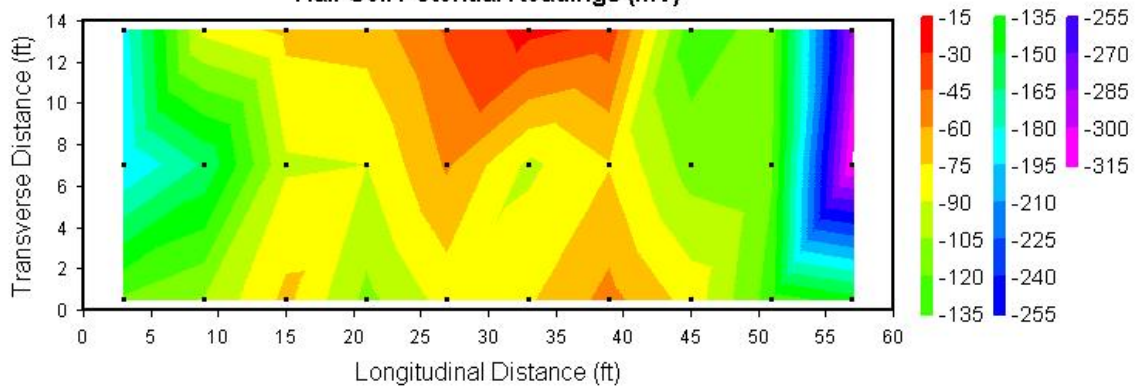
Span 175-176; North Bound Lane Half Cell Potential Readings (mV)
