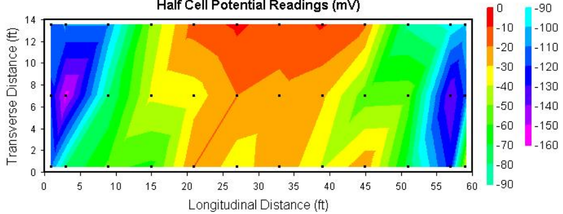
Span 87-88; North Bound Lane Half Cell Potential Readings (mV)
