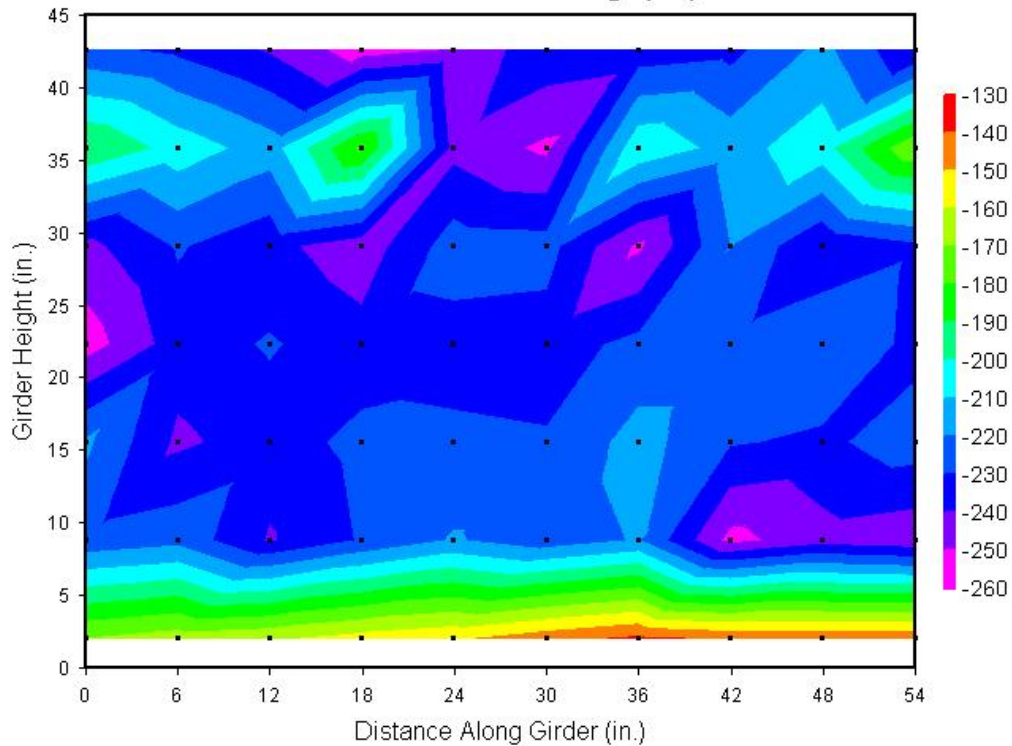
Span 160-161 Girder #3, East Elevation, Midspan Half Cell Potential Readings (mV)
