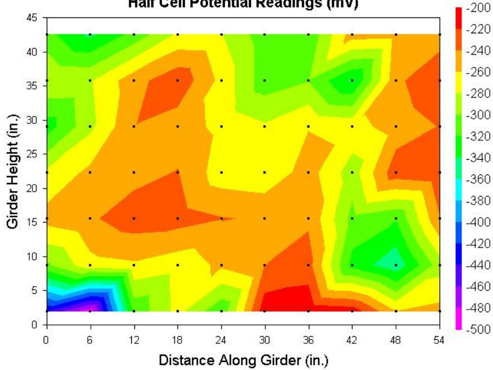
Span 148-149 Girder #3, East Elevation, Midspan Half Cell Potential Readings (mV)
