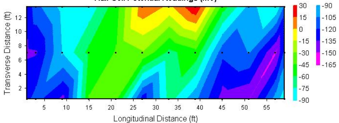
Span 92-93; North Bound Lane Half Cell Potential Readings (mV)
