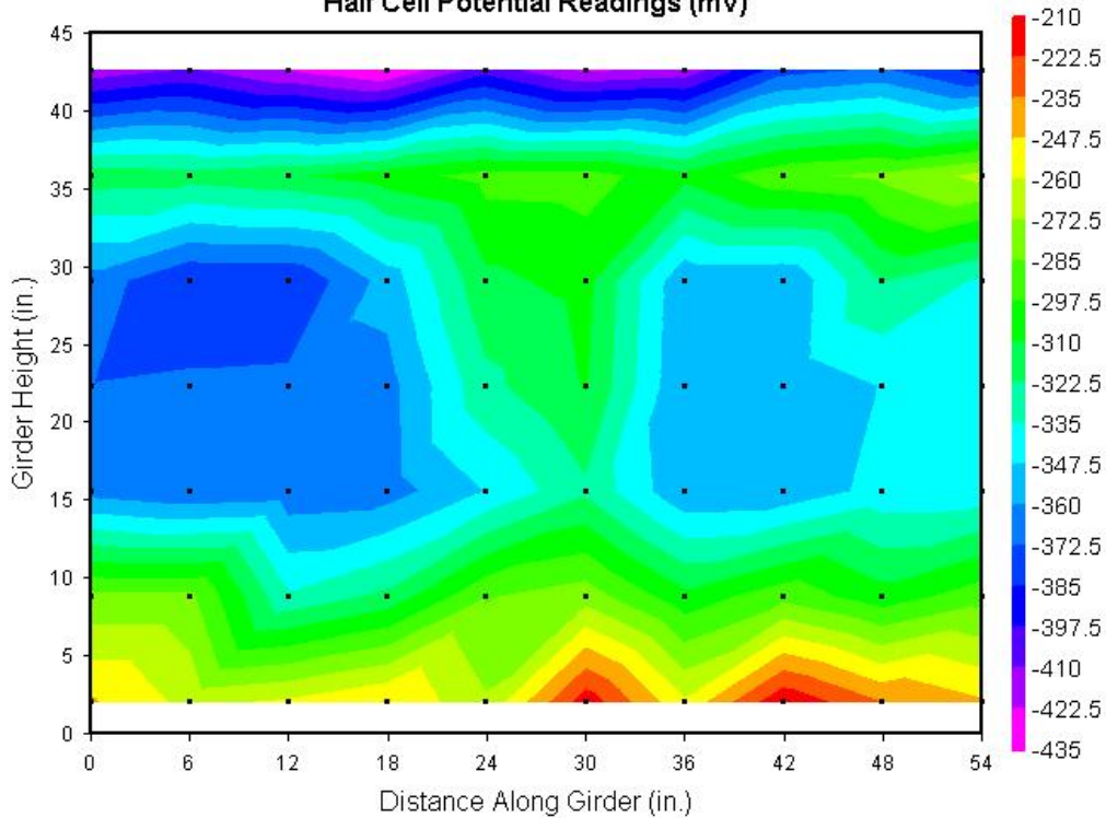
Span 149-150 Girder #4, East Elevation - Midspan Half Cell Potential Readings (mV)
