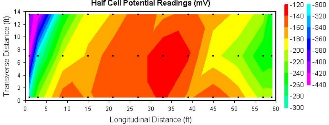
Span 116-117; North Bound Lane Half Cell Potential Readings (mV)
