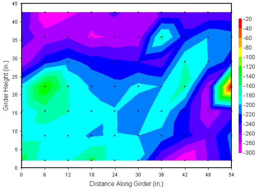
Span 160-161 Girder #1, West Elevation, North End Half Cell Potential Readings (mV)
