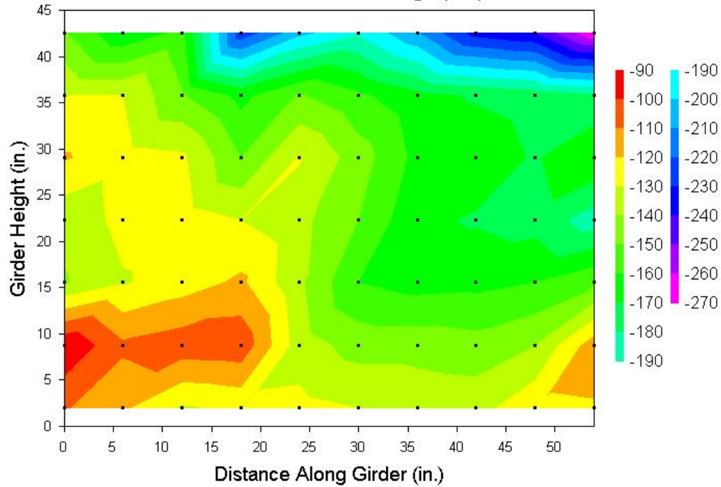
Span 149-150, Girder #1, West Elevation, North End Half Cell Potential Readings (mV)
