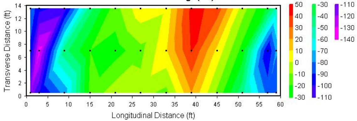
Span 87-88; North Bound Lane Half Cell Potential Readings (mV)
