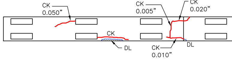
Top of Bent Cap
