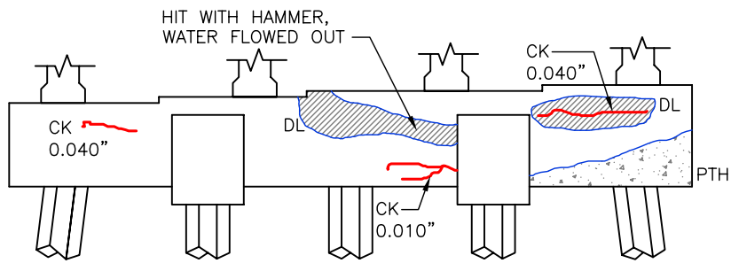
North Elevation
