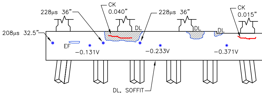
North Elevation
