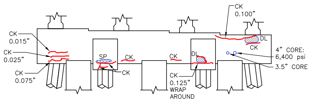
South Elevation
