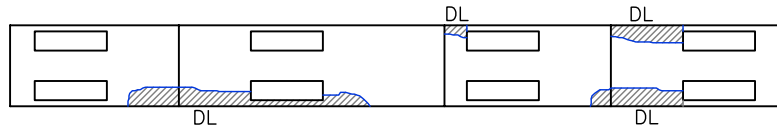
← West Top of Bent Cap East →
