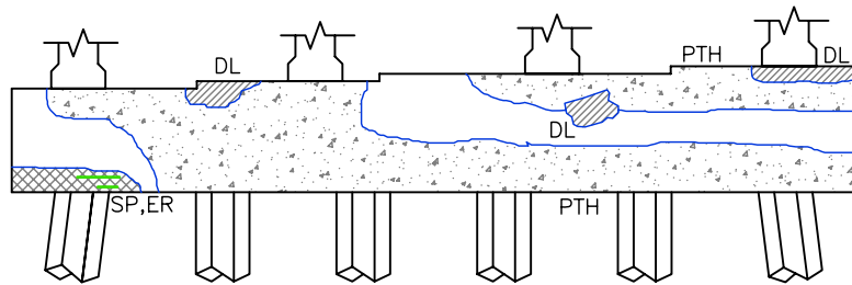
North Elevation
