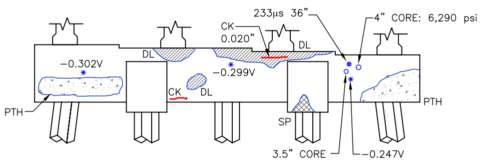
South Elevation
