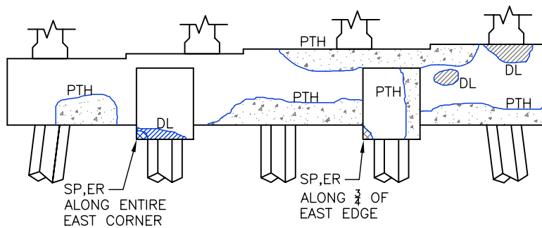
North Elevation
