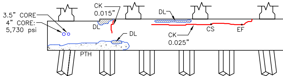
North Elevation
