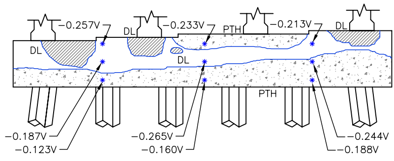
North Elevation
