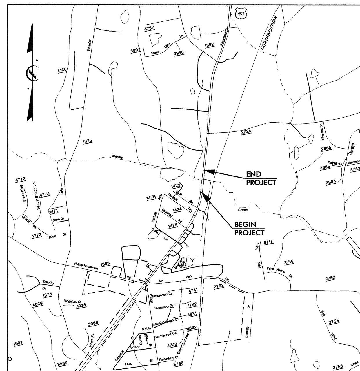
VICINITY MAP
