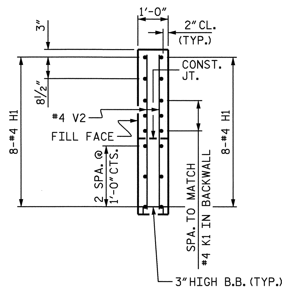
SECTION X-X
