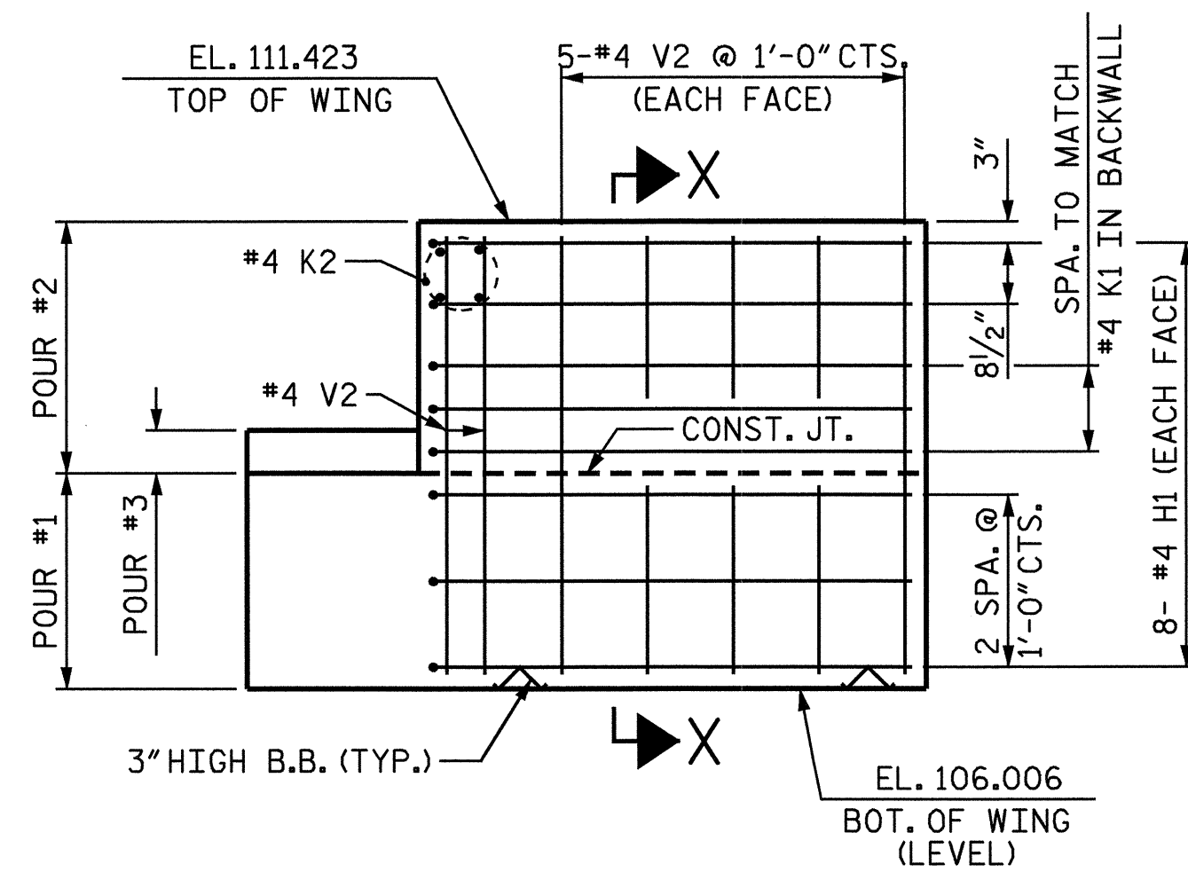
ELEVATION OF LEFT WING (W1)
