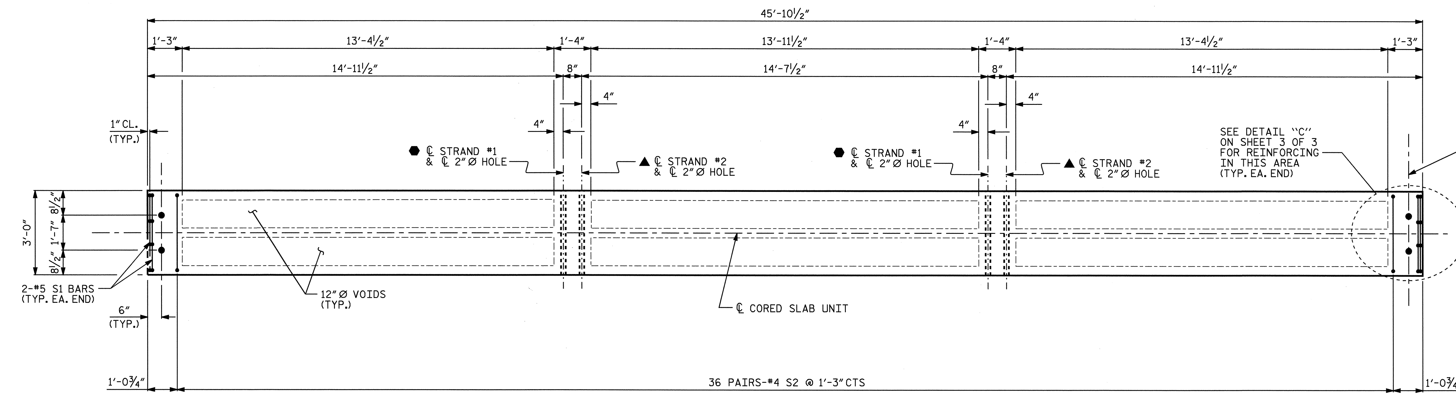
PLAN OF TYPE II CORED SLAB UNIT (STAGE 1)
