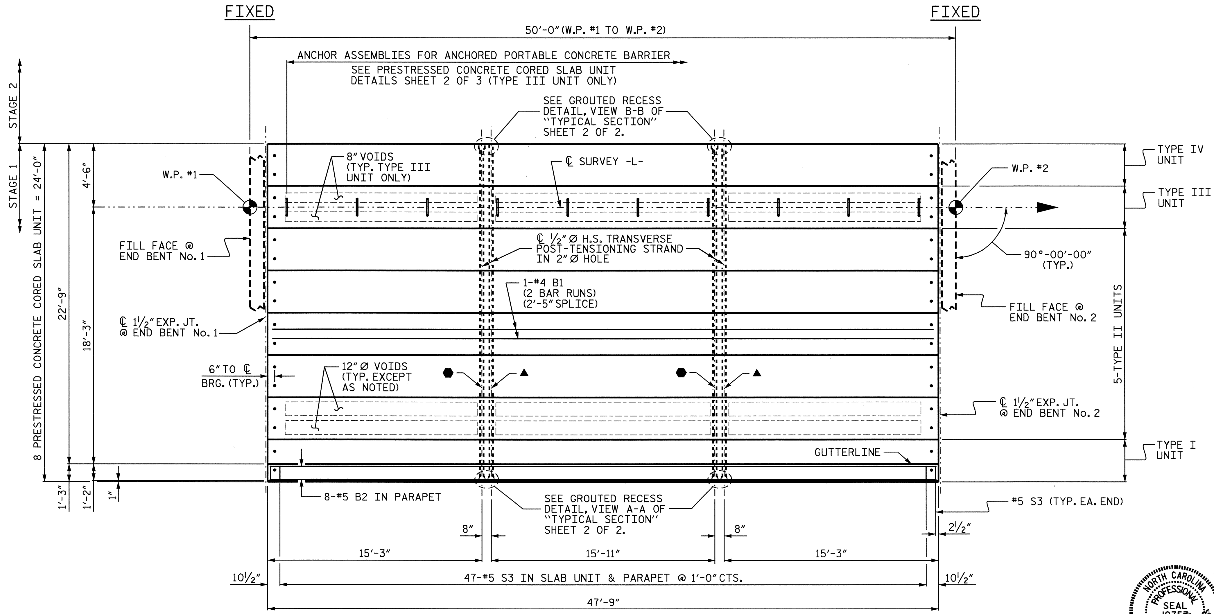
PLAN OF SPAN (STAGE 1)
