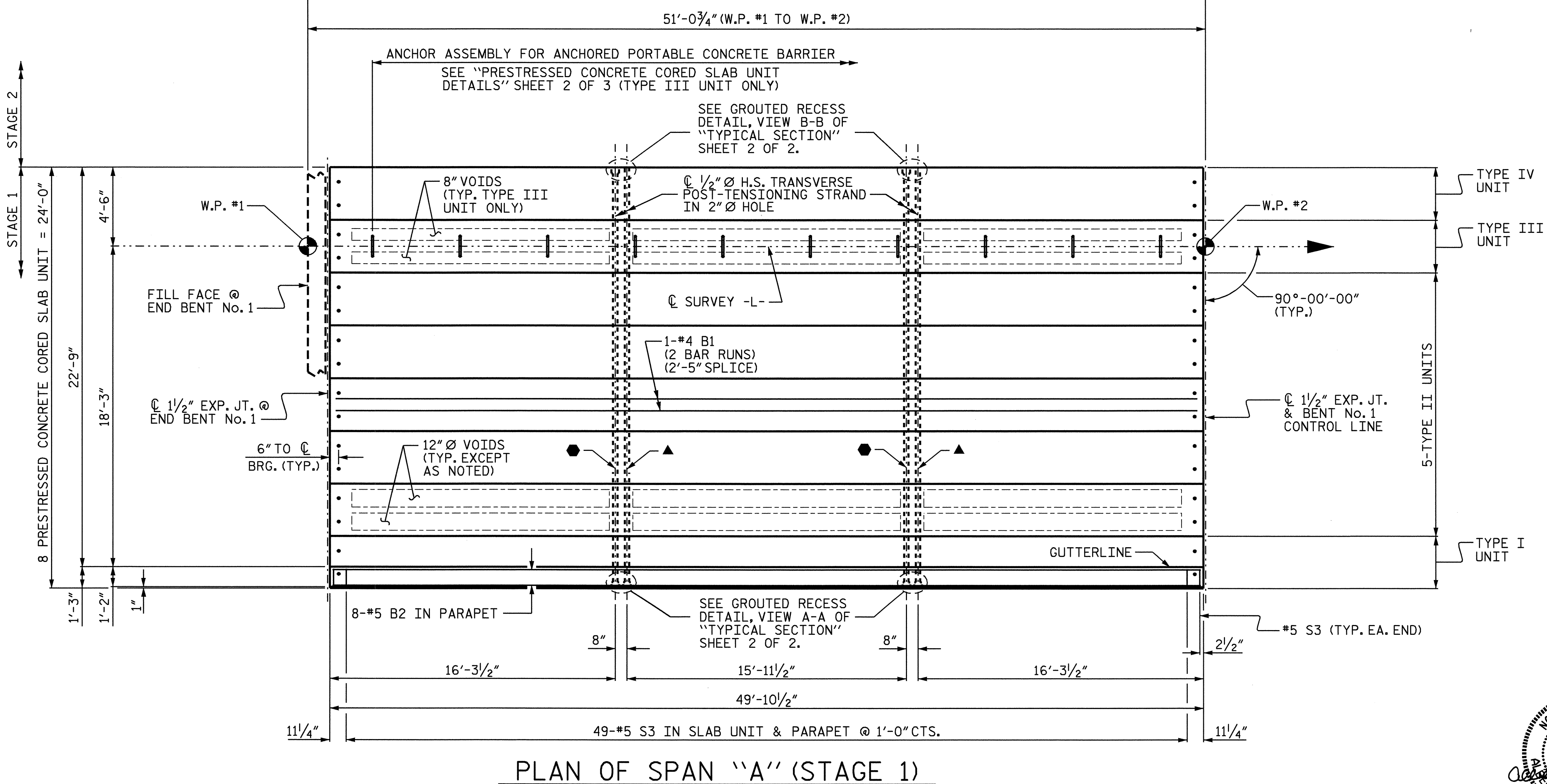
PLAN OF SPAN "A" (STAGE 2)
