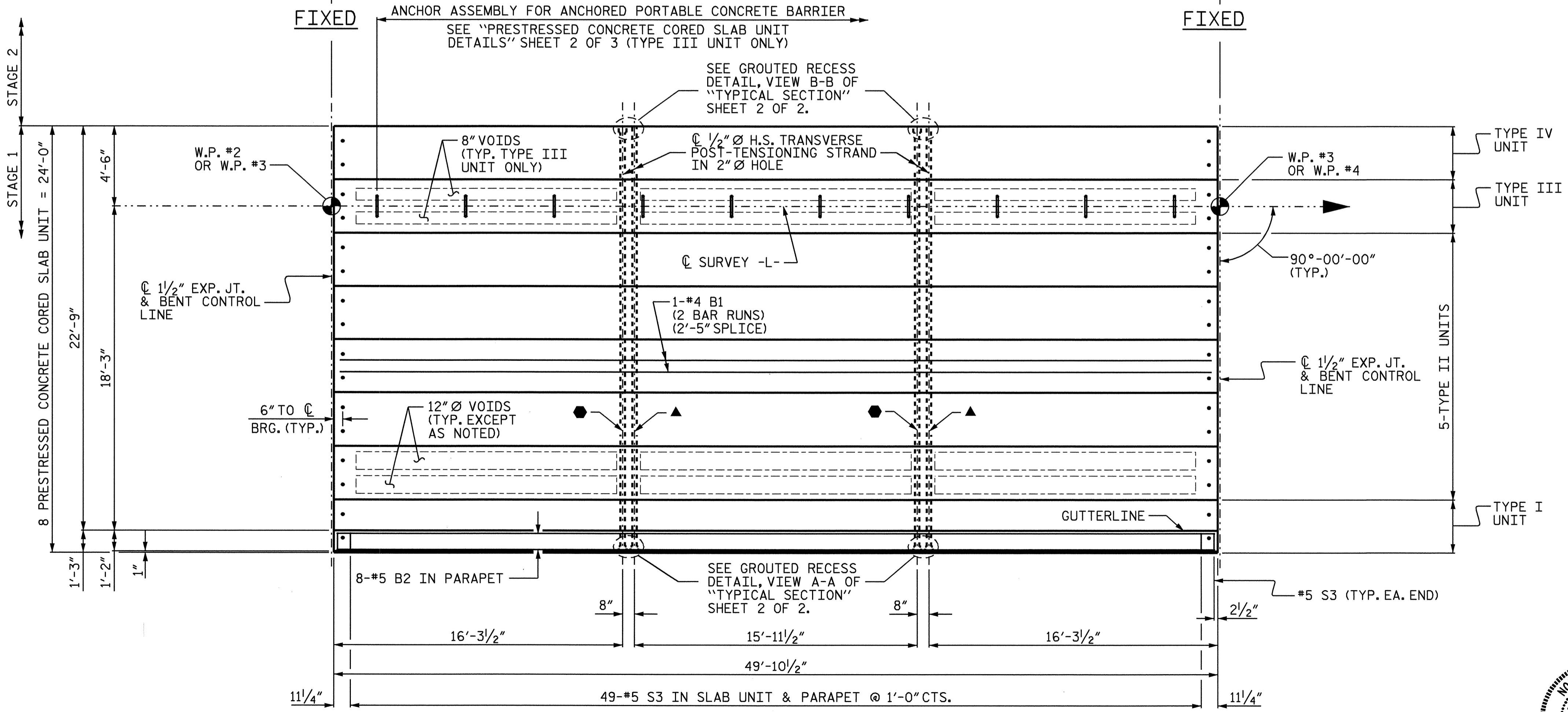
PLAN OF SPAN "B" OR "C" (STAGE 1)
