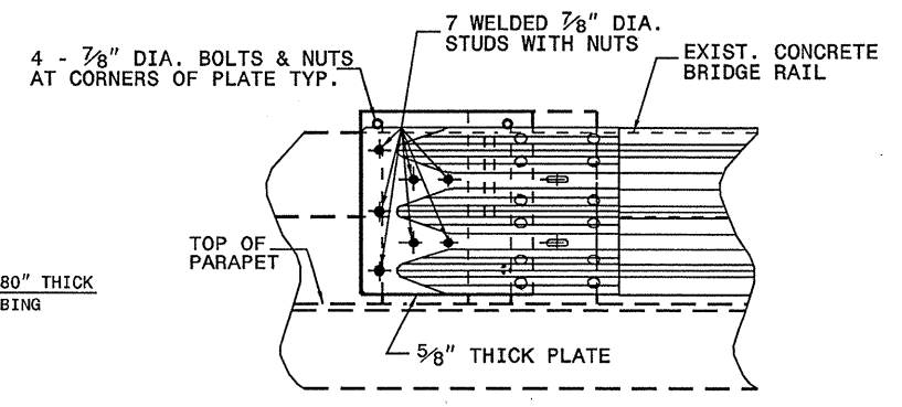
ELEVATION VIEW
