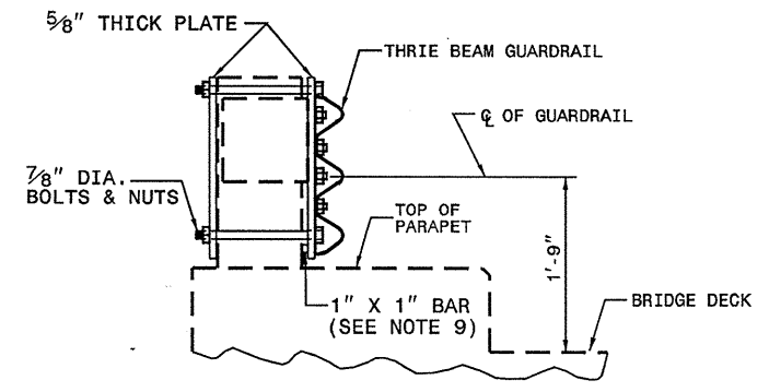
SECTION VIEW
