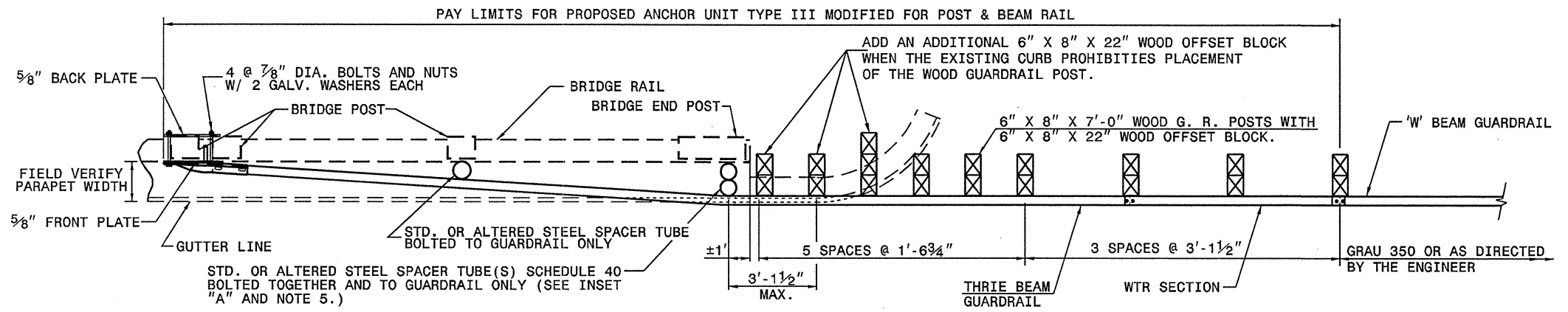
PLAN VIEW
