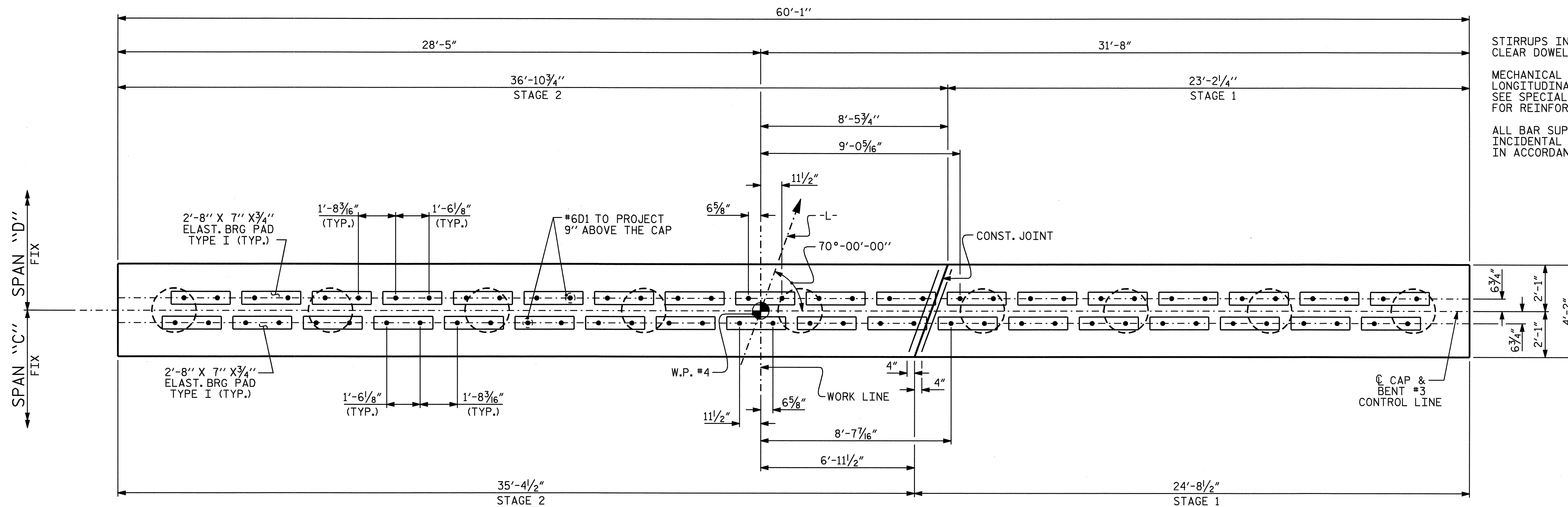
PLAN
