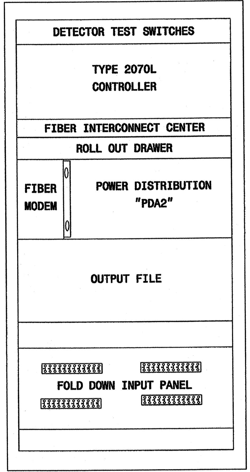
336S CABINET REAR VIEW
