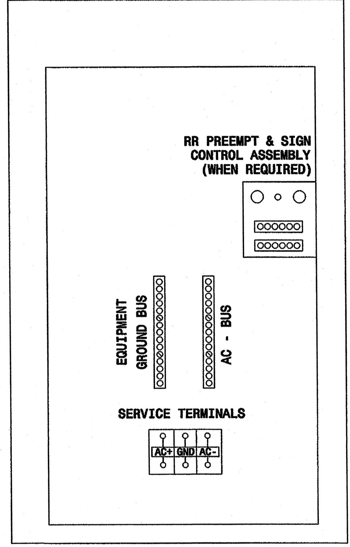
336S CABINET REAR VIEW RIGHT SIDE
