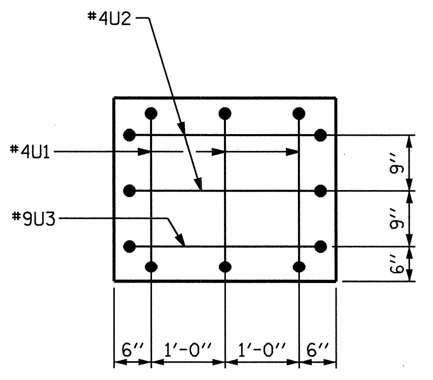
END VIEW
