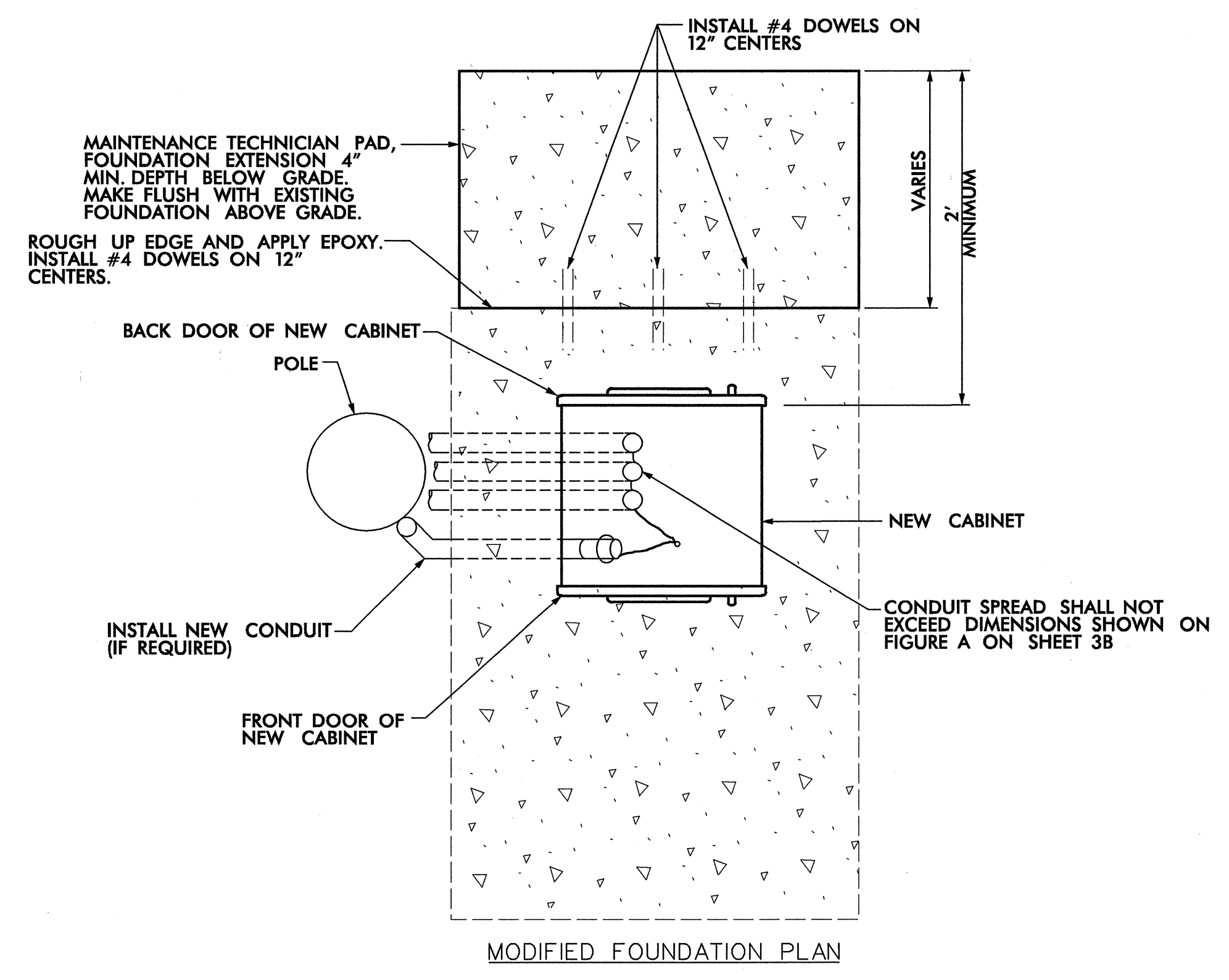
NEW CABINETS ON MODIFIED FOUNDATION WITH SAME ORIENTATION AS EXISTING CABINET
