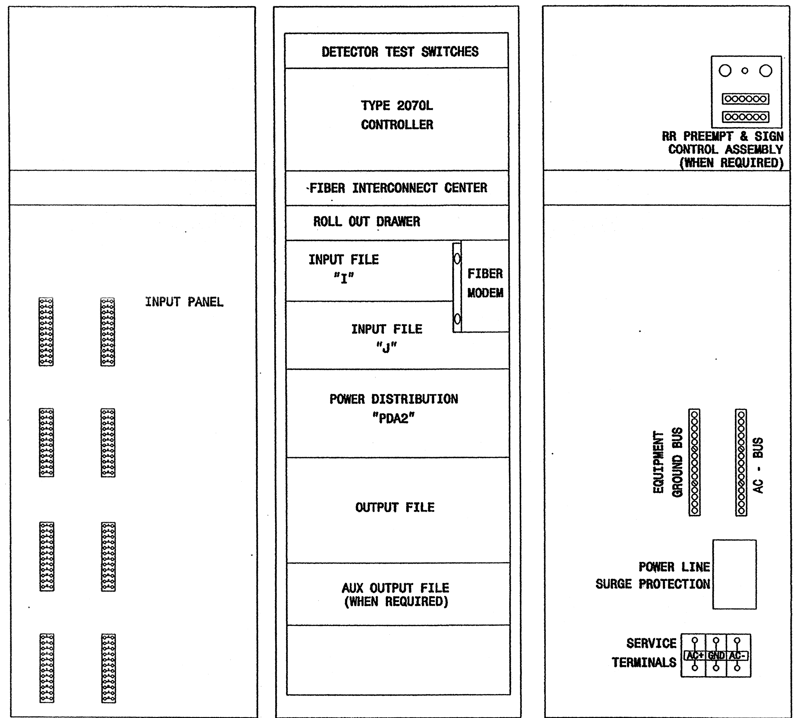
332A CABINET LEFT SIDE
