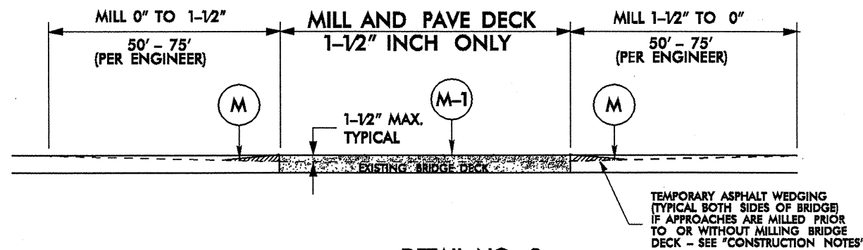
DETAIL NO. 2 MAP NO. 1, BRIDGE NO. 8 SEE CHART BELOW FOR EXISTING BRIDGE RESURFACING INSTRUCTIONS
