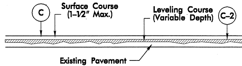
DETAIL NO. 1 LEVELING DETAIL MAP NO. 3, SR 1210, BROWN MTN. RD. (AT LOCATIONS DESIGNATED BY ENGINEER)
