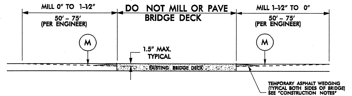
DETAIL NO. 3 MAP NO. 1, BRIDGE NO. 22 SEE CHART BELOW FOR EXISTING BRIDGE PAVING INSTRUCTIONS
