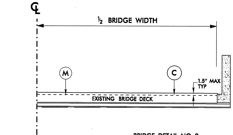
BRIDGE DETAIL NO. 2 BRIDGE NO. 301, MAP NO 7, SR 2312 EXISTING BRIDGE DECK: STEEL PLANK WITH 3" ASPHALT WEARING SURFACE BRIDGE POSTED - SV 33, TTST 38
