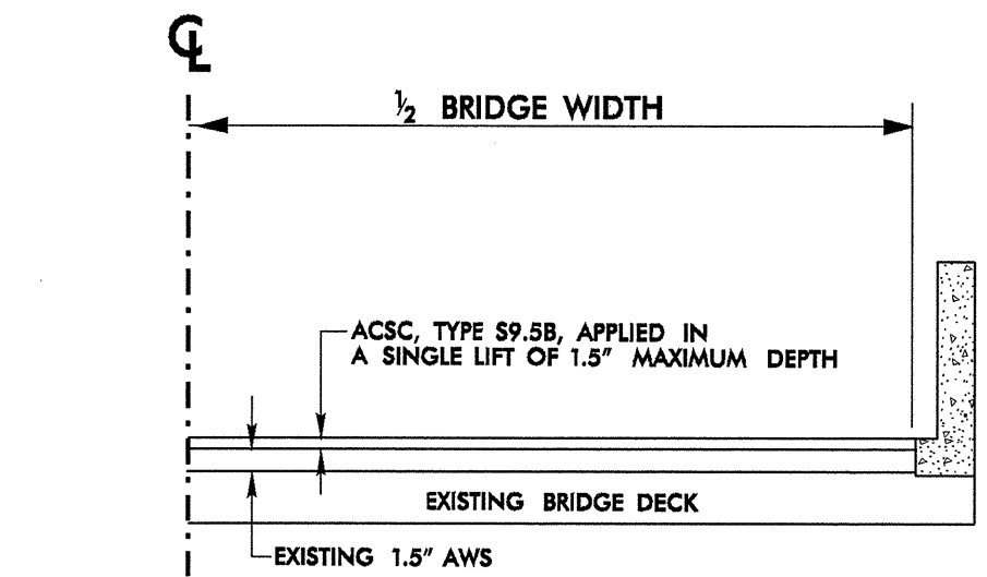
BRIDGE DETAIL NO. 1 BRIDGE NO. 210, MAP NO 3, SR 1506 EXISTING BRIDGE DECK: 4x8 TIMBERS WITH 1.5" ASPHALT WEARING SURFACE BRIDGE POSTED - SV 18, TTST 23
